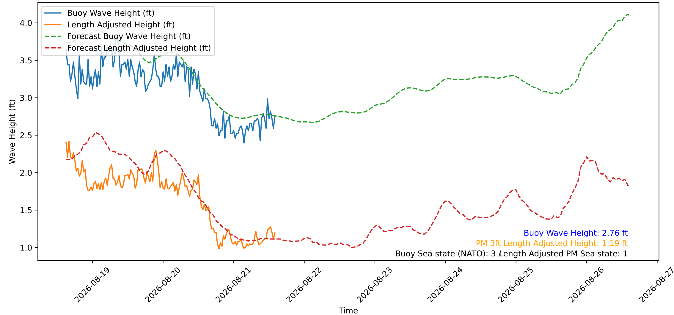
Wave Heights over Time for Oceanside Harbor at 2026-08-21 15:00:27
