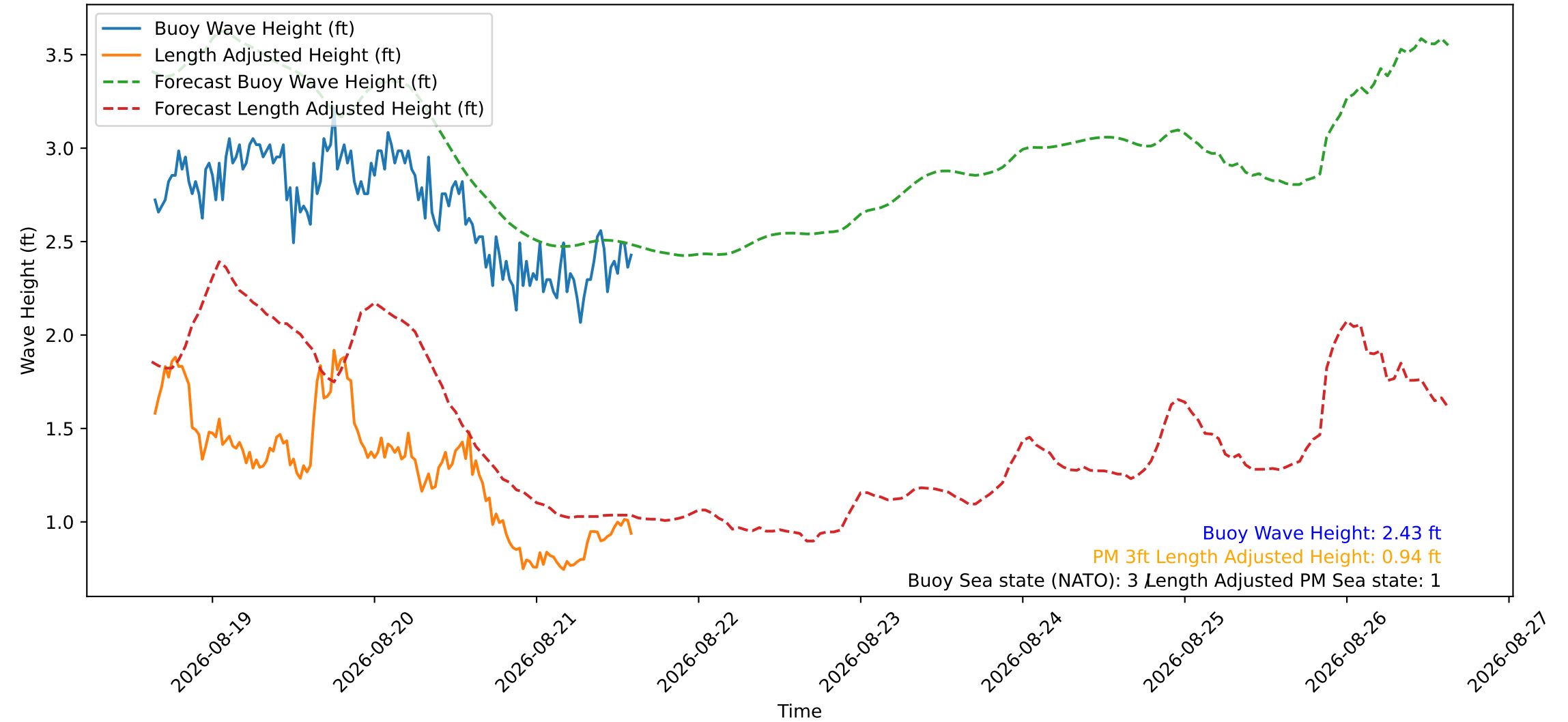
Wave Heights over Time for Red Beach at 2026-08-21 15:00:47
