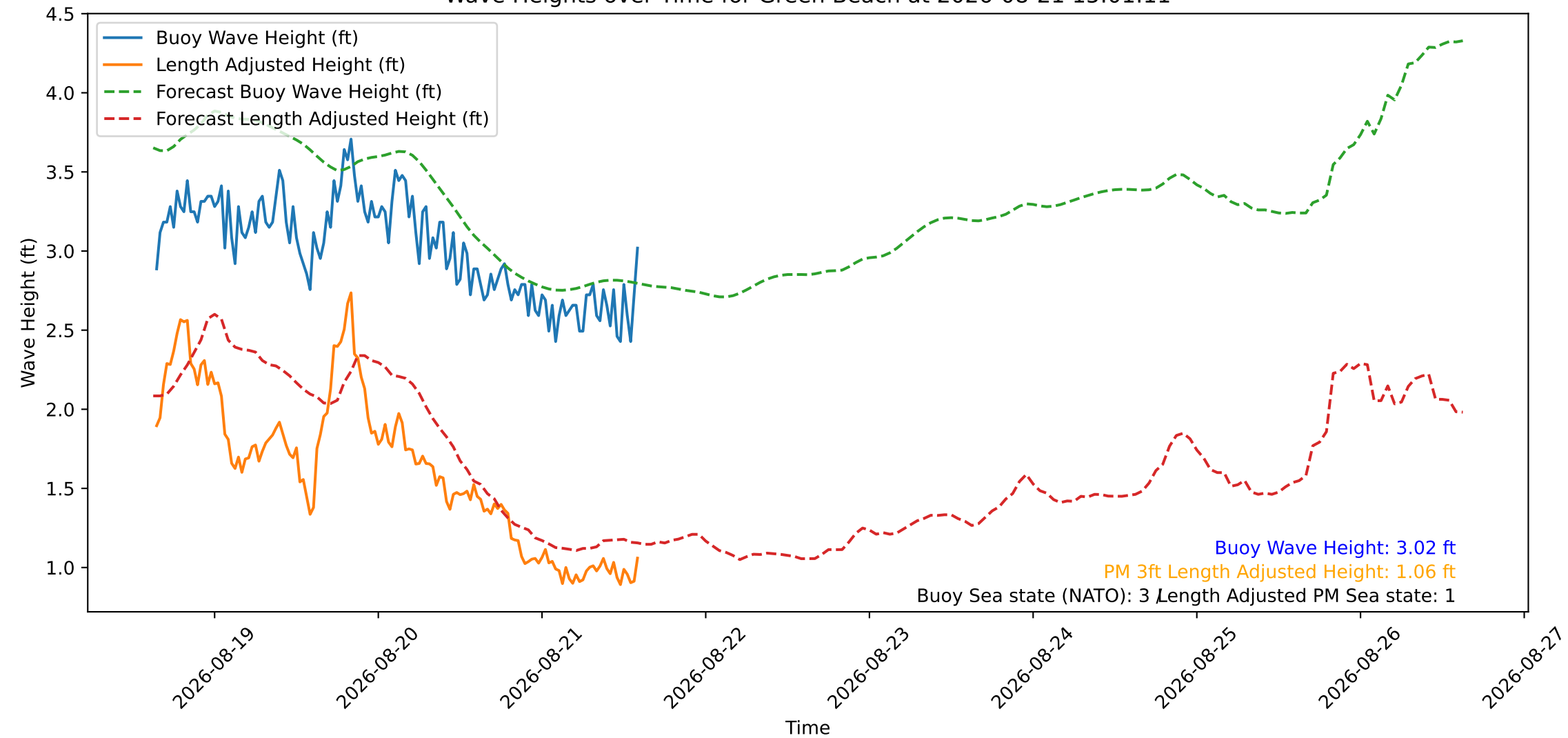
Wave Heights over Time for Green Beach at 2026-08-21 15:01:11
