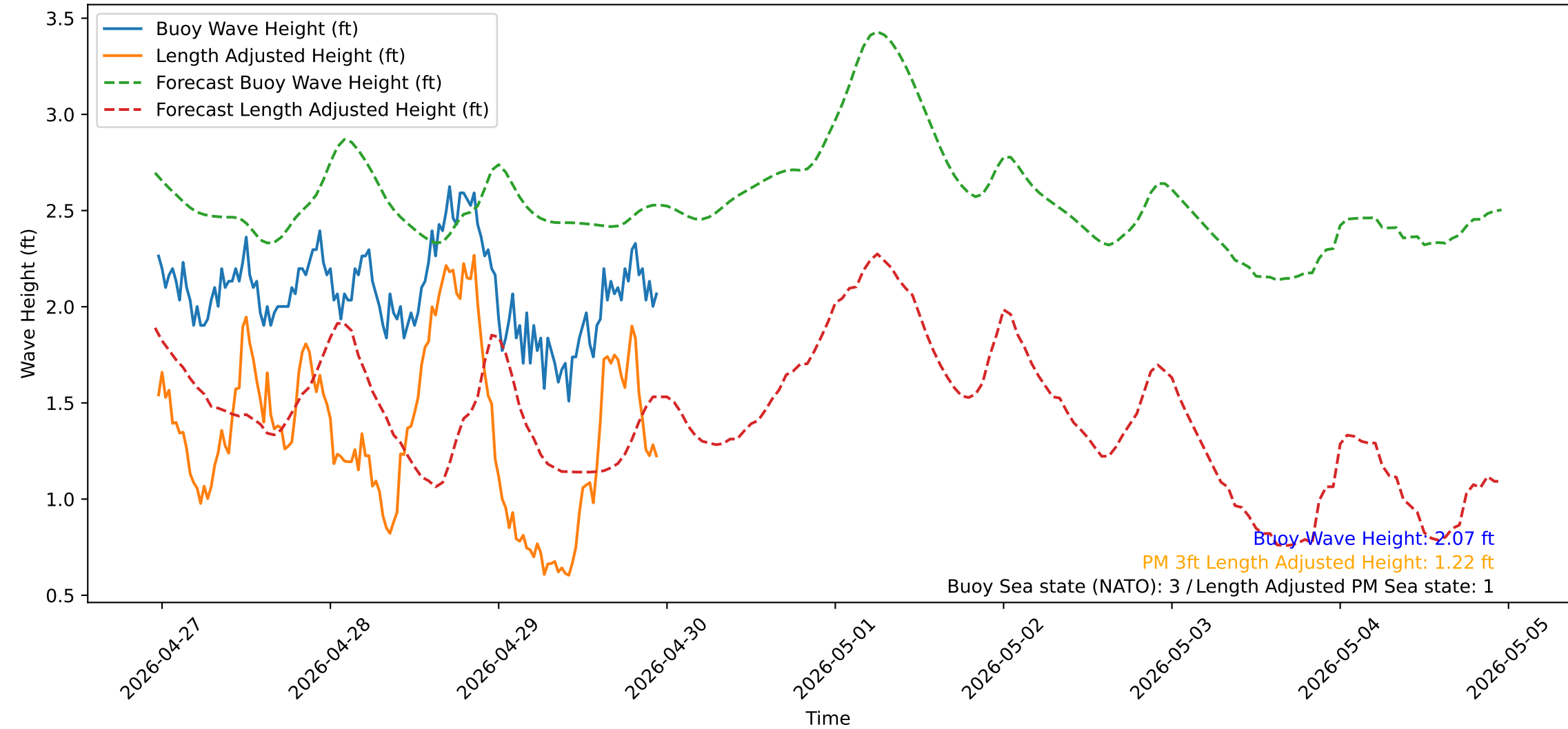
Wave Heights over Time for Red Beach at 2026-04-29 23:20:51
