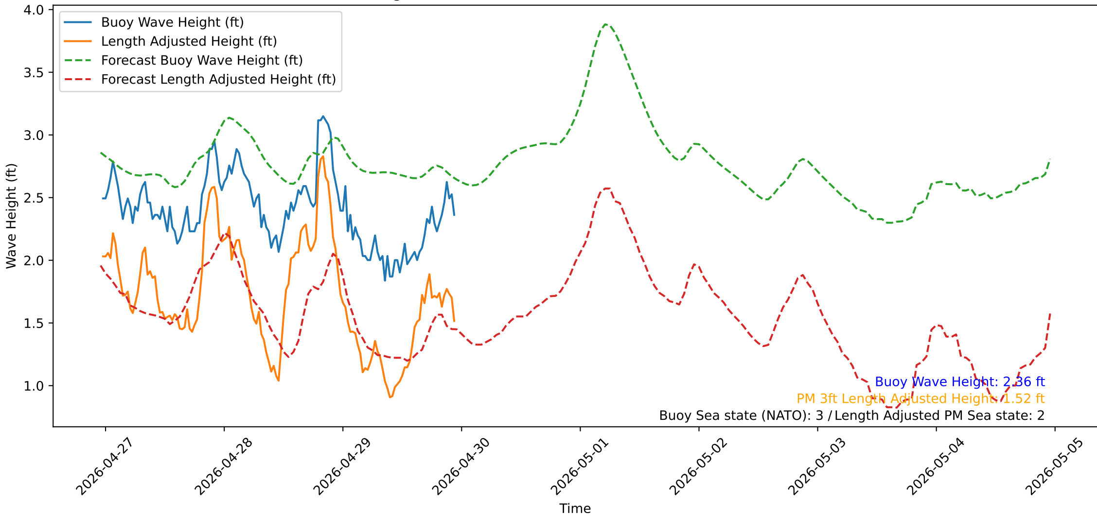
Wave Heights over Time for Green Beach at 2026-04-29 23:21:13
