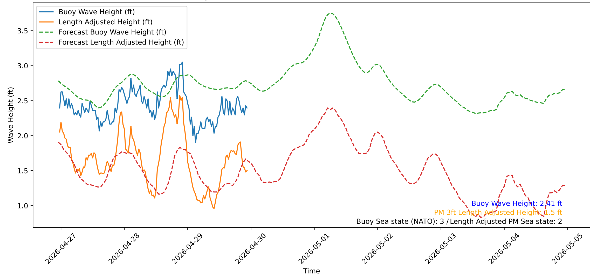
Wave Heights over Time for Oceanside Harbor at 2026-04-29 23:20:30
