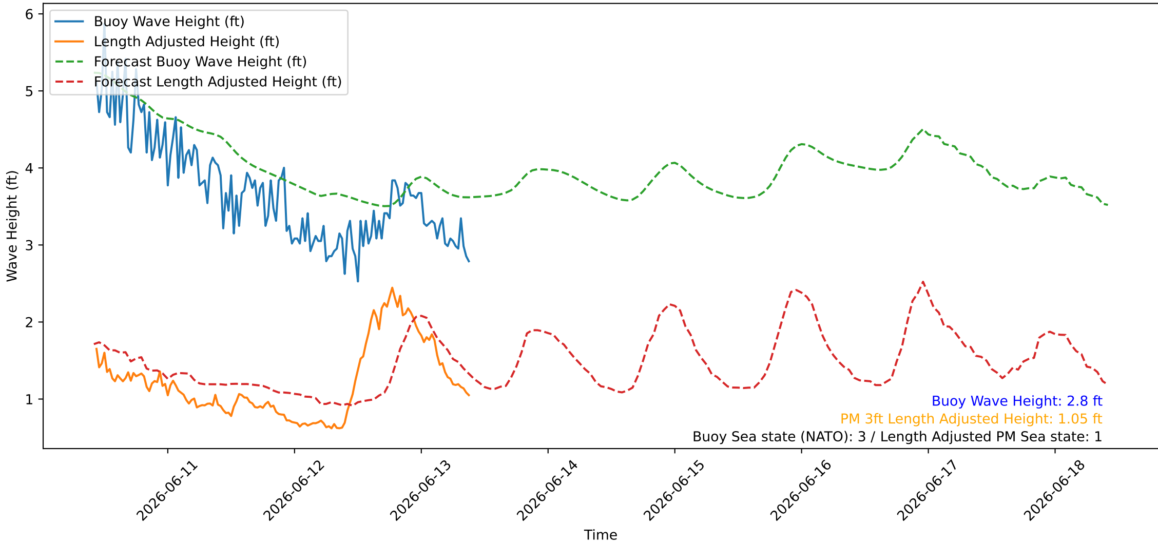
Wave Heights over Time for Red Beach at 2026-06-13 10:00:45
