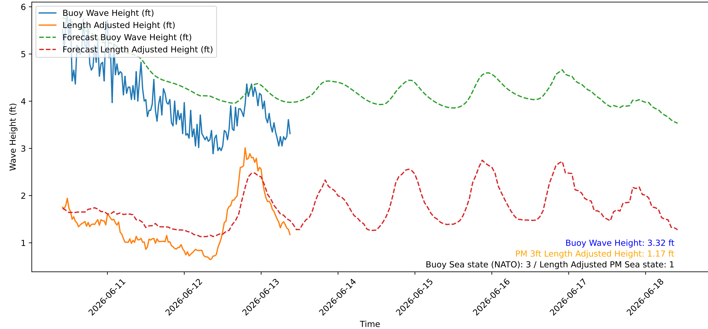
Wave Heights over Time for Green Beach at 2026-06-13 10:01:08
