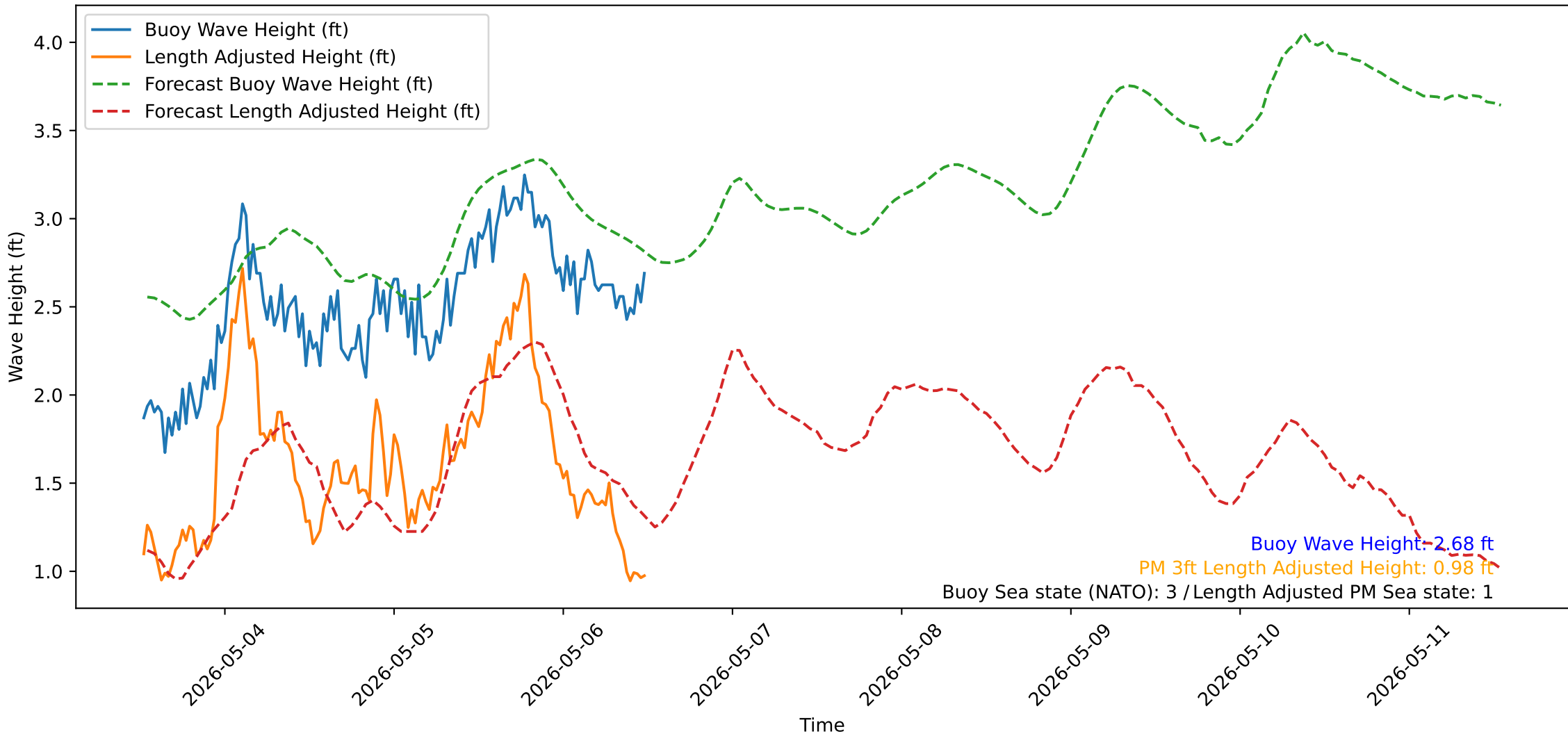
Wave Heights over Time for Oceanside Harbor at 2026-05-06 12:30:31
