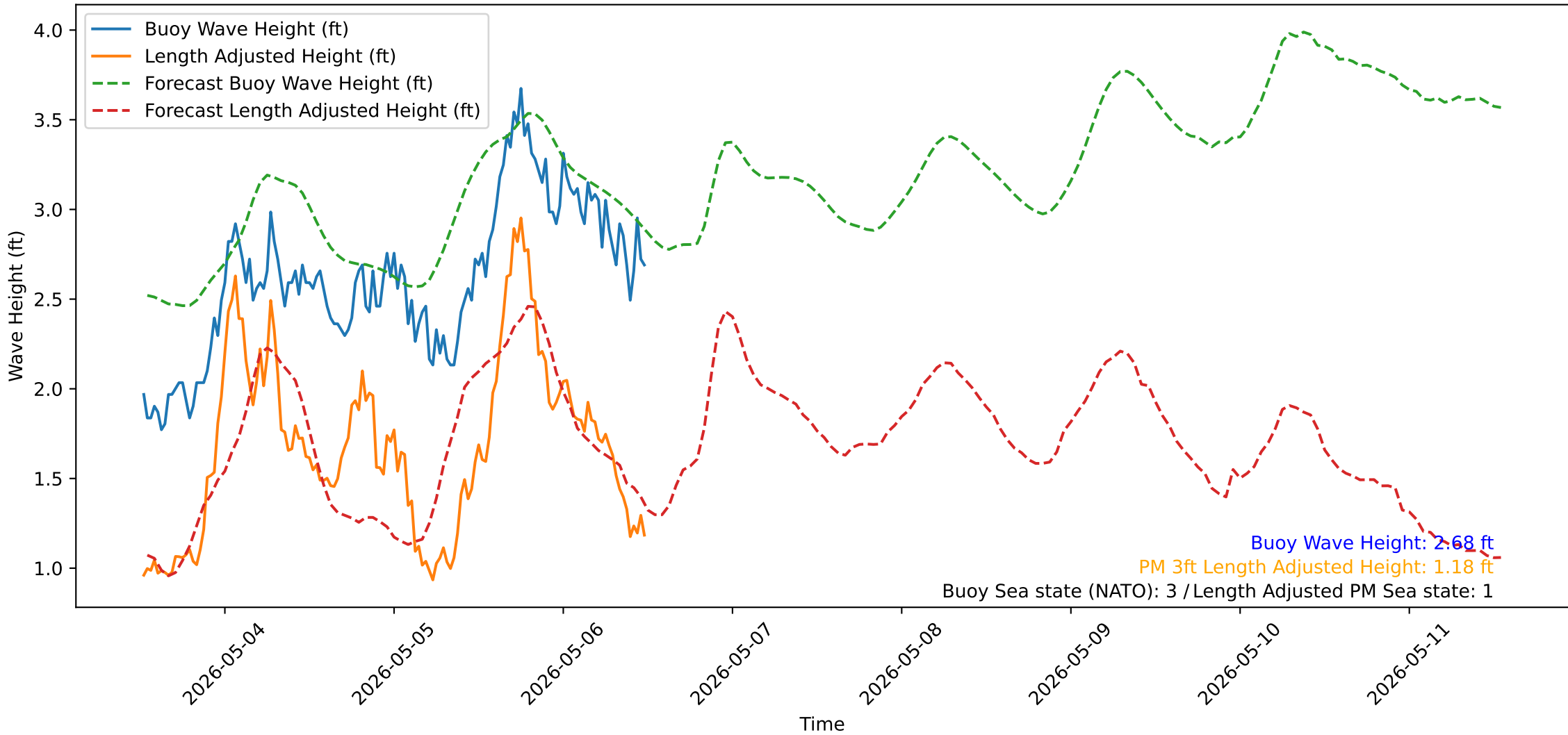
Wave Heights over Time for Green Beach at 2026-05-06 12:31:12
