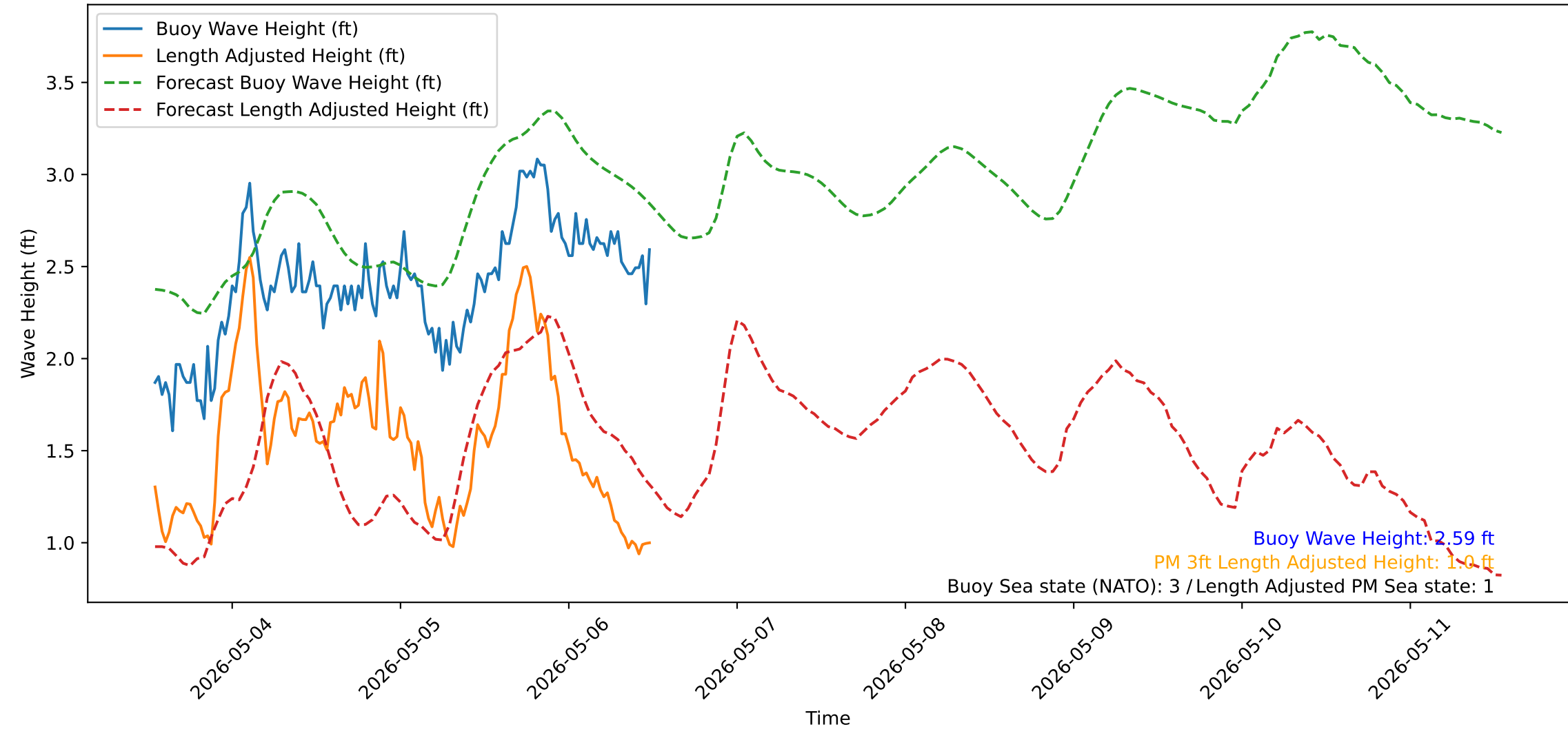
Wave Heights over Time for Red Beach at 2026-05-06 12:30:50
