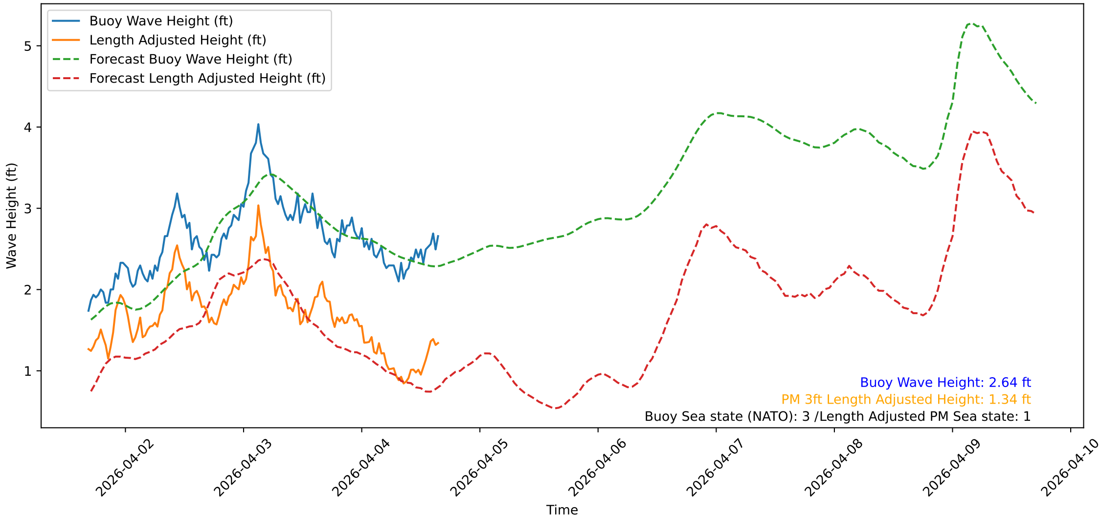
Wave Heights over Time for Oceanside Harbor at 2026-04-04 16:40:33
