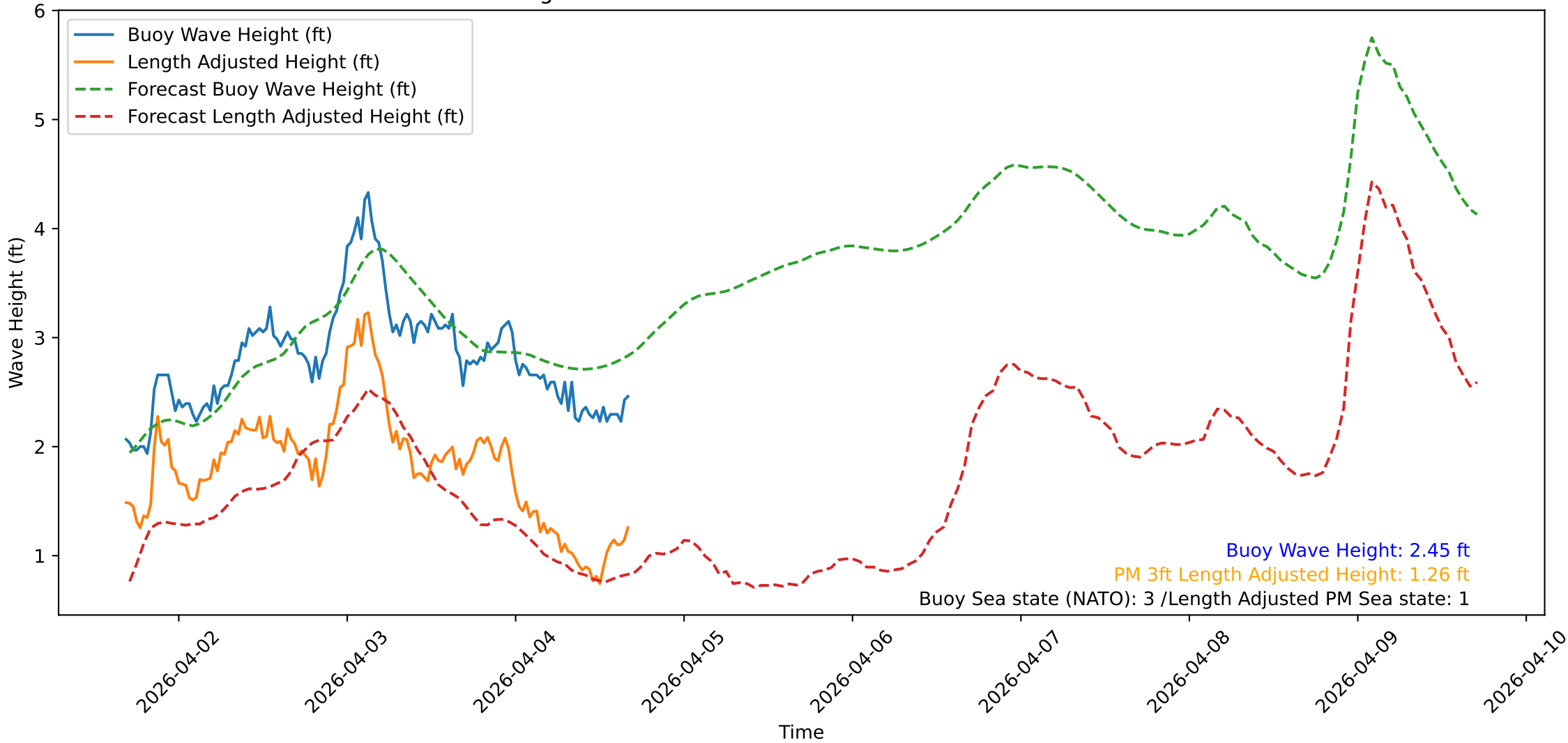
Wave Heights over Time for Green Beach at 2026-04-04 16:41:13
