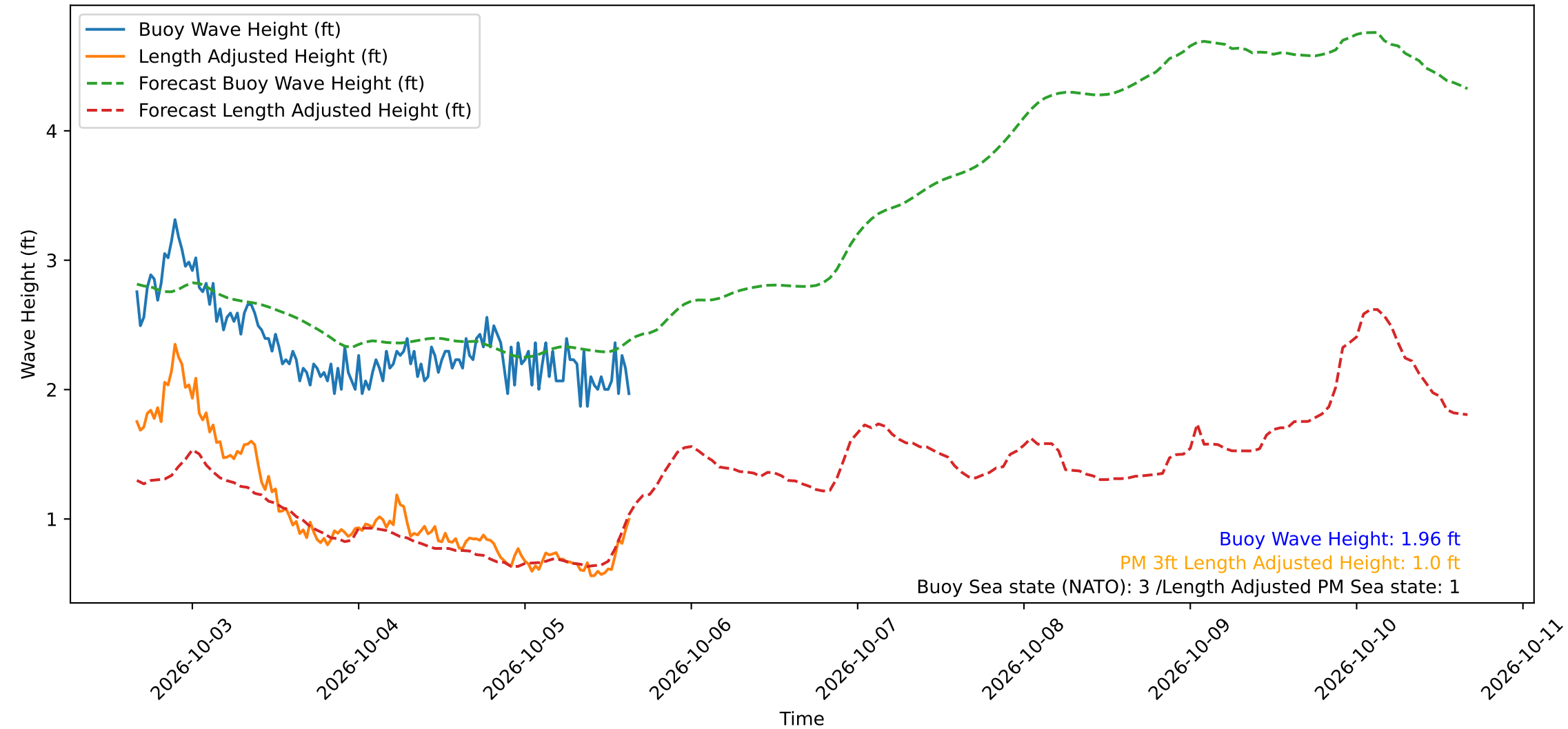
Wave Heights over Time for Oceanside Harbor at 2026-10-05 16:00:29
