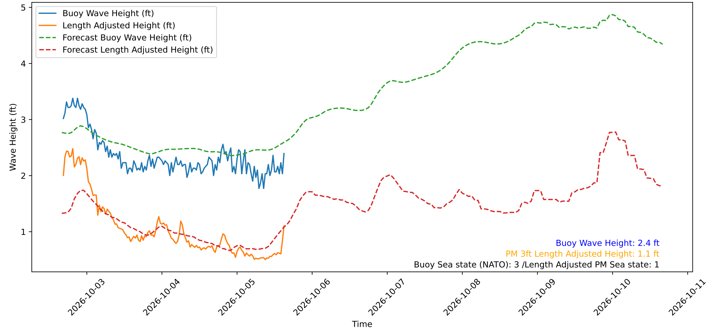
Wave Heights over Time for Green Beach at 2026-10-05 16:01:11
