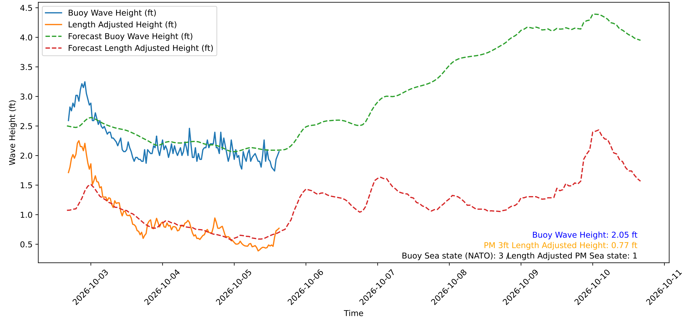
Wave Heights over Time for Red Beach at 2026-10-05 16:00:49
