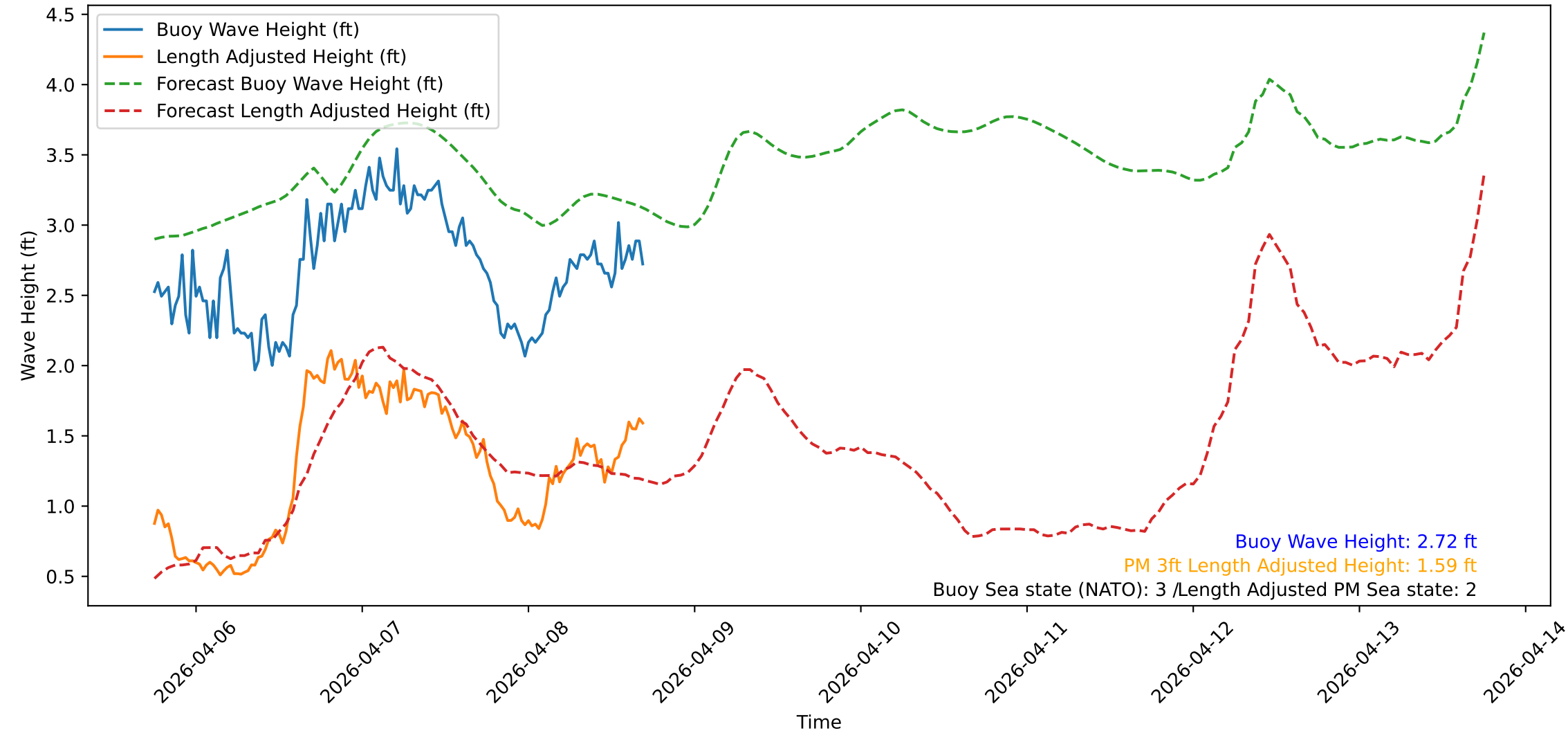
Wave Heights over Time for Red Beach at 2026-04-08 17:30:48
