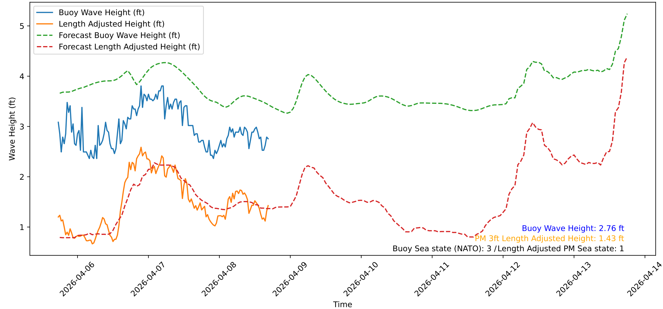
Wave Heights over Time for Green Beach at 2026-04-08 17:31:10
