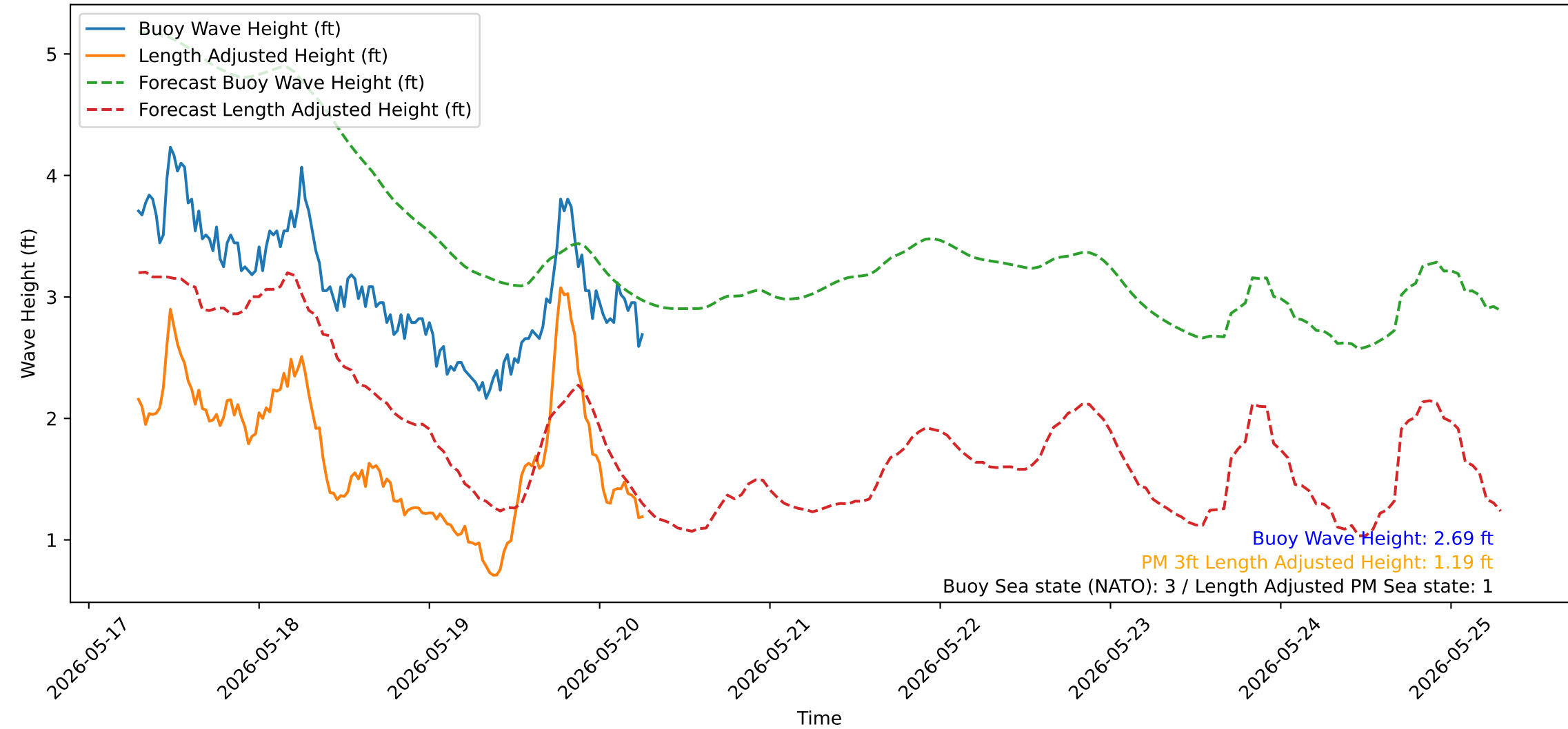
Wave Heights over Time for Green Beach at 2026-05-20 06:51:15
