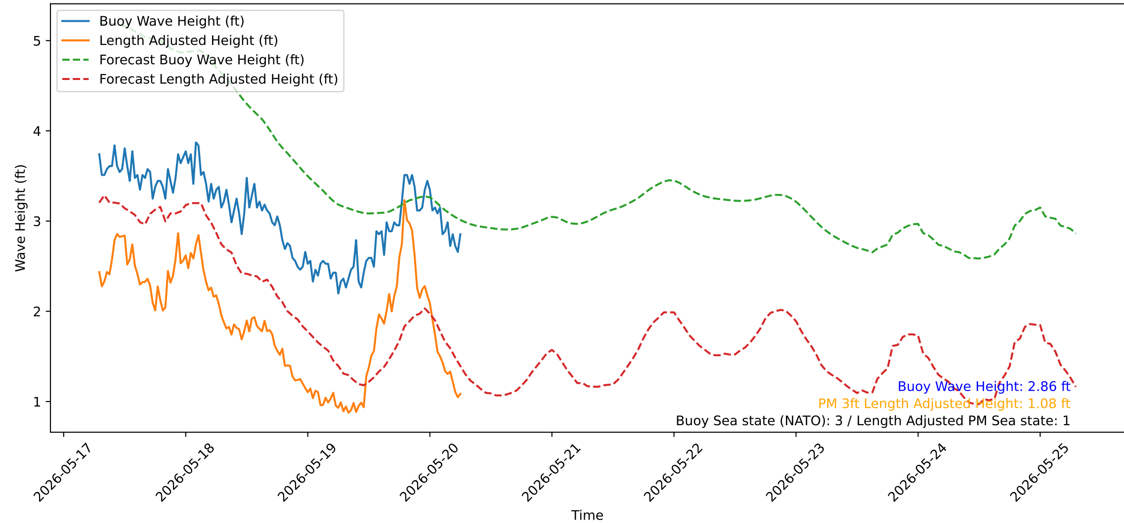
Wave Heights over Time for Oceanside Harbor at 2026-05-20 06:50:31
