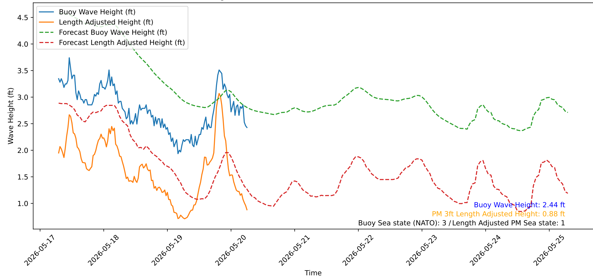
Wave Heights over Time for Red Beach at 2026-05-20 06:50:52
