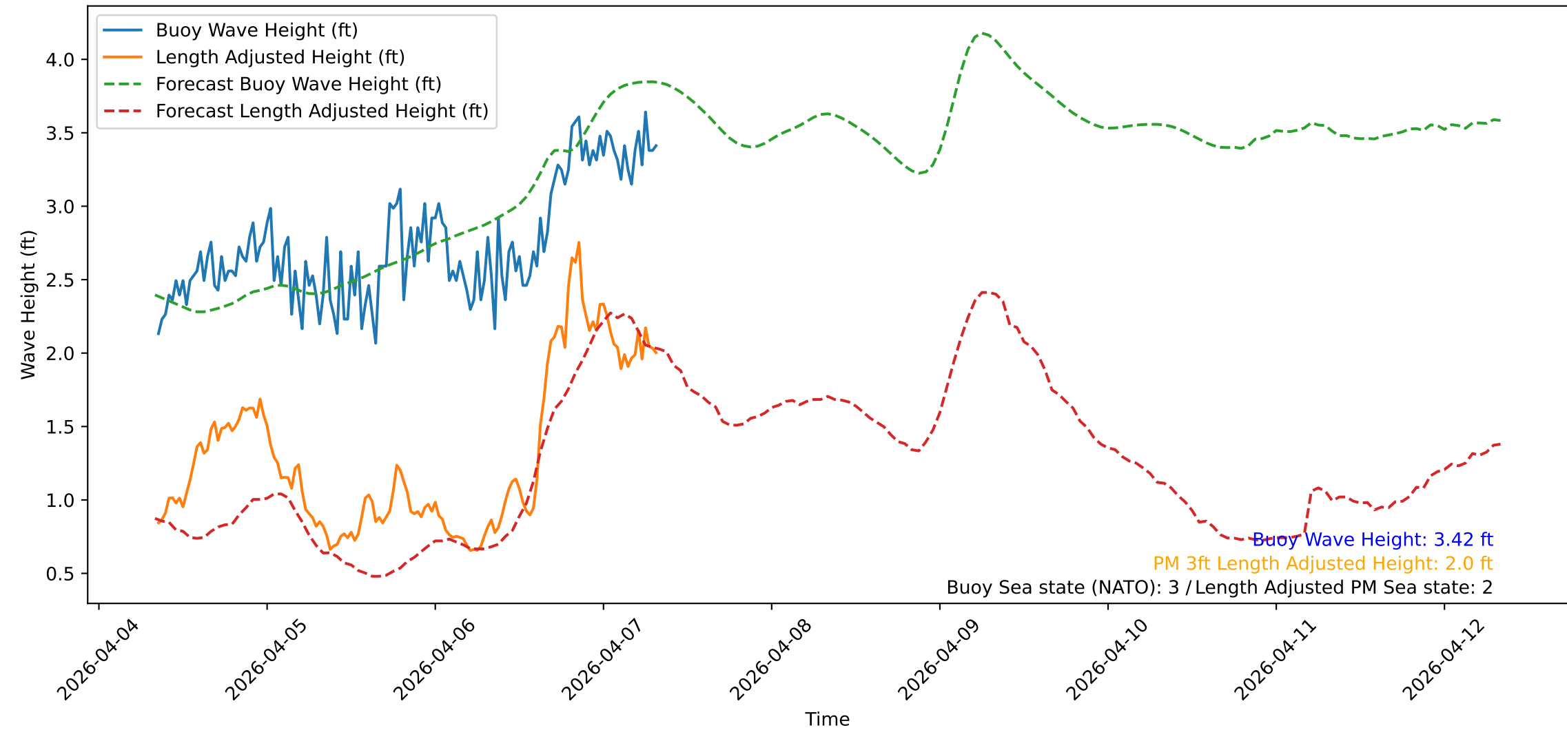
Wave Heights over Time for Oceanside Harbor at 2026-04-07 08:20:32
