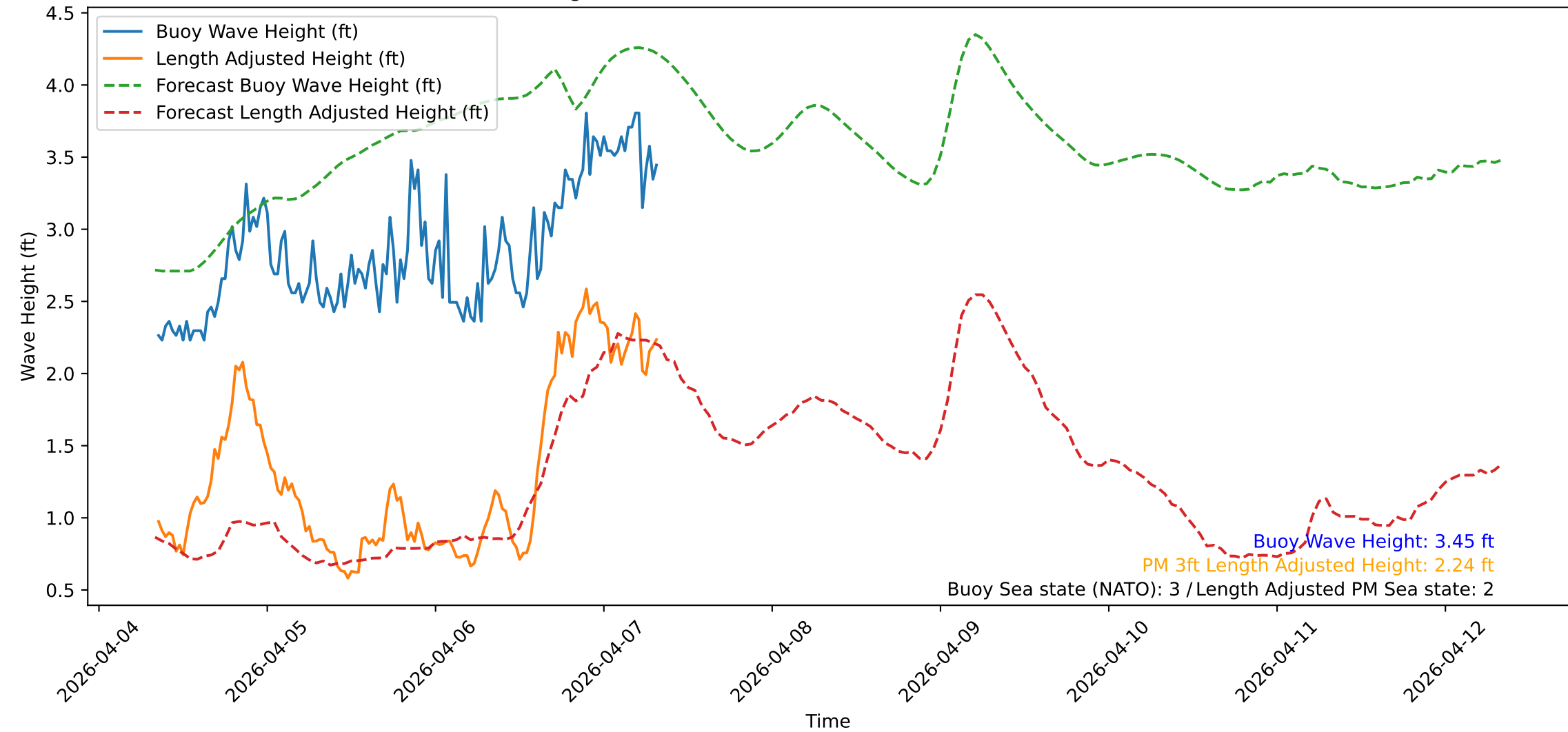
Wave Heights over Time for Green Beach at 2026-04-07 08:21:11
