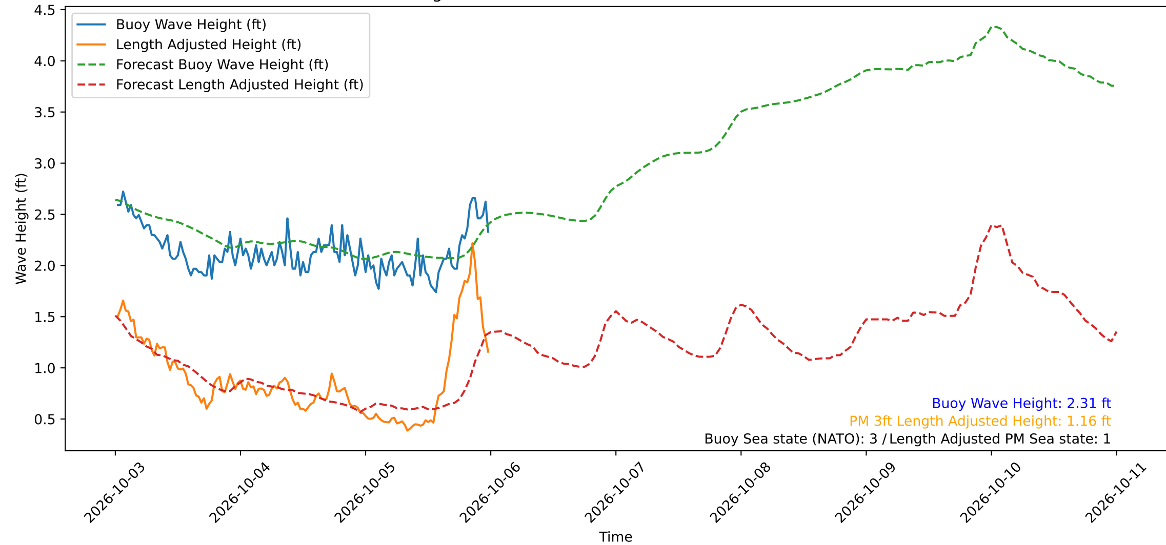
Wave Heights over Time for Red Beach at 2026-10-06 00:10:50
