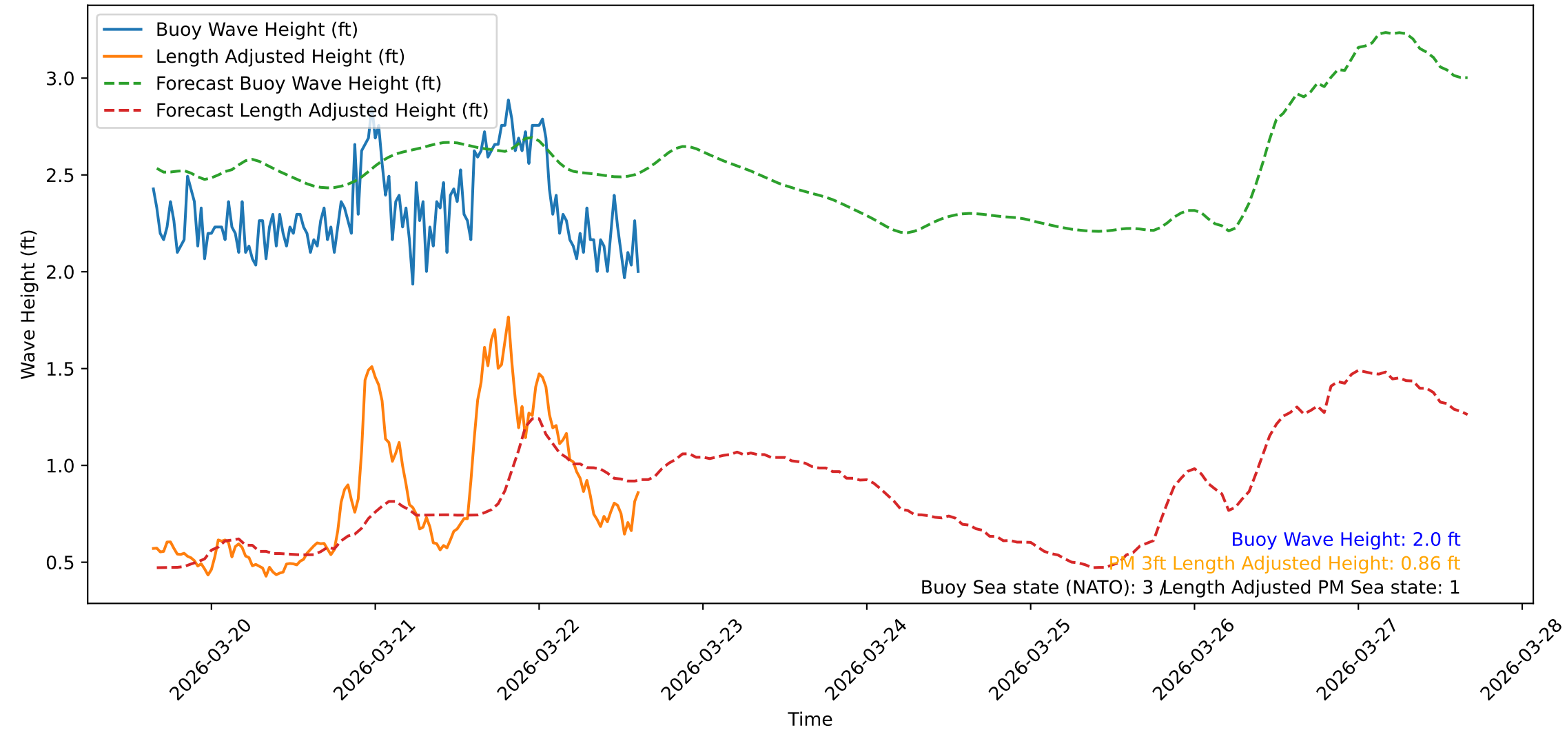
Wave Heights over Time for Green Beach at 2026-03-22 15:31:09
