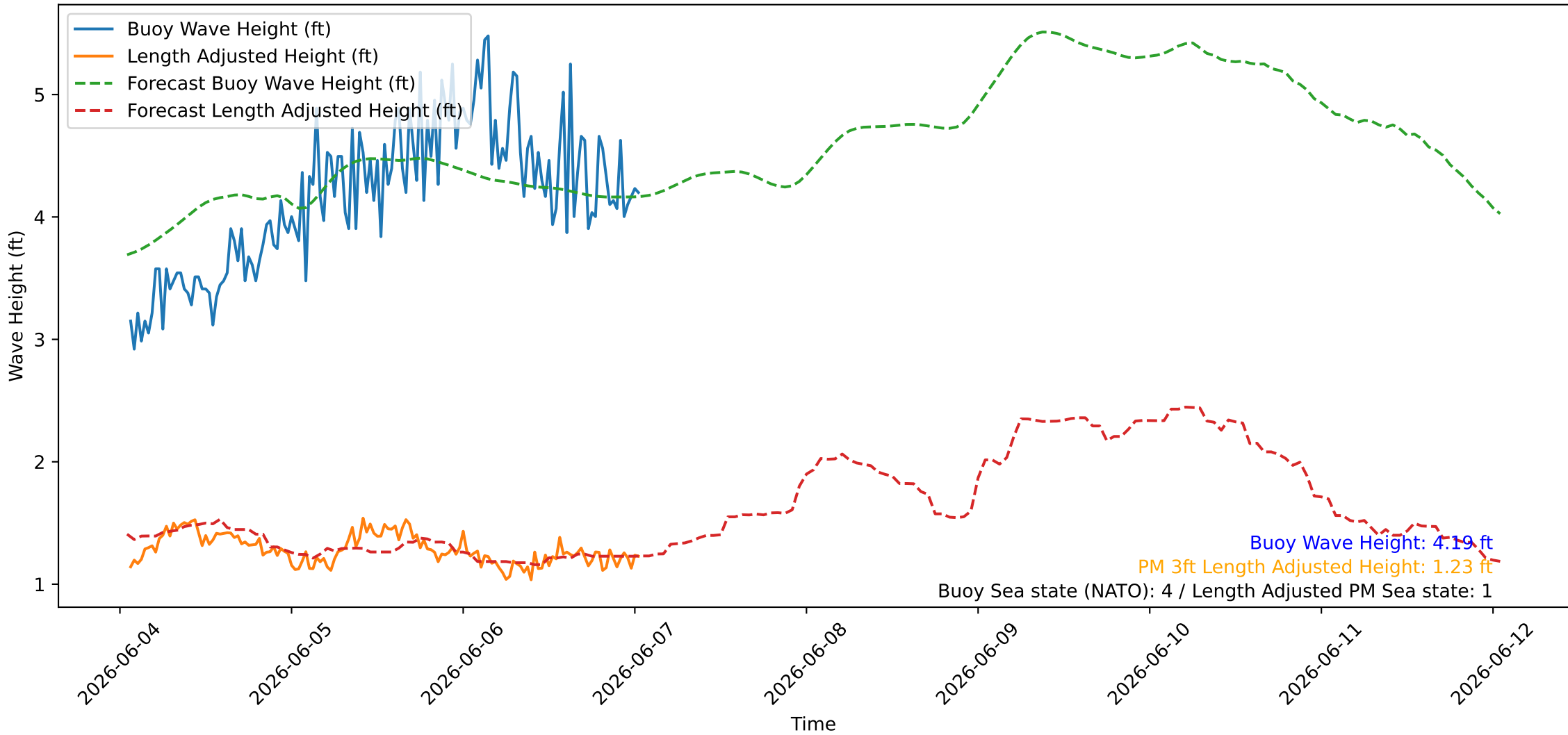
Wave Heights over Time for Oceanside Harbor at 2026-06-07 01:20:26
