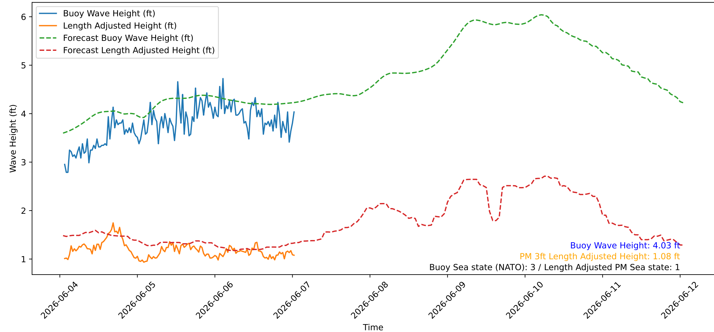
Wave Heights over Time for Green Beach at 2026-06-07 01:21:09
