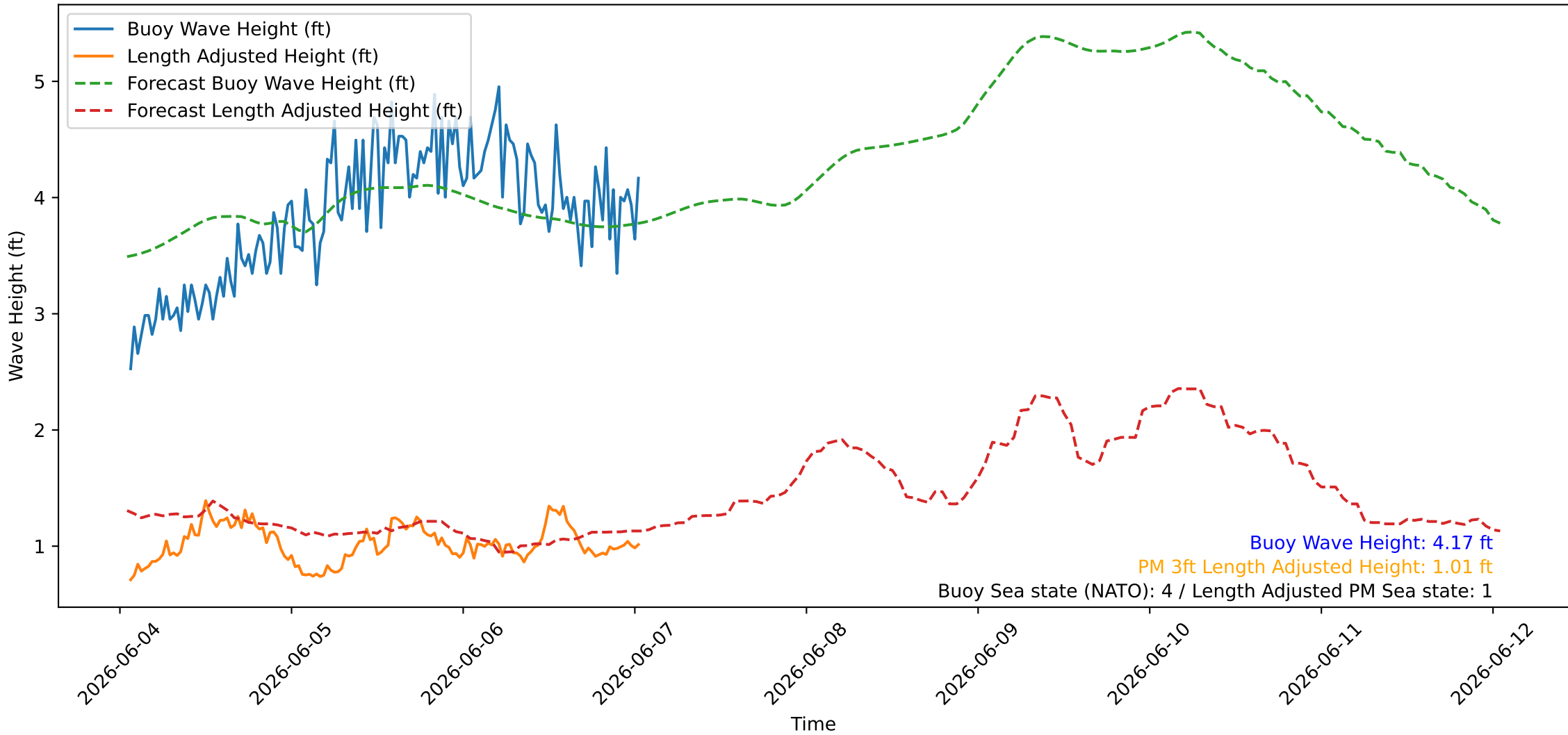
Wave Heights over Time for Red Beach at 2026-06-07 01:20:46
