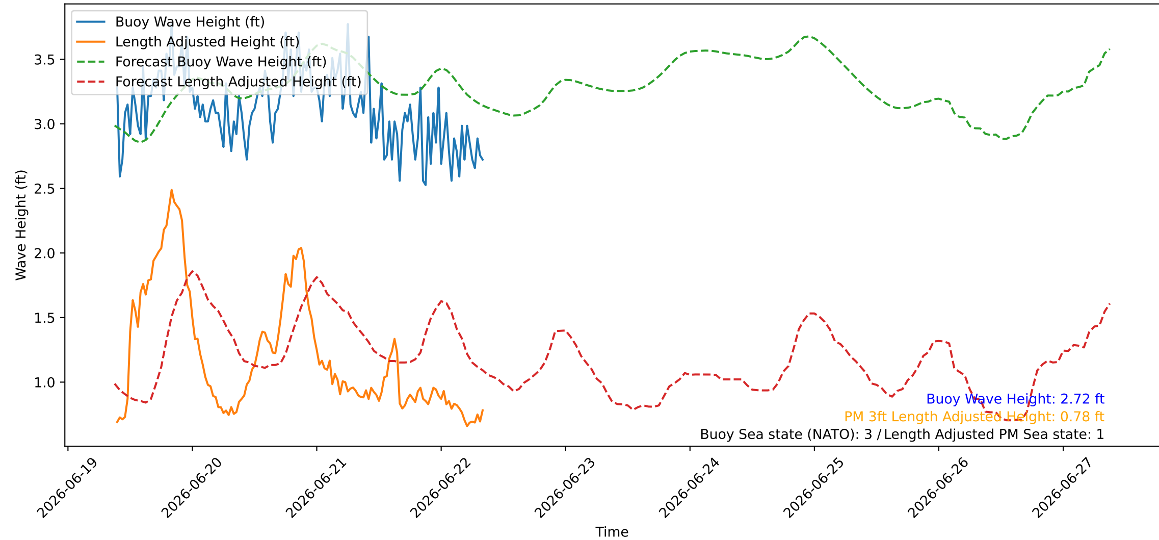
Wave Heights over Time for Red Beach at 2026-06-22 09:00:47
