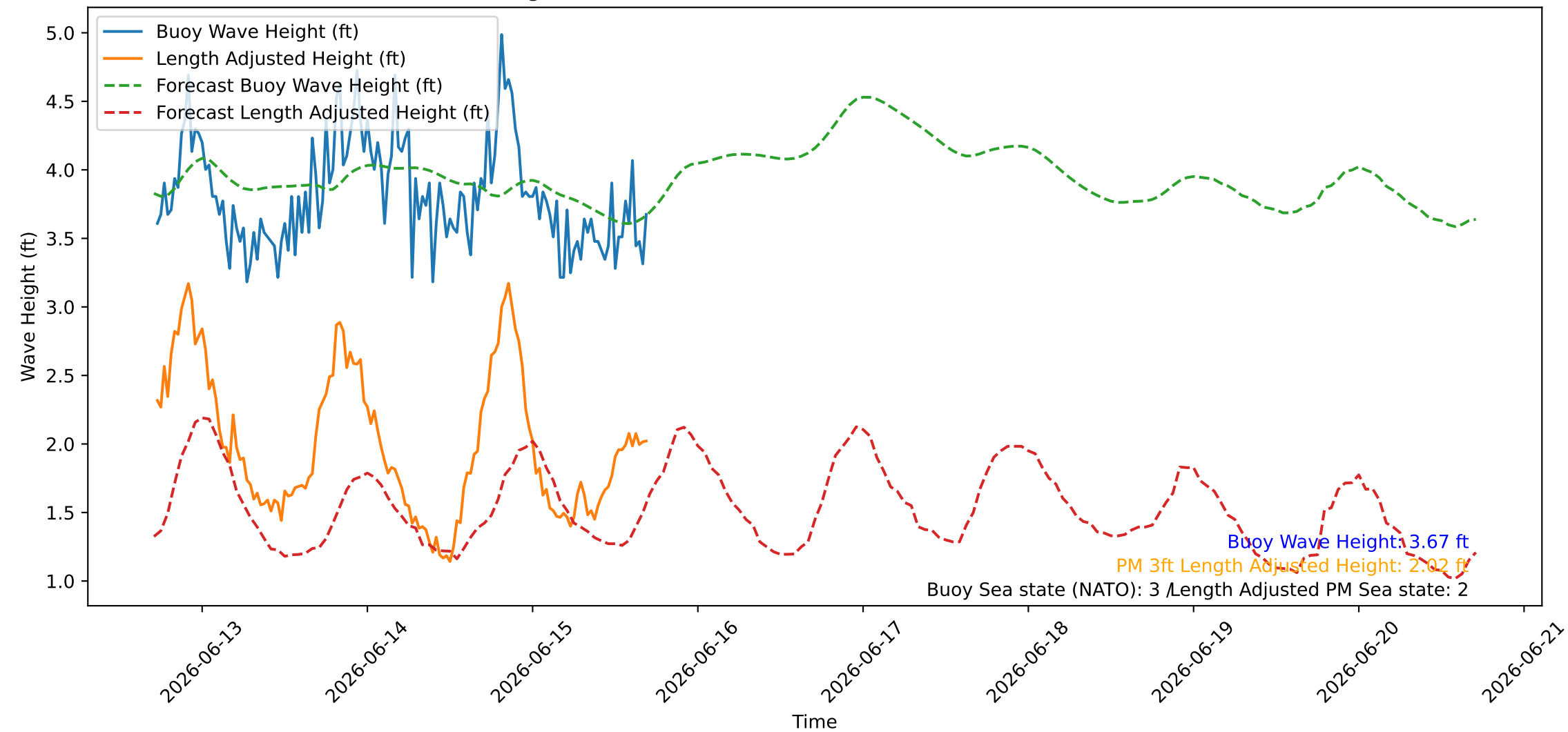
Wave Heights over Time for Oceanside Harbor at 2026-06-15 17:20:26
