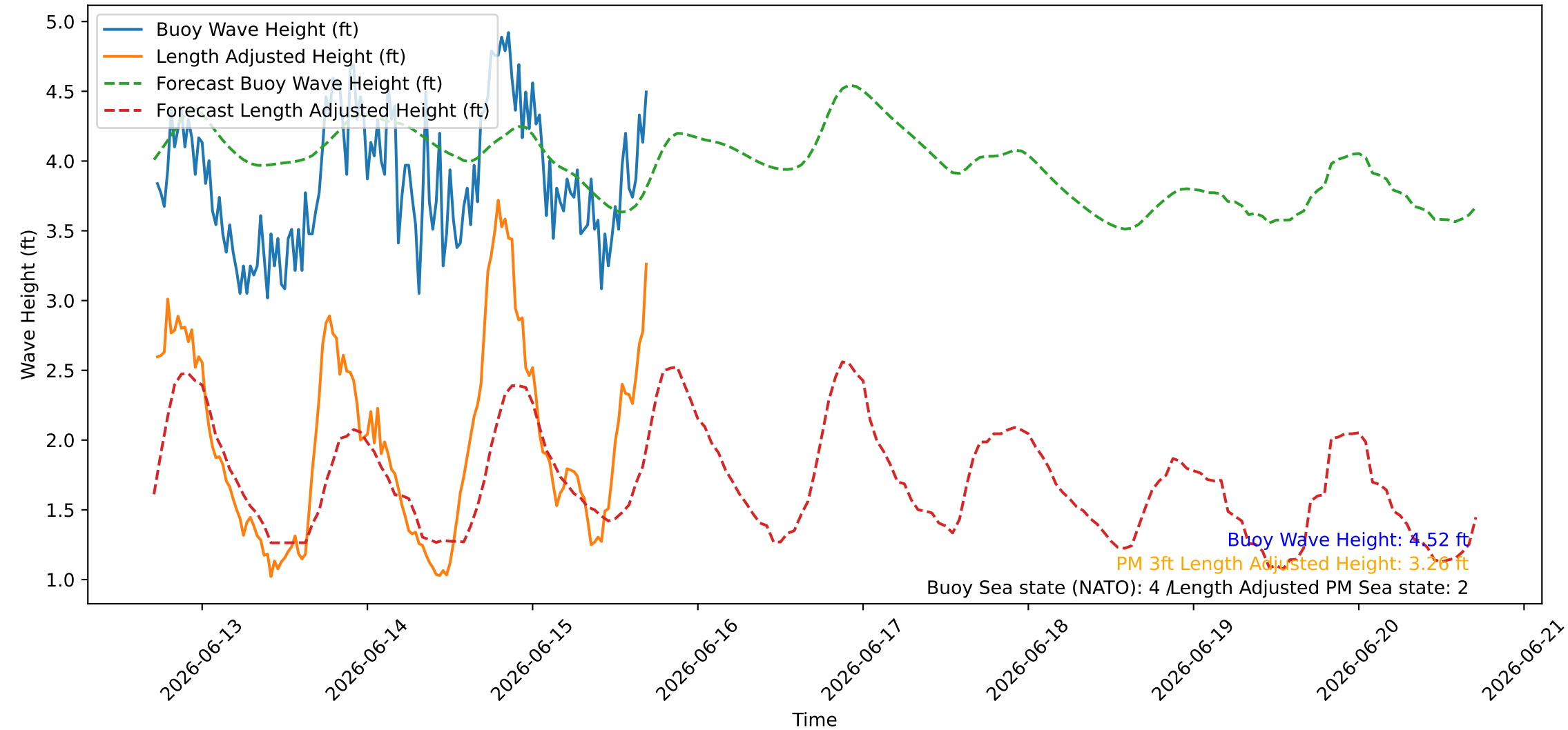
Wave Heights over Time for Green Beach at 2026-06-15 17:21:09
