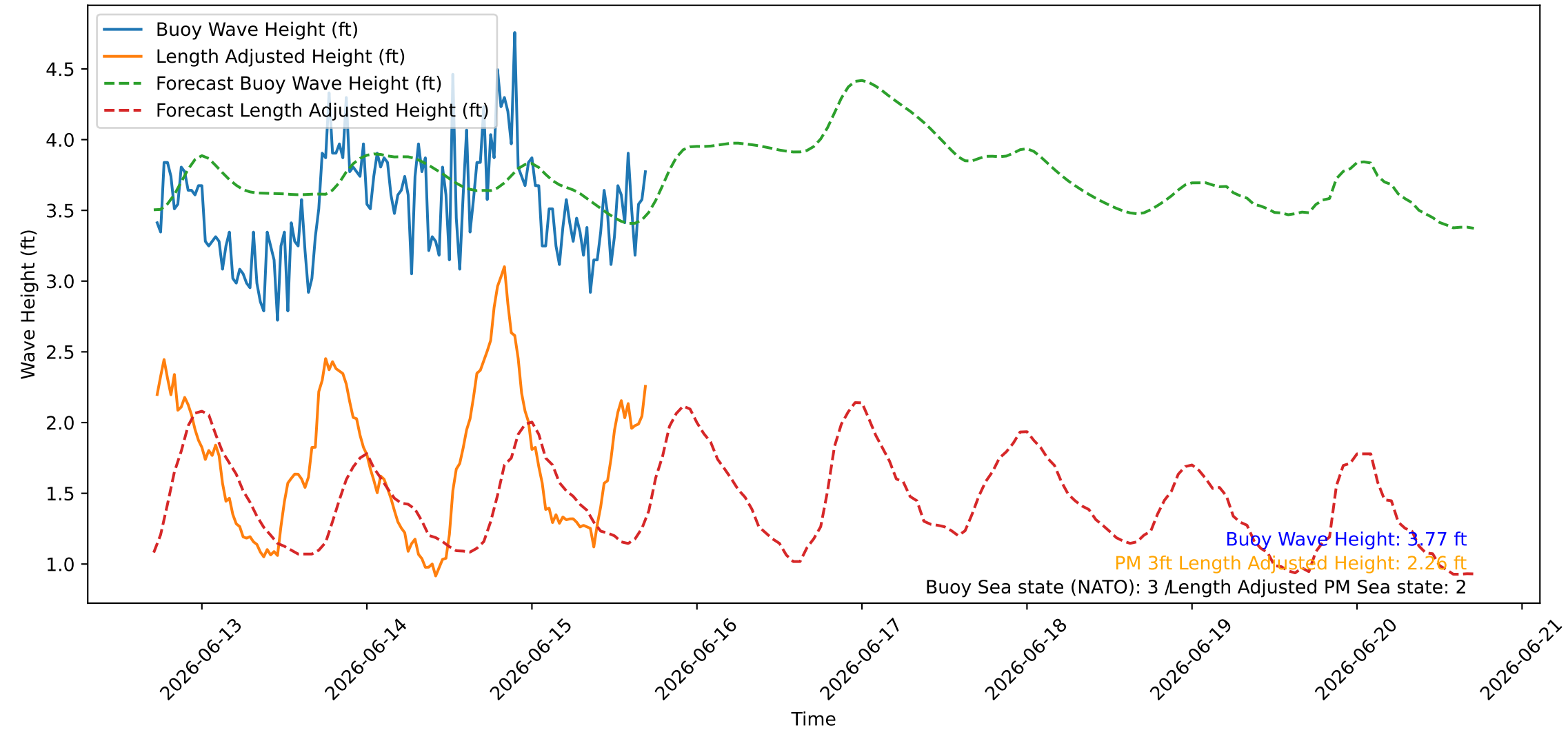
Wave Heights over Time for Red Beach at 2026-06-15 17:20:46
