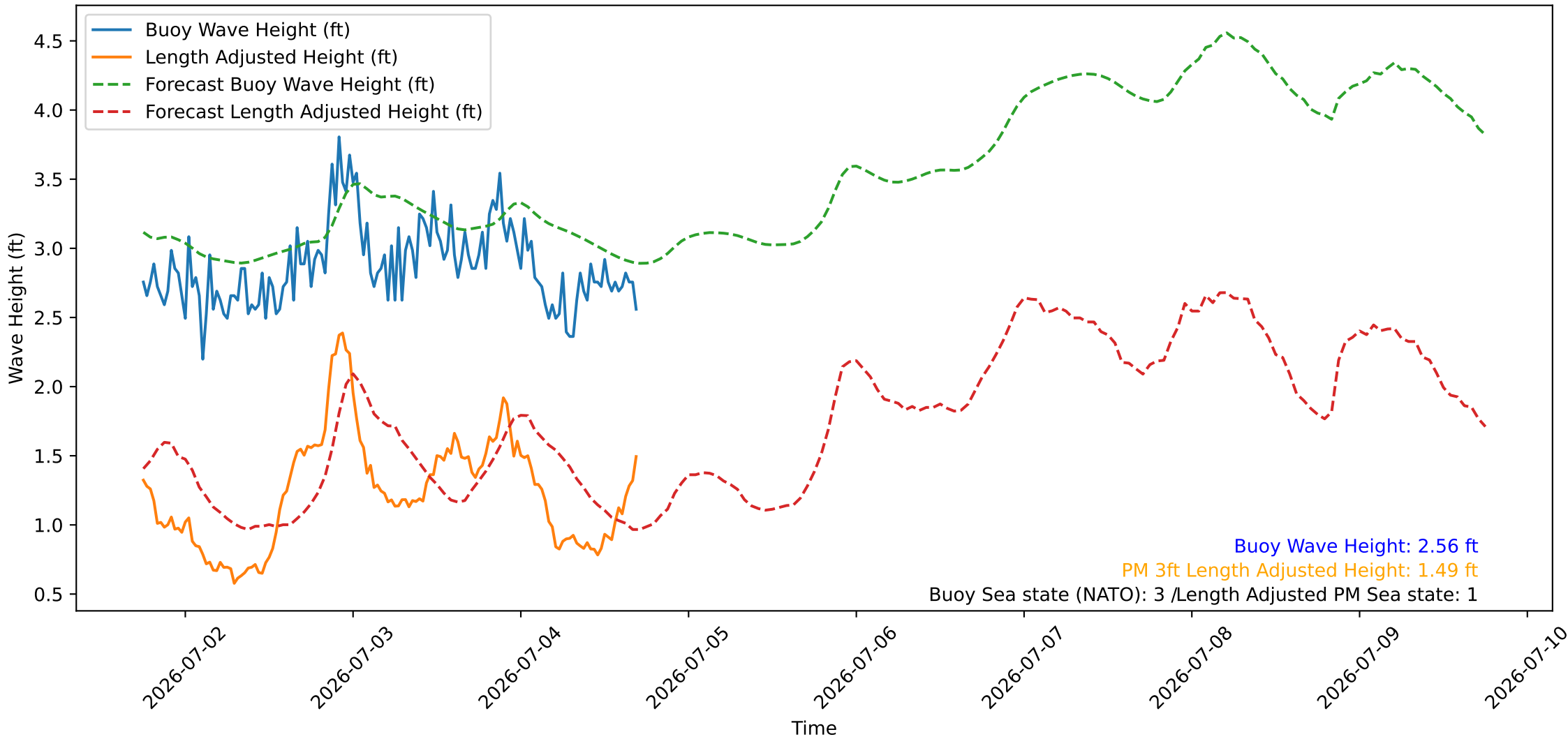
Wave Heights over Time for Red Beach at 2026-07-04 17:50:47
