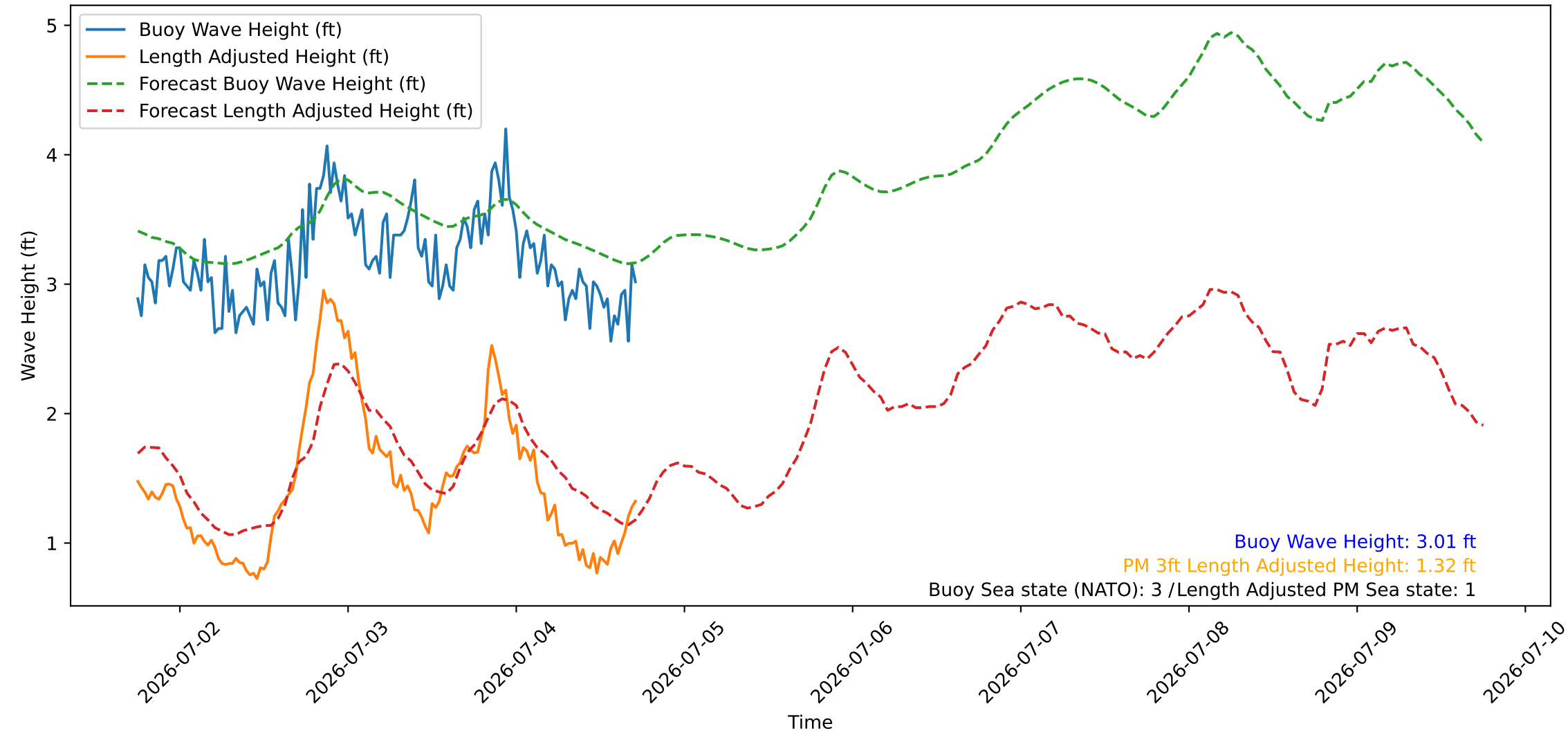
Wave Heights over Time for Green Beach at 2026-07-04 17:51:10
