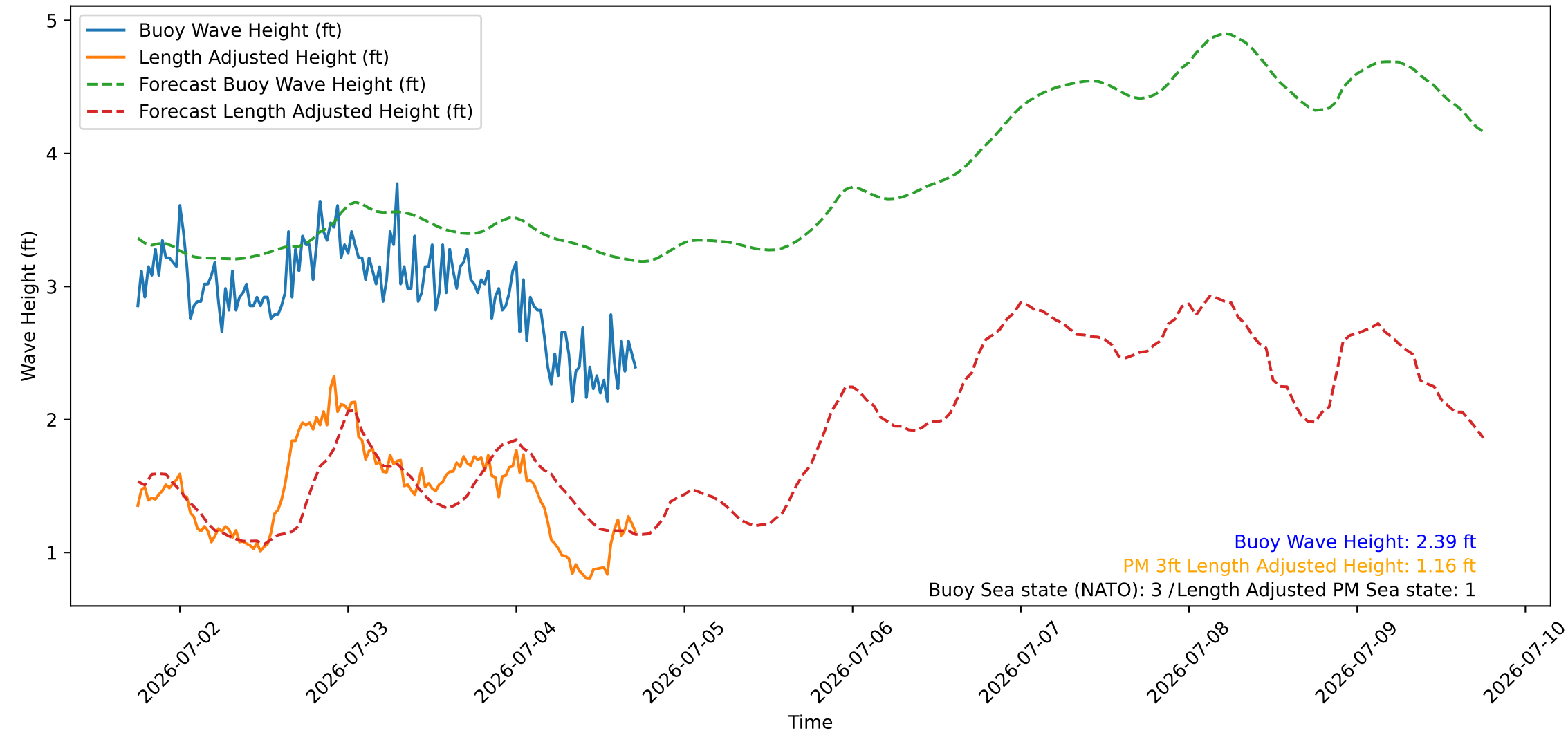
Wave Heights over Time for Oceanside Harbor at 2026-07-04 17:50:26
