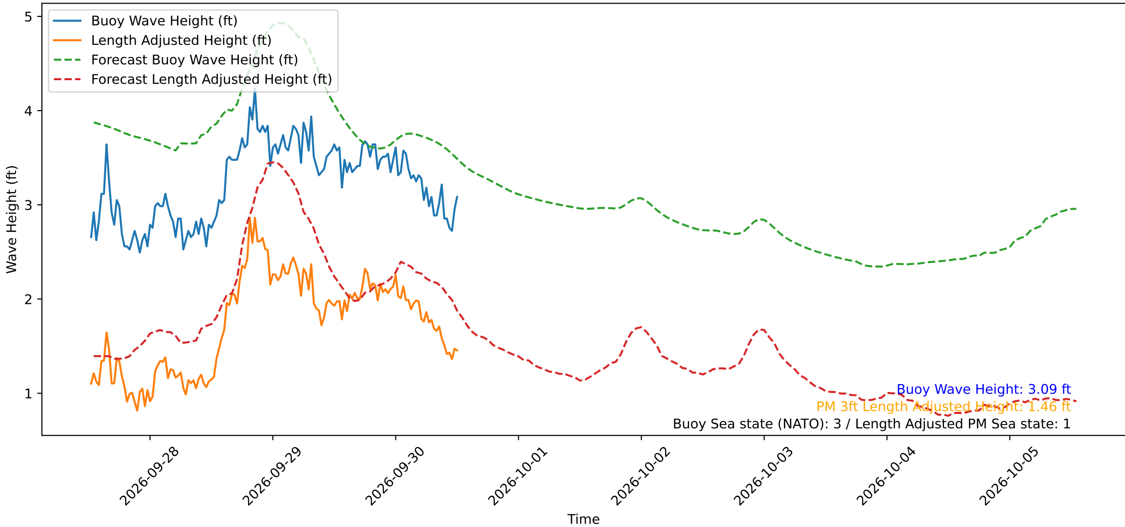
Wave Heights over Time for Oceanside Harbor at 2026-09-30 12:30:31
