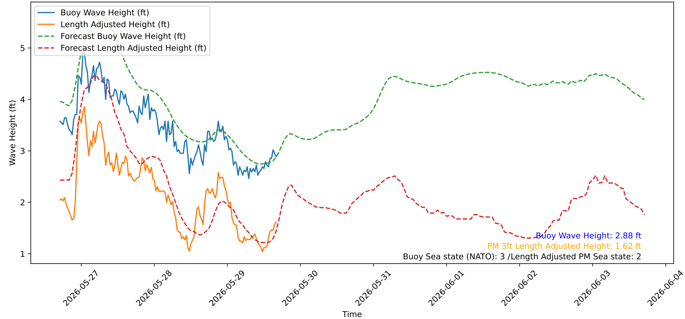
Wave Heights over Time for Green Beach at 2026-05-29 17:01:04
