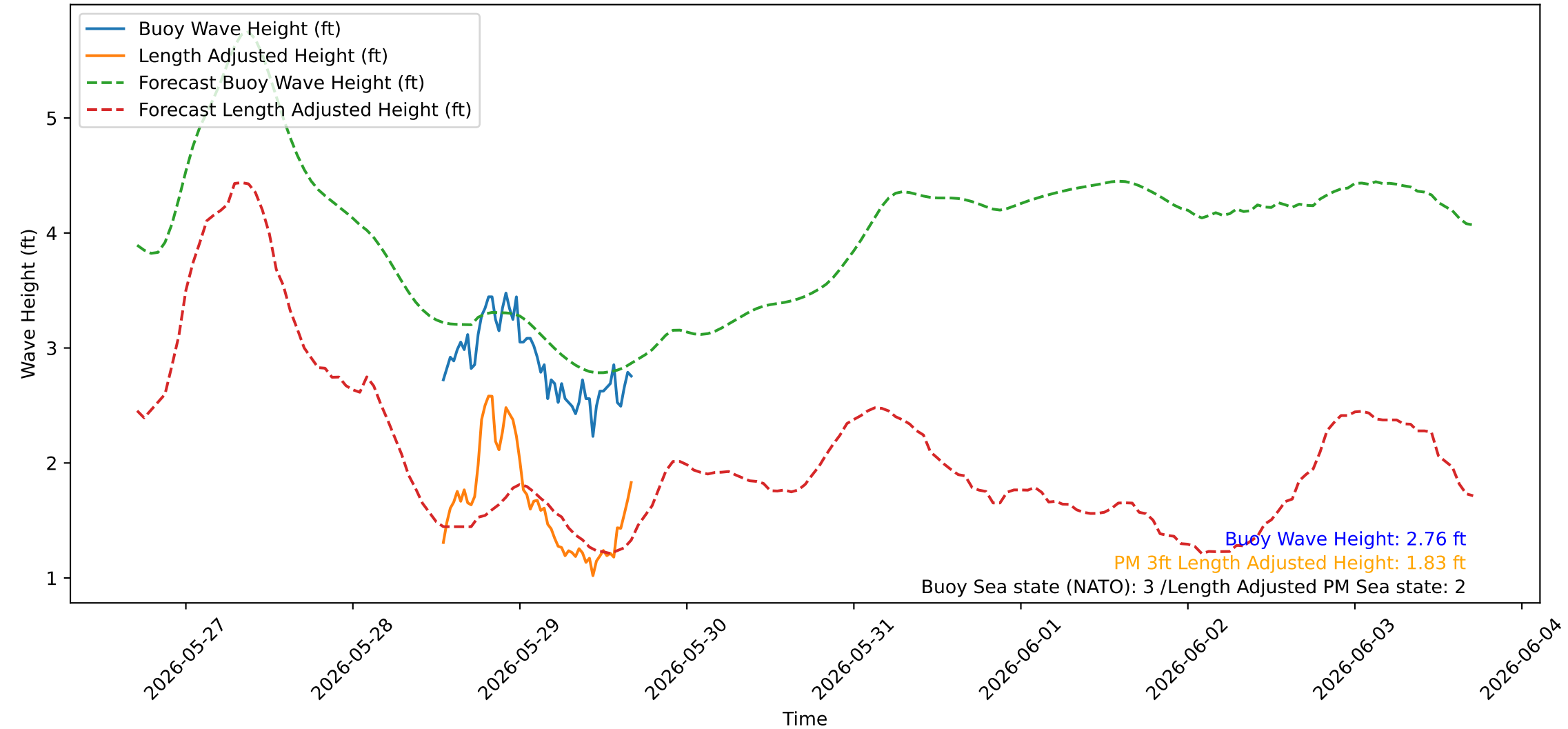
Wave Heights over Time for Oceanside Harbor at 2026-05-29 17:00:22
