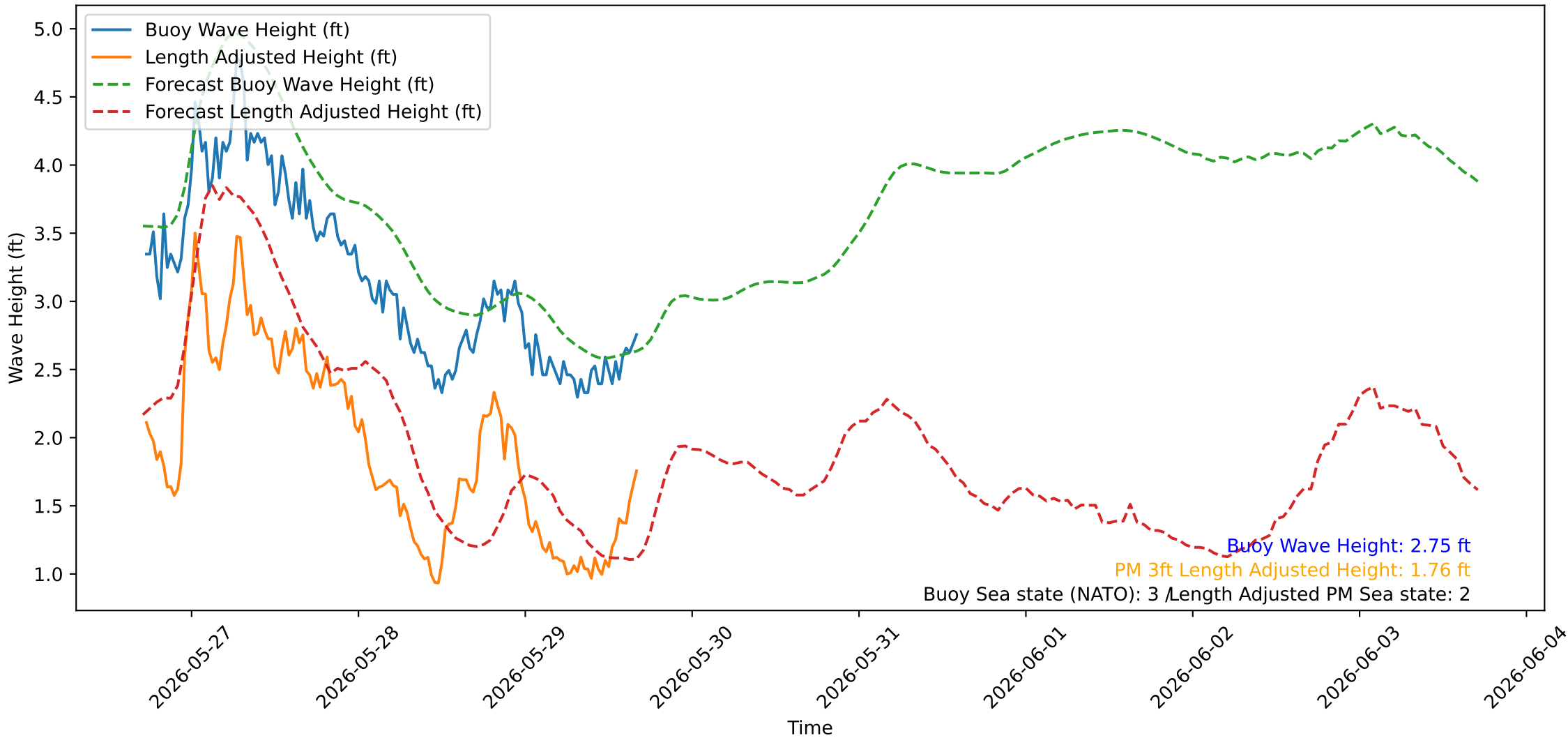
Wave Heights over Time for Red Beach at 2026-05-29 17:00:41
