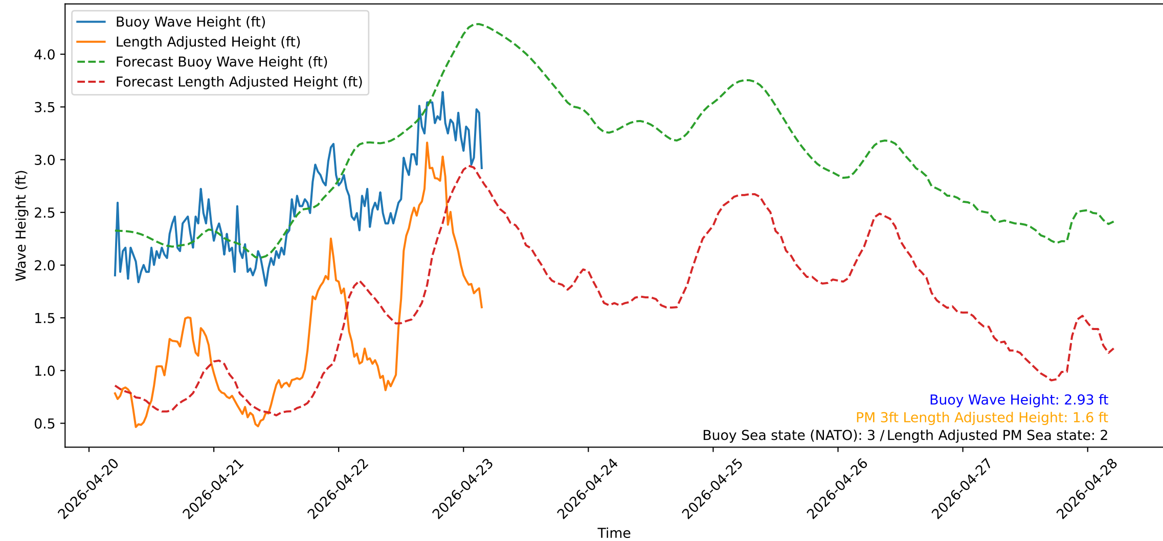
Wave Heights over Time for Red Beach at 2026-04-23 04:40:49
