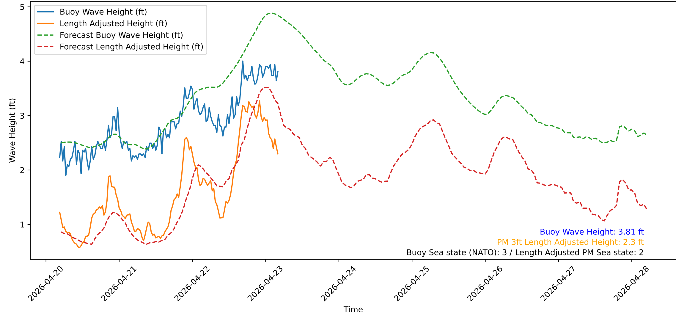
Wave Heights over Time for Green Beach at 2026-04-23 04:41:12
