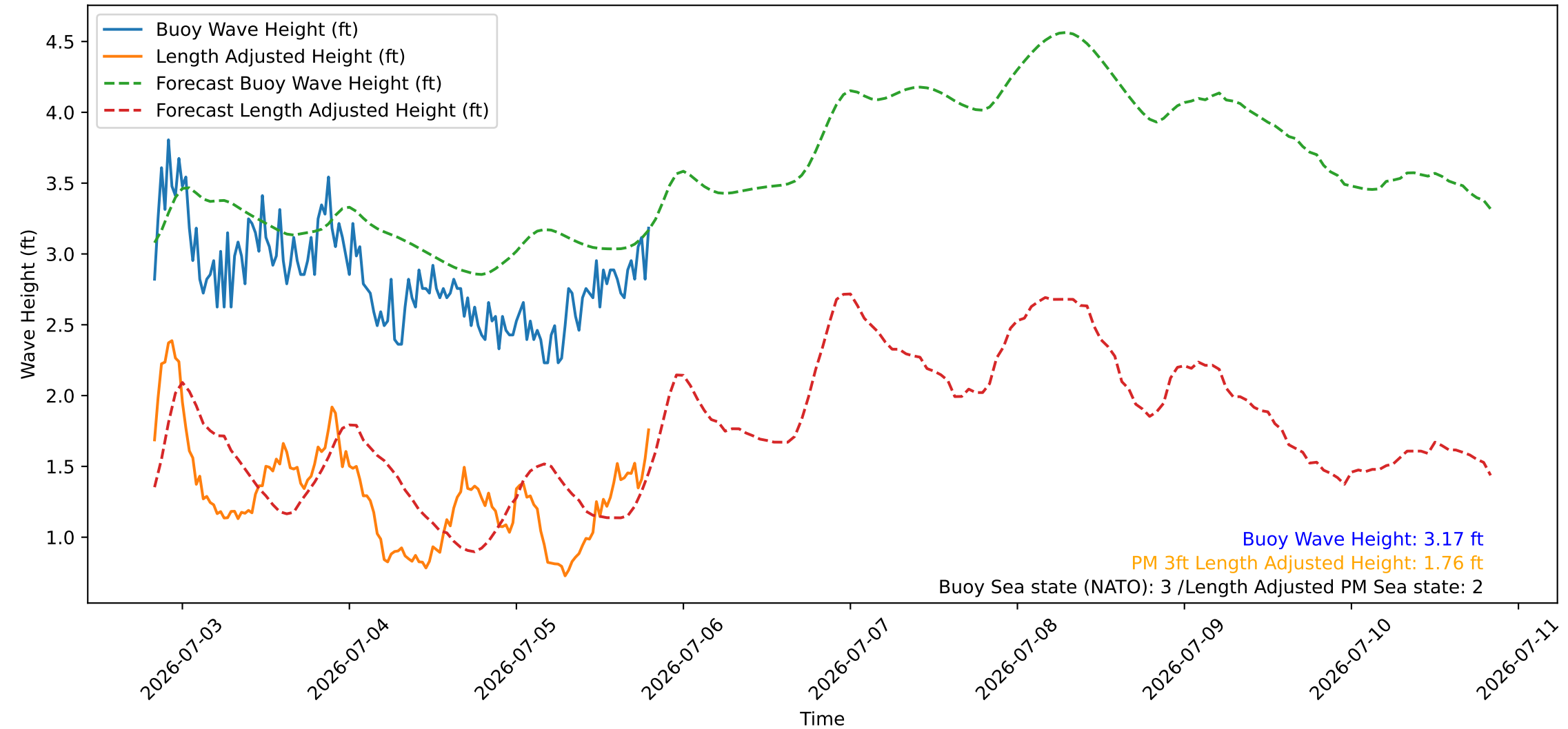
Wave Heights over Time for Red Beach at 2026-07-05 19:50:46
