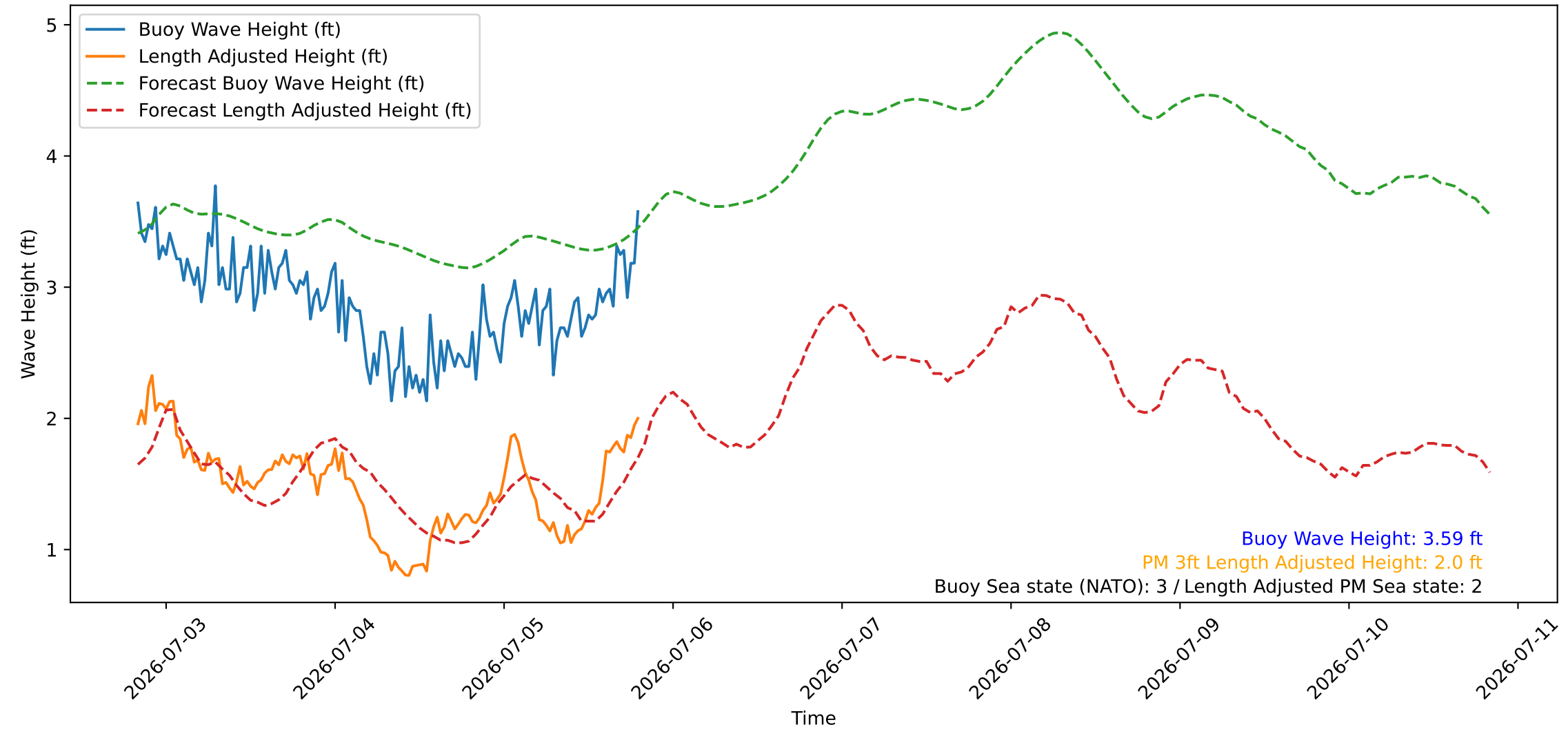
Wave Heights over Time for Oceanside Harbor at 2026-07-05 19:50:26
