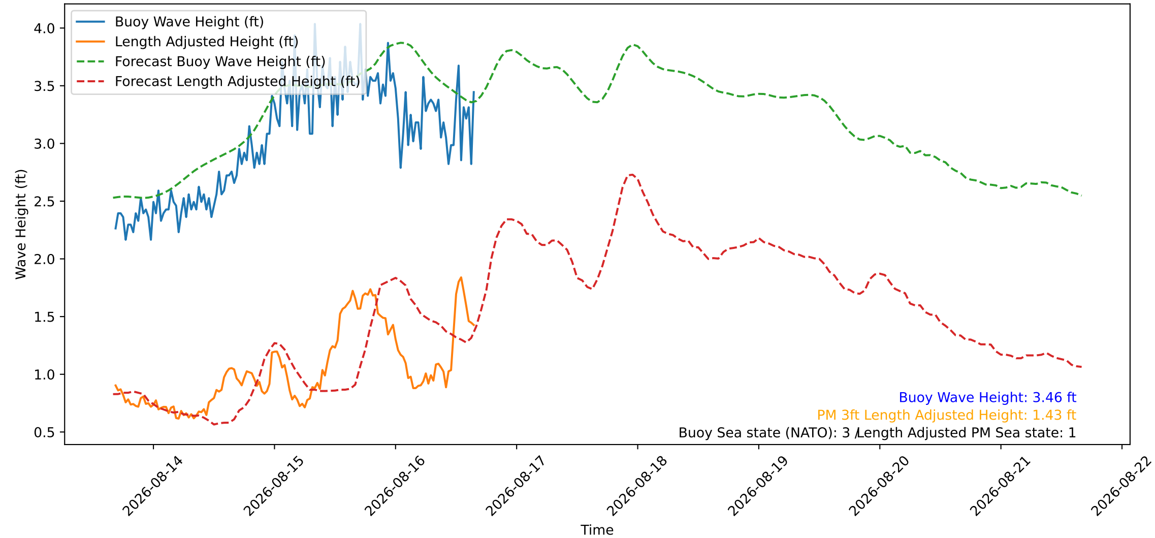
Wave Heights over Time for Red Beach at 2026-08-16 16:20:47
