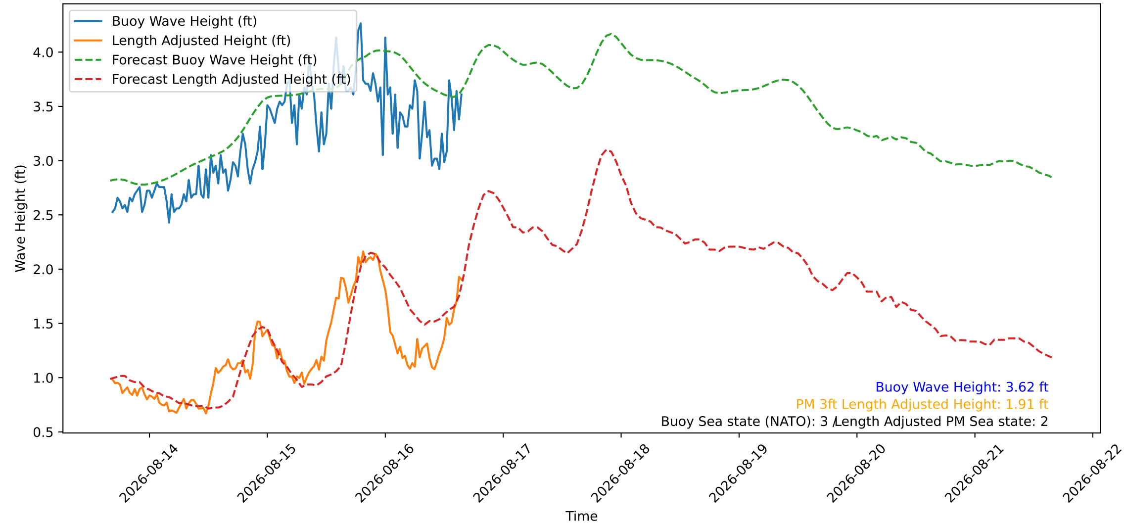
Wave Heights over Time for Green Beach at 2026-08-16 16:21:10
