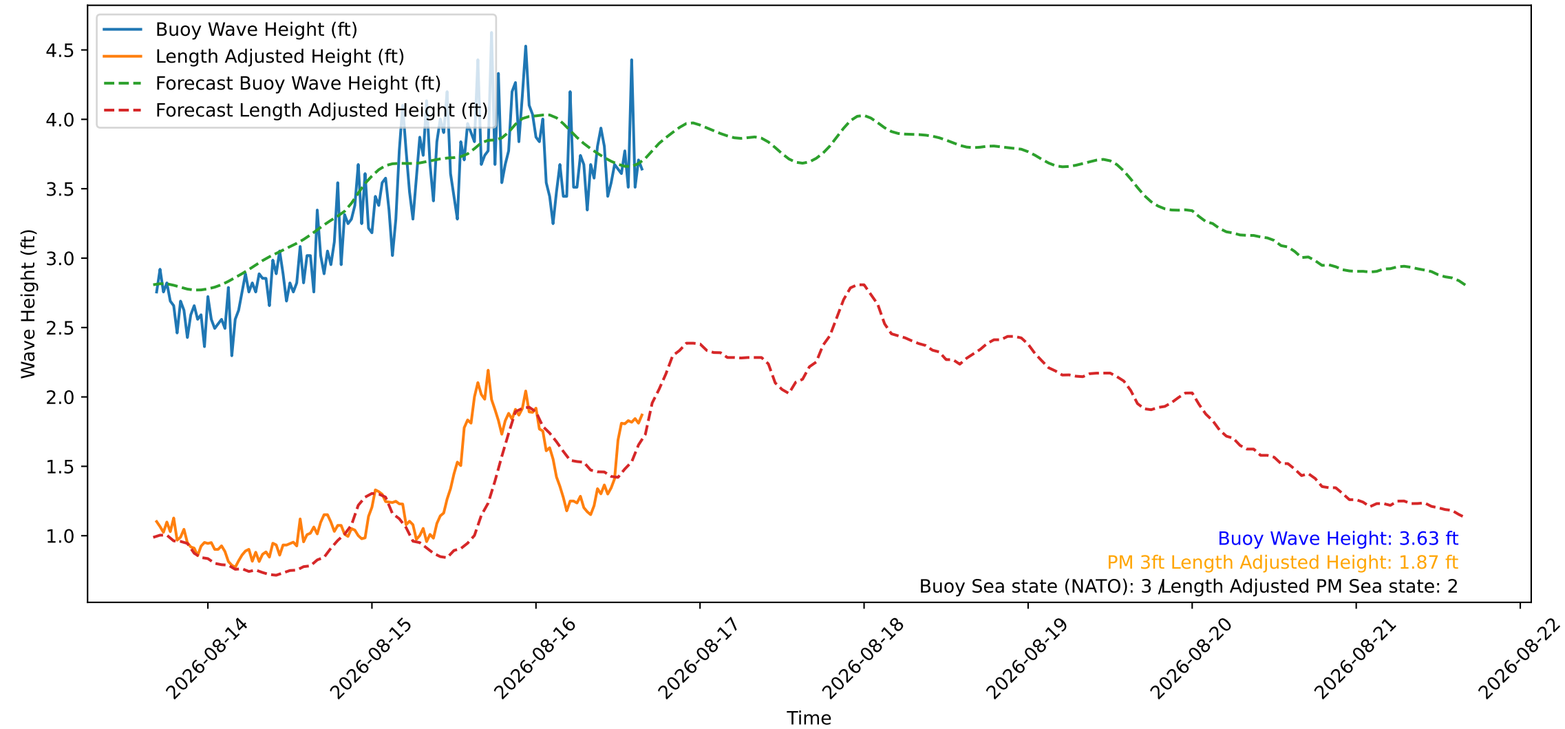
Wave Heights over Time for Oceanside Harbor at 2026-08-16 16:20:26
