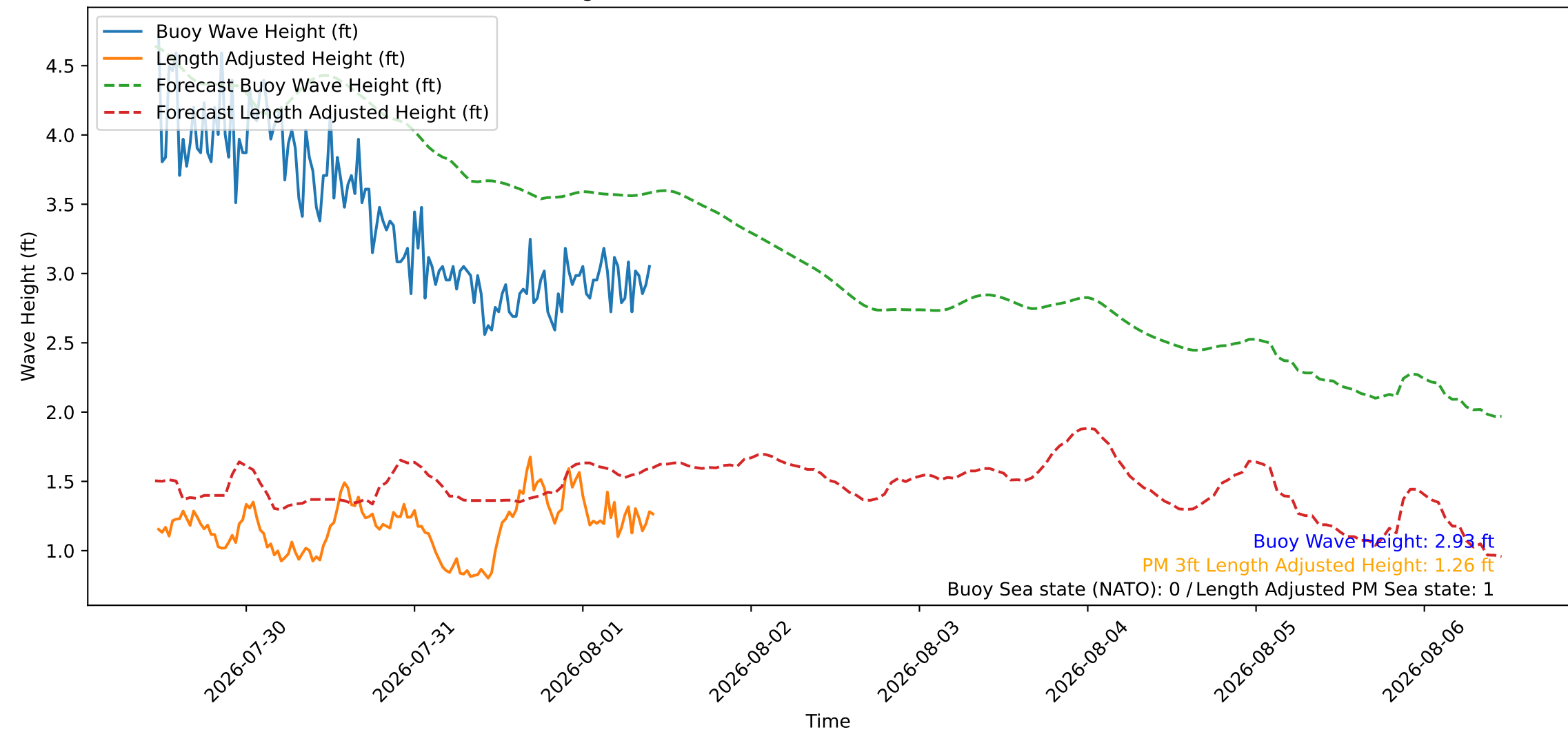
Wave Heights over Time for Red Beach at 2026-08-01 11:00:46
