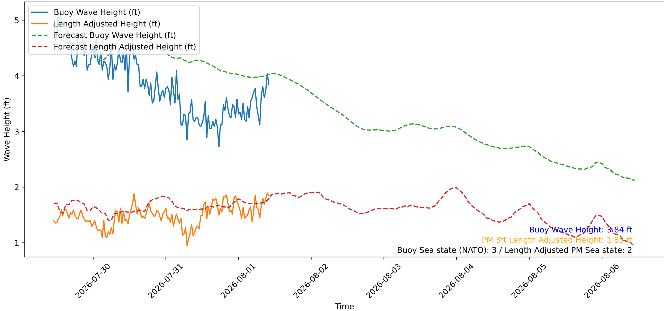
Wave Heights over Time for Oceanside Harbor at 2026-08-01 11:00:26
