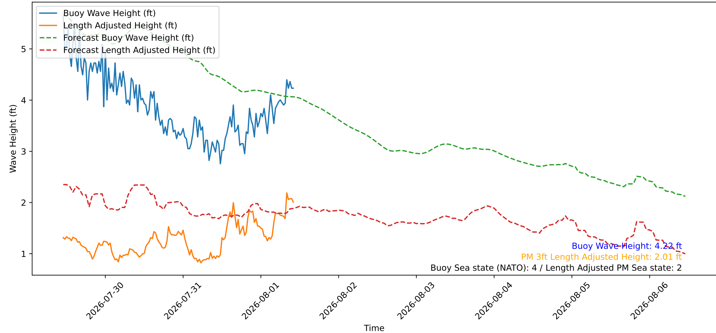
Wave Heights over Time for Green Beach at 2026-08-01 11:01:08
