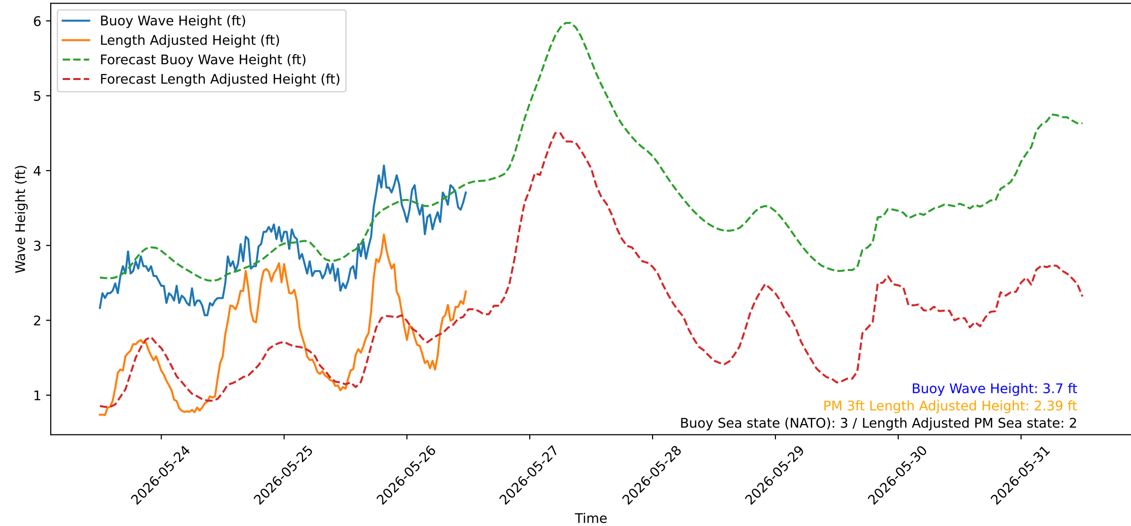
Wave Heights over Time for Green Beach at 2026-05-26 12:11:10
