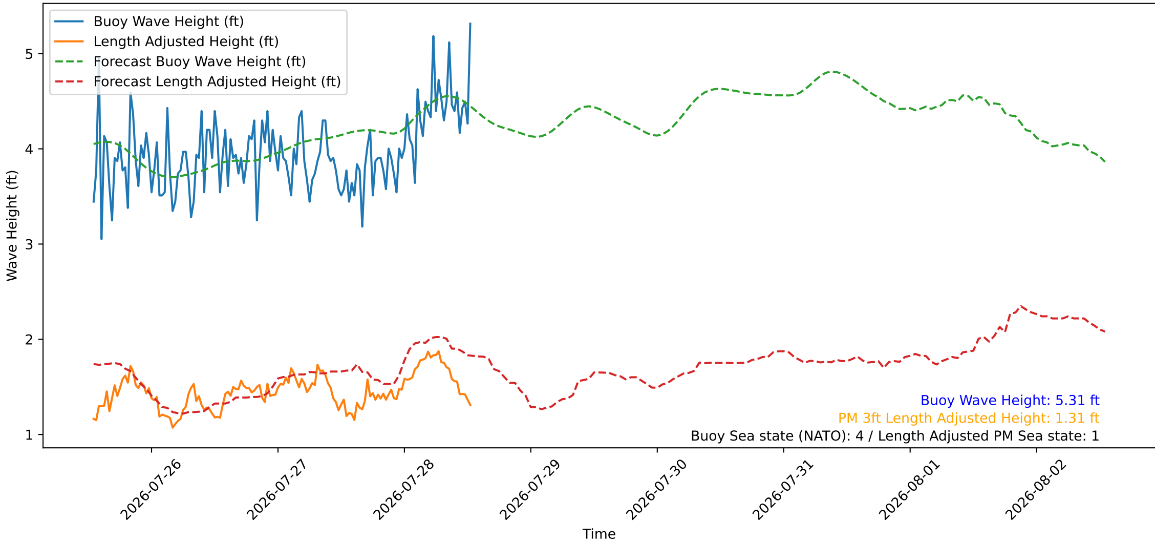
Wave Heights over Time for Oceanside Harbor at 2026-07-28 13:10:26
