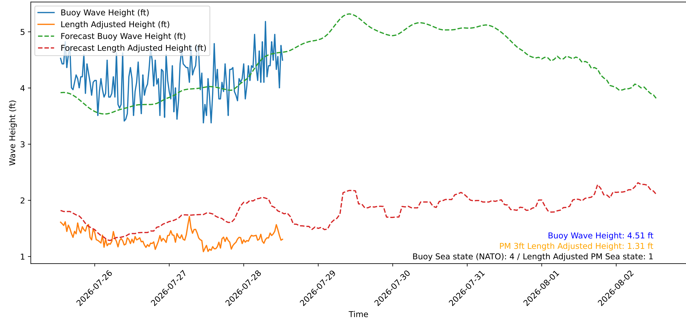
Wave Heights over Time for Green Beach at 2026-07-28 13:11:07
