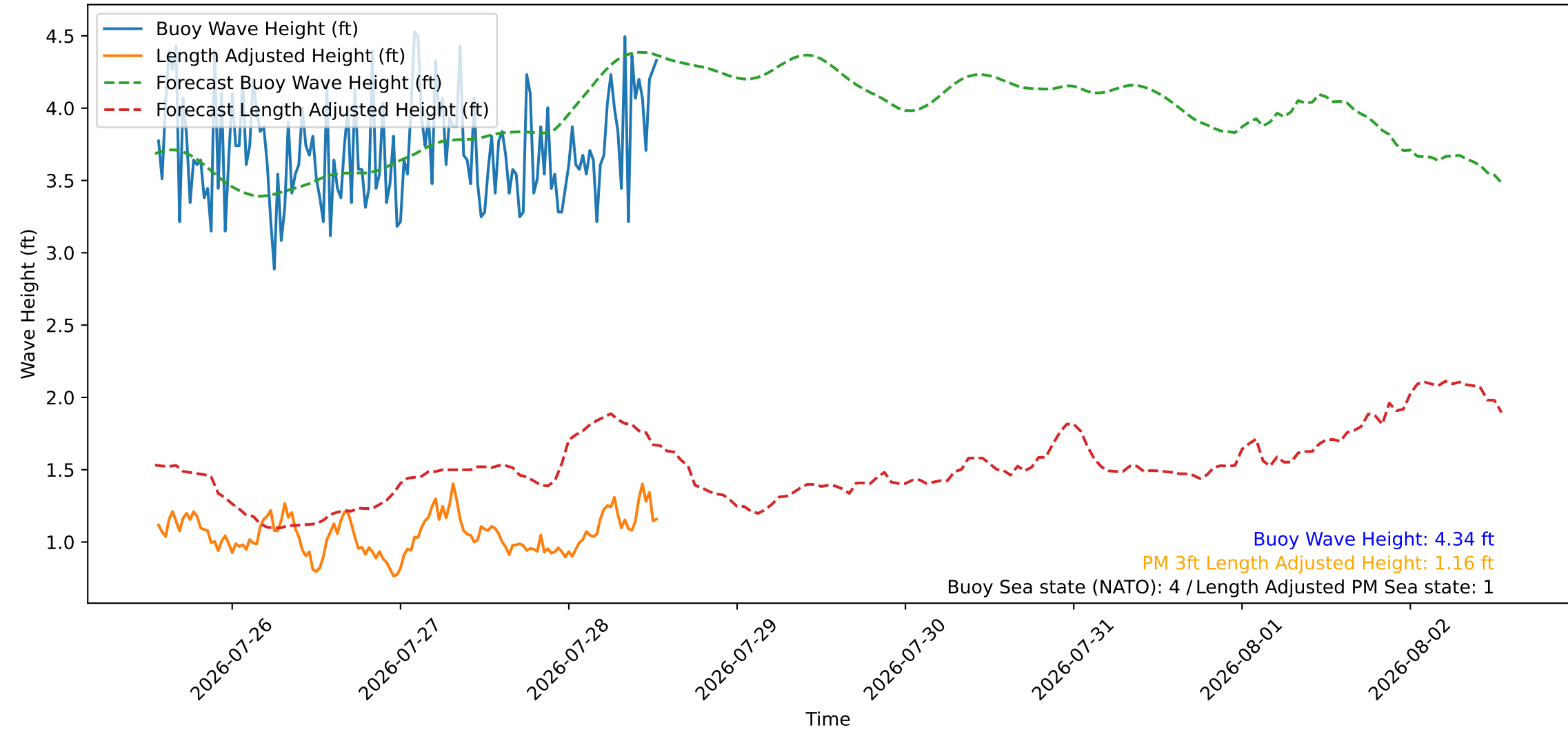
Wave Heights over Time for Red Beach at 2026-07-28 13:10:45
