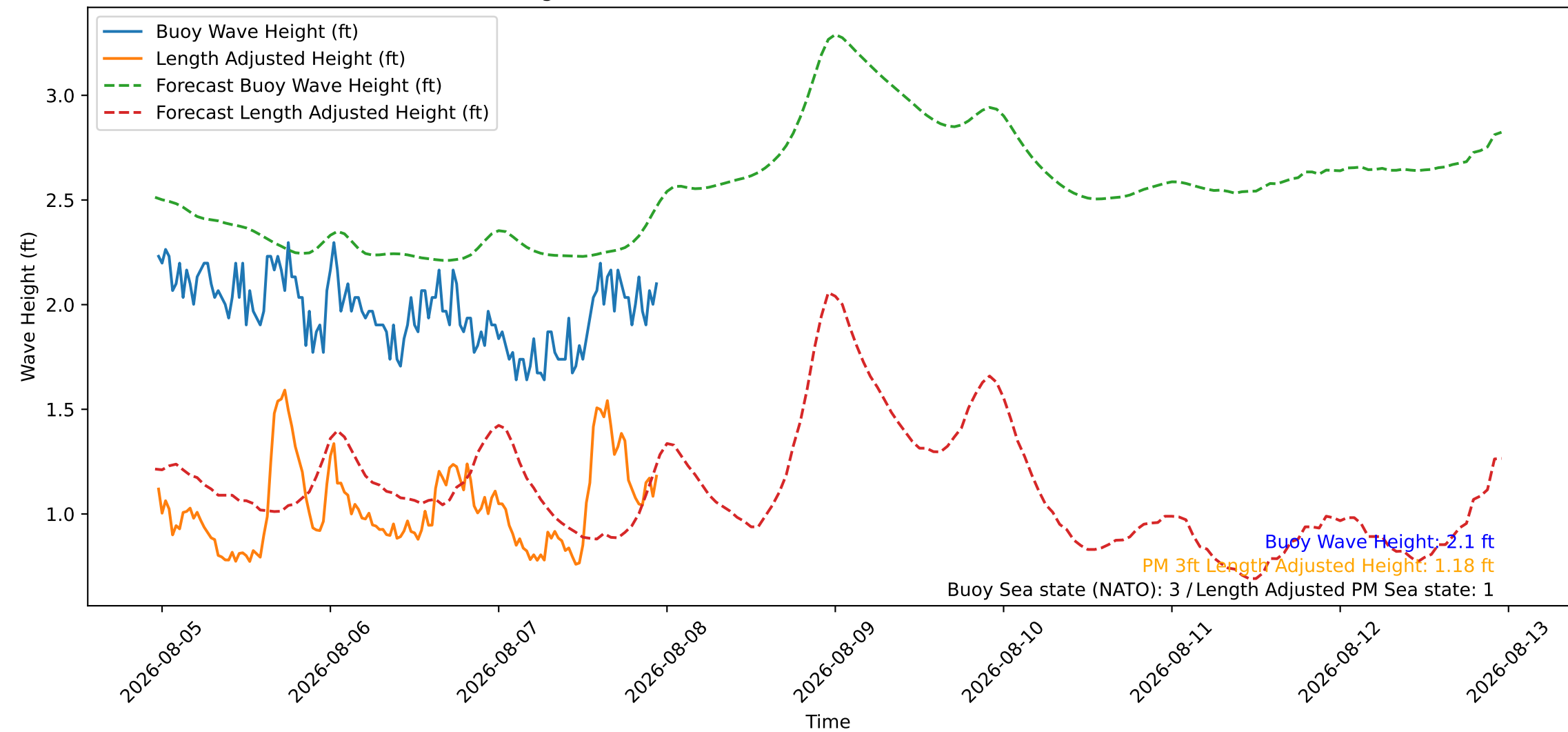
Wave Heights over Time for Oceanside Harbor at 2026-08-07 23:20:27
