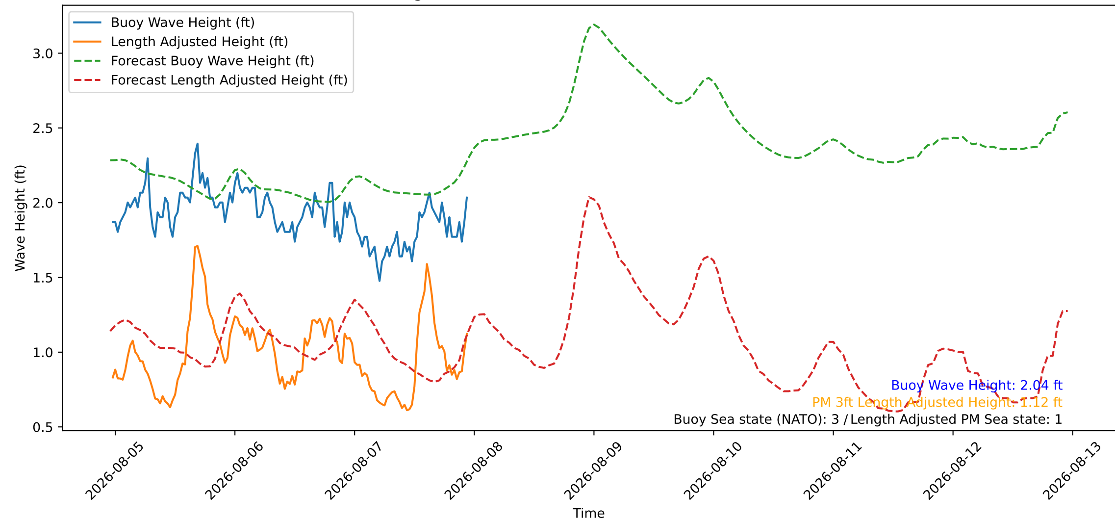
Wave Heights over Time for Red Beach at 2026-08-07 23:20:48
