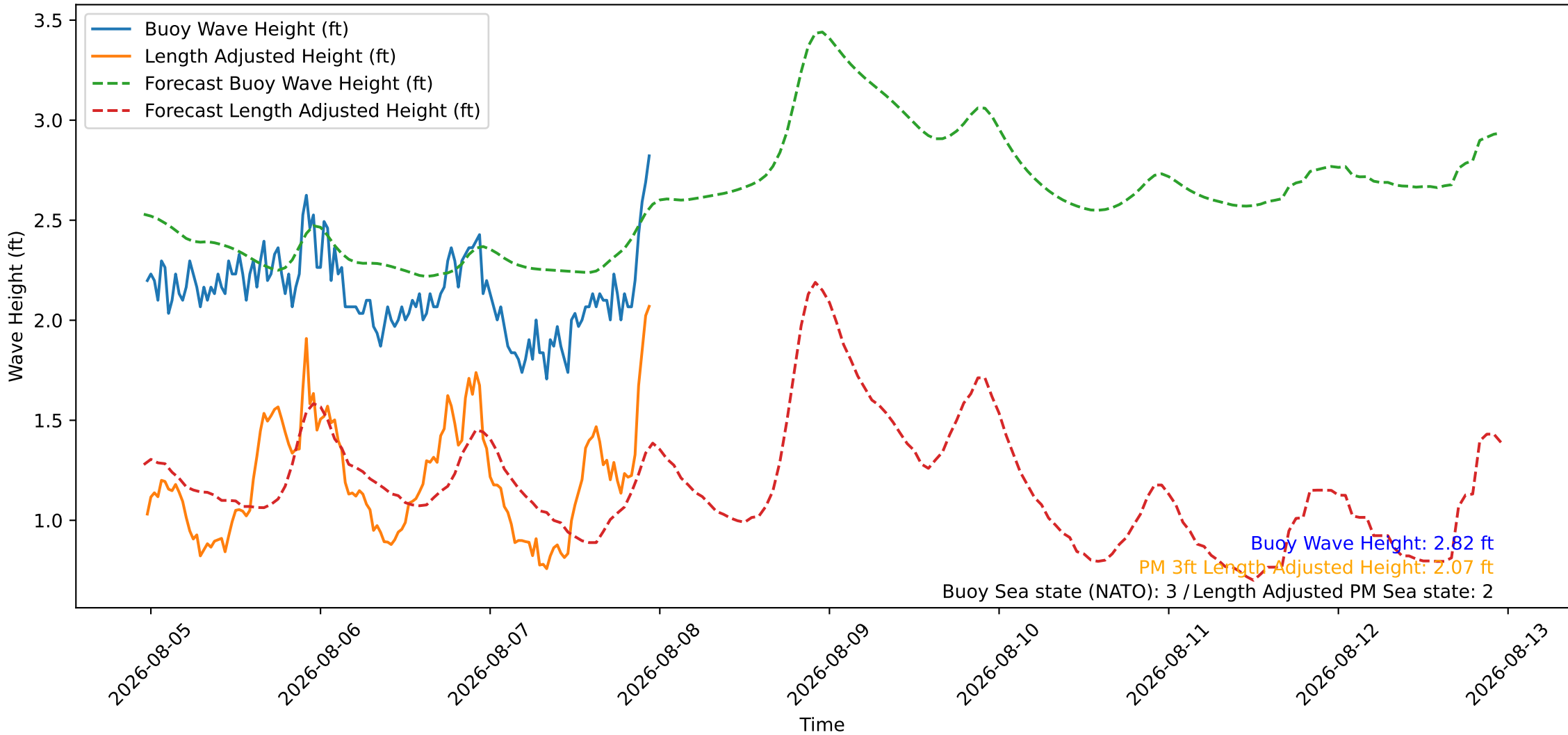
Wave Heights over Time for Green Beach at 2026-08-07 23:21:10
