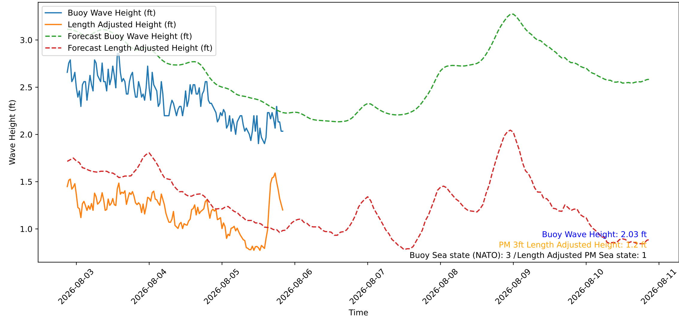
Wave Heights over Time for Oceanside Harbor at 2026-08-05 20:50:26
