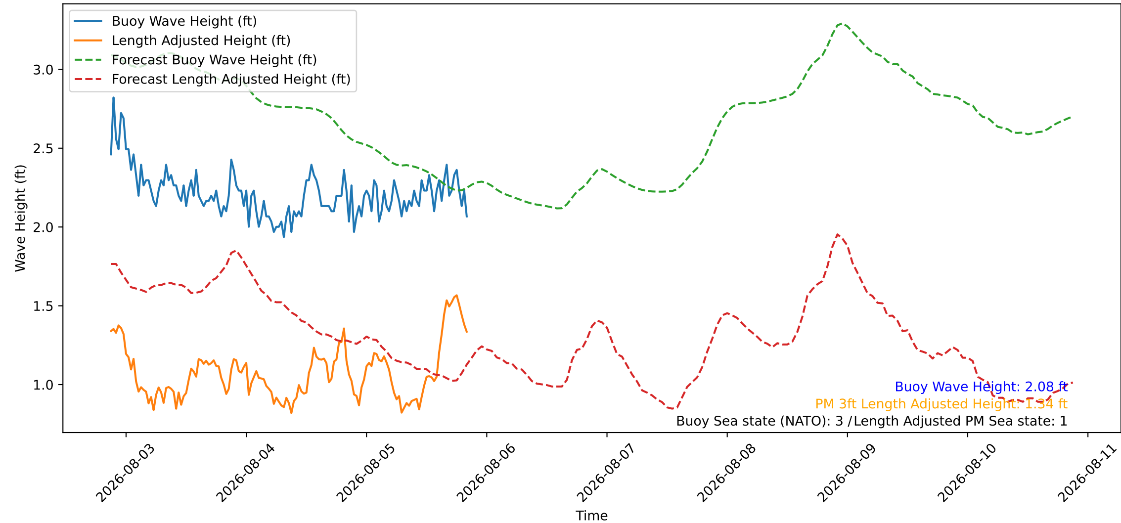
Wave Heights over Time for Green Beach at 2026-08-05 20:51:09
