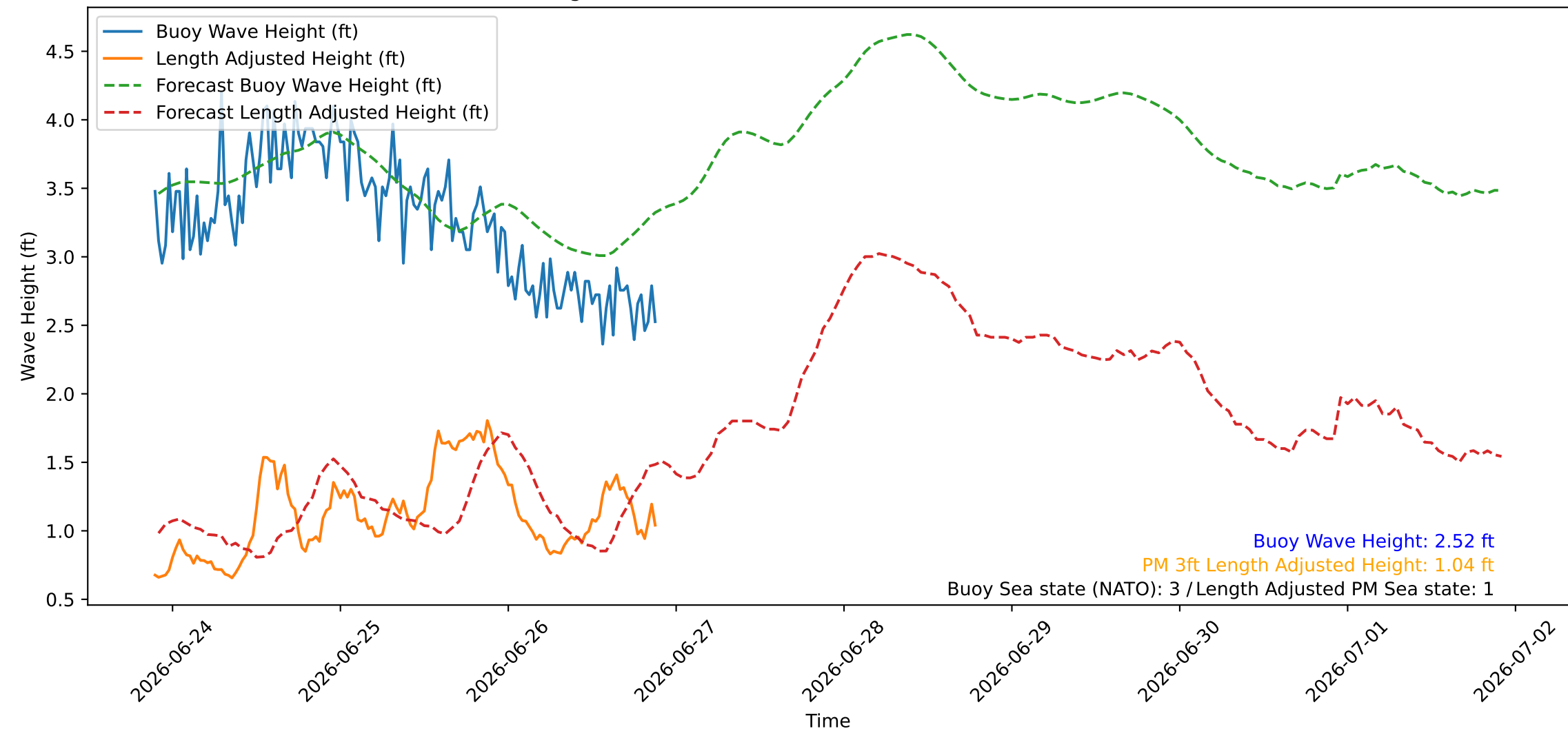
Wave Heights over Time for Green Beach at 2026-06-26 21:41:08
