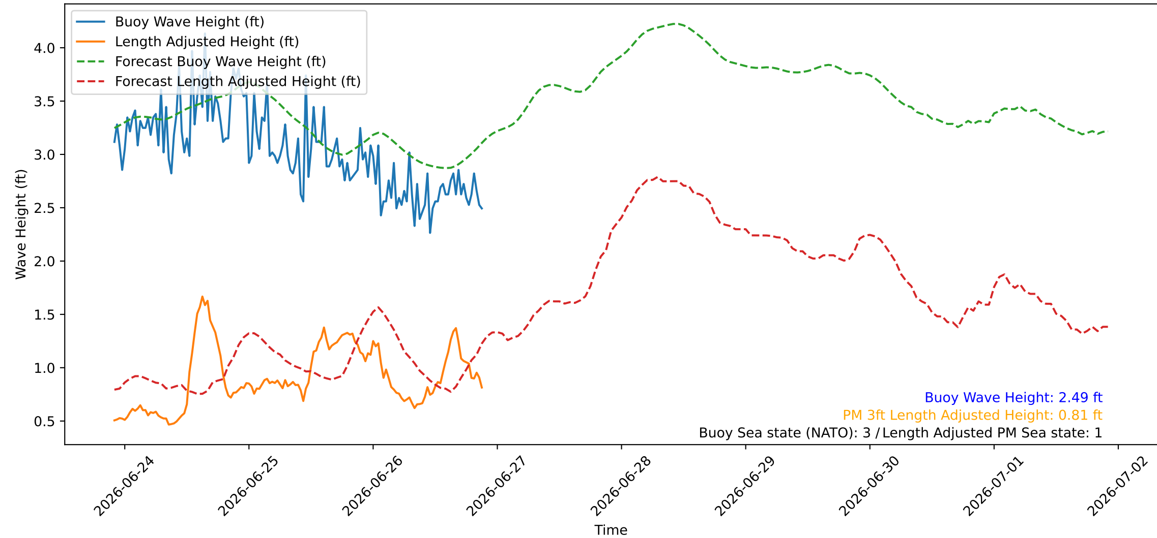
Wave Heights over Time for Red Beach at 2026-06-26 21:40:45
