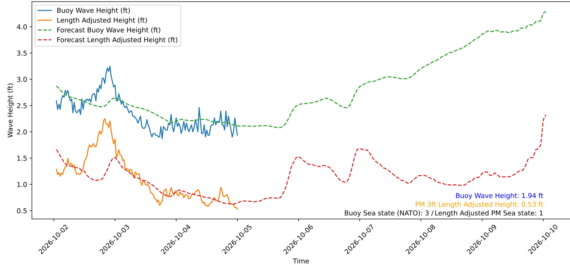
Wave Heights over Time for Red Beach at 2026-10-05 00:50:50
