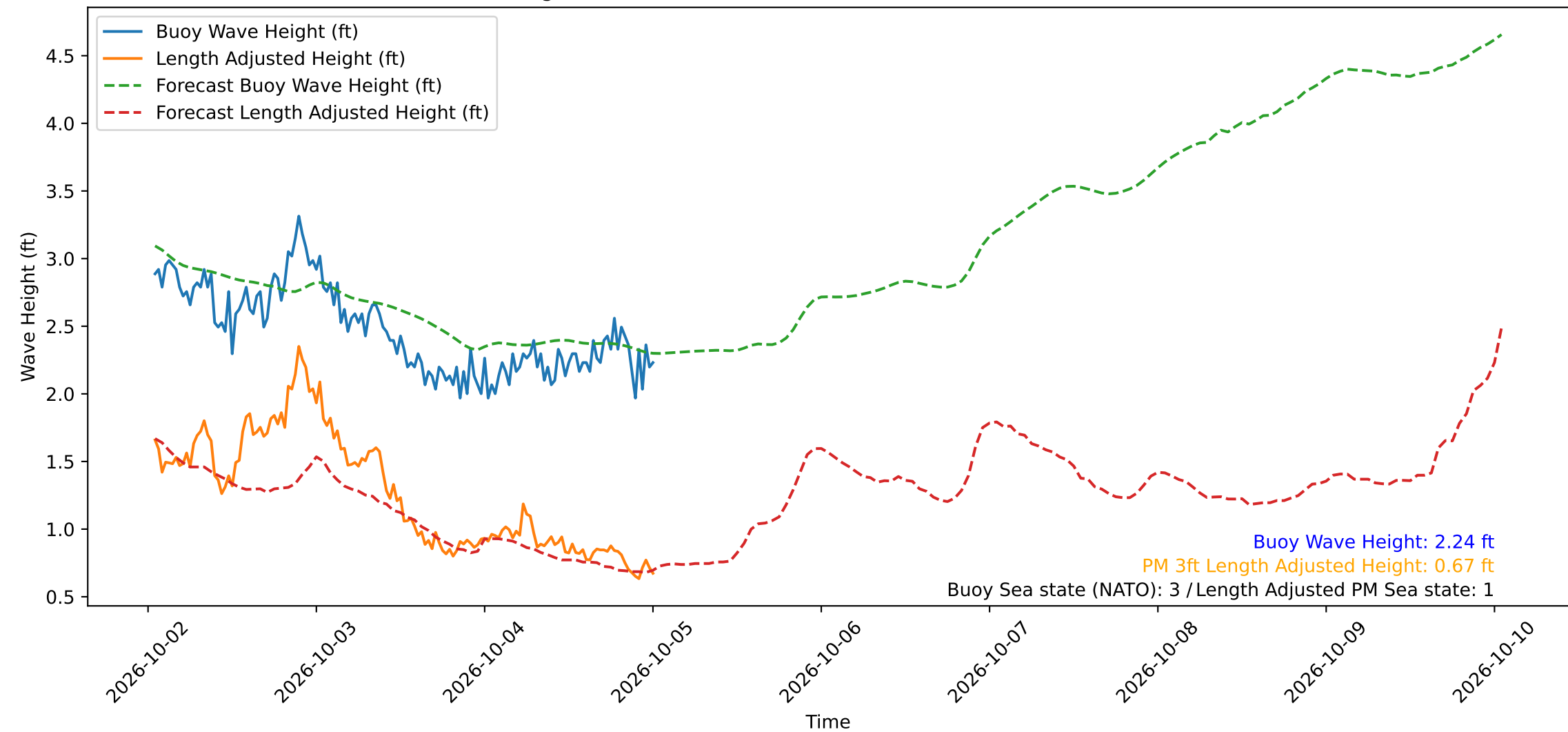
Wave Heights over Time for Oceanside Harbor at 2026-10-05 00:50:30
