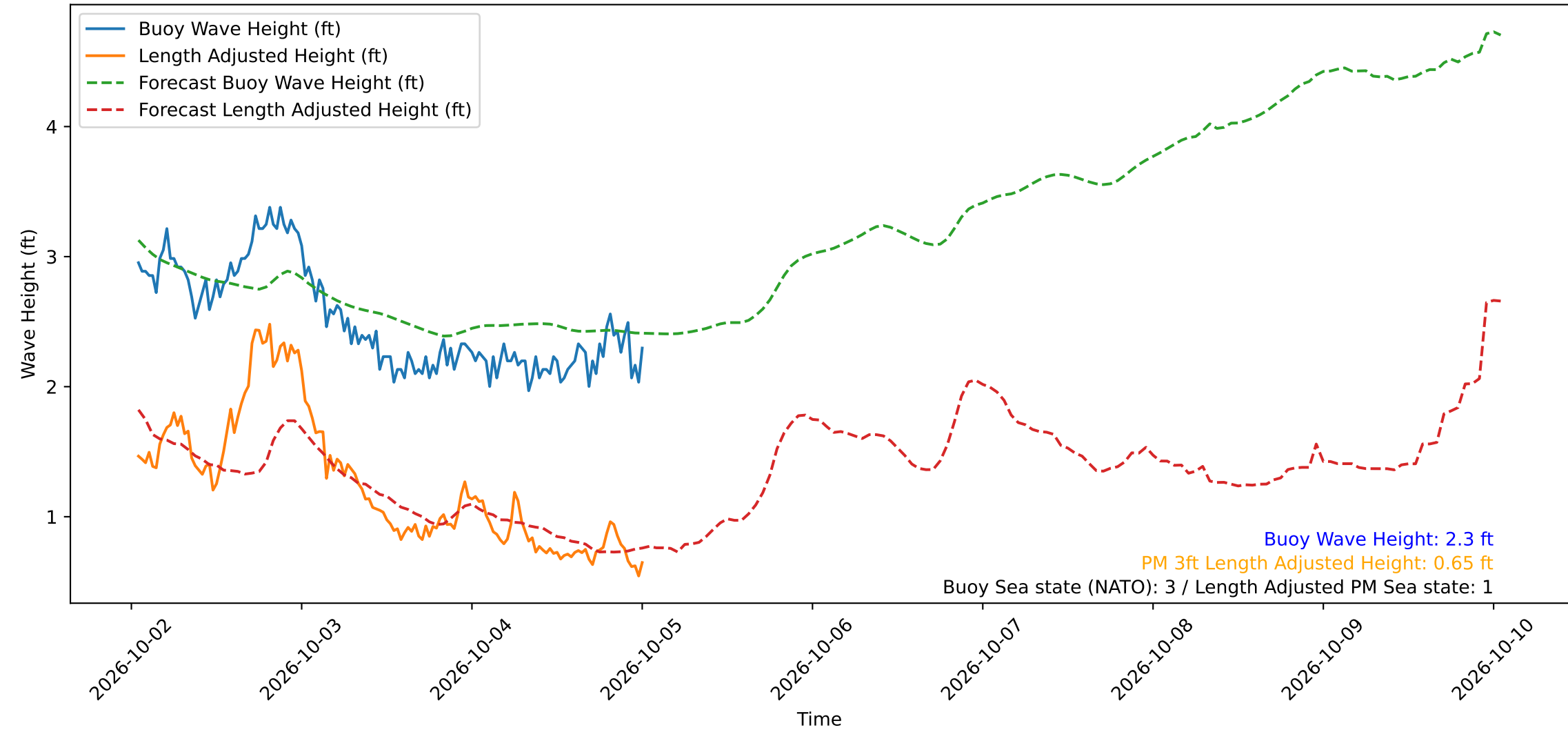
Wave Heights over Time for Green Beach at 2026-10-05 00:51:14
