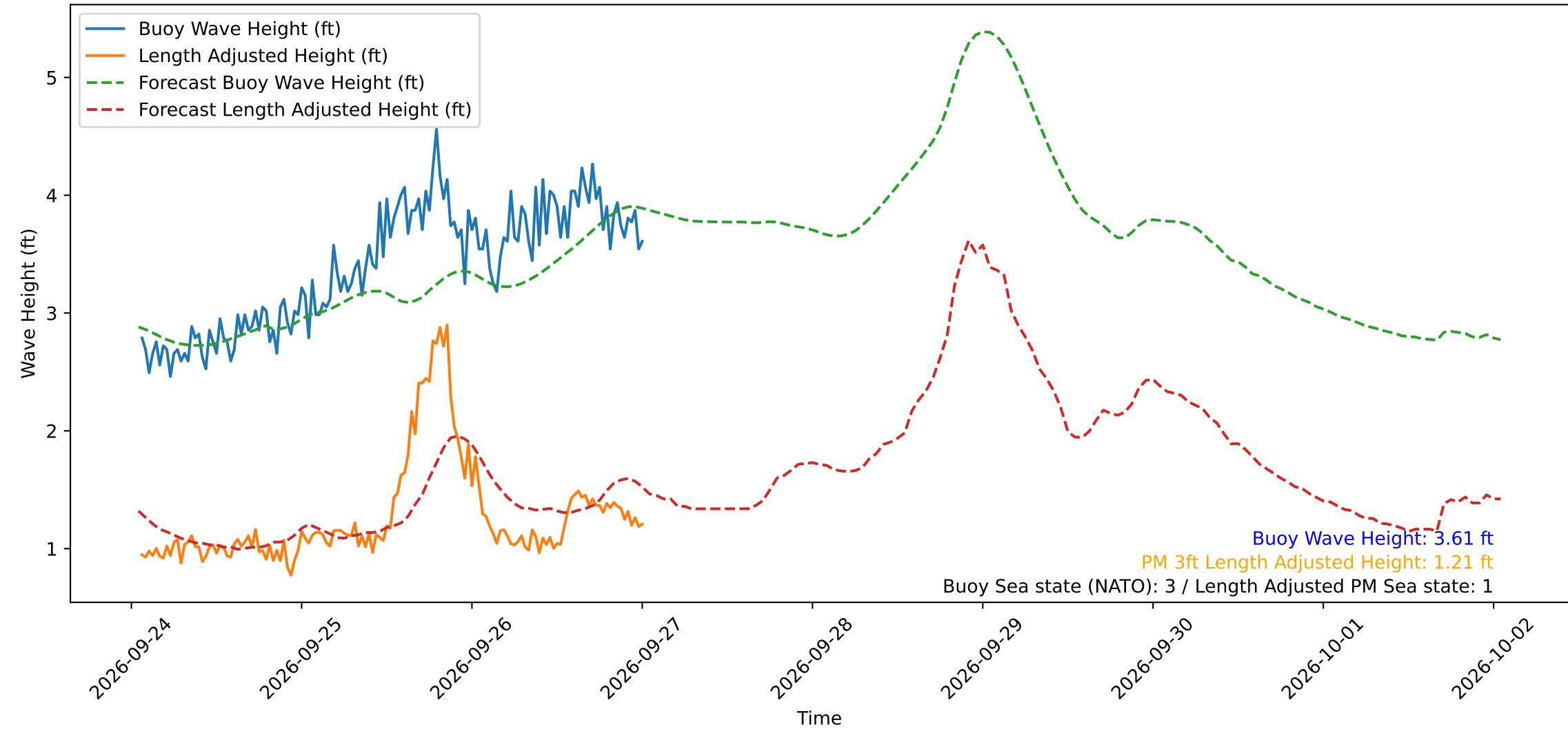
Wave Heights over Time for Green Beach at 2026-09-27 01:01:15
