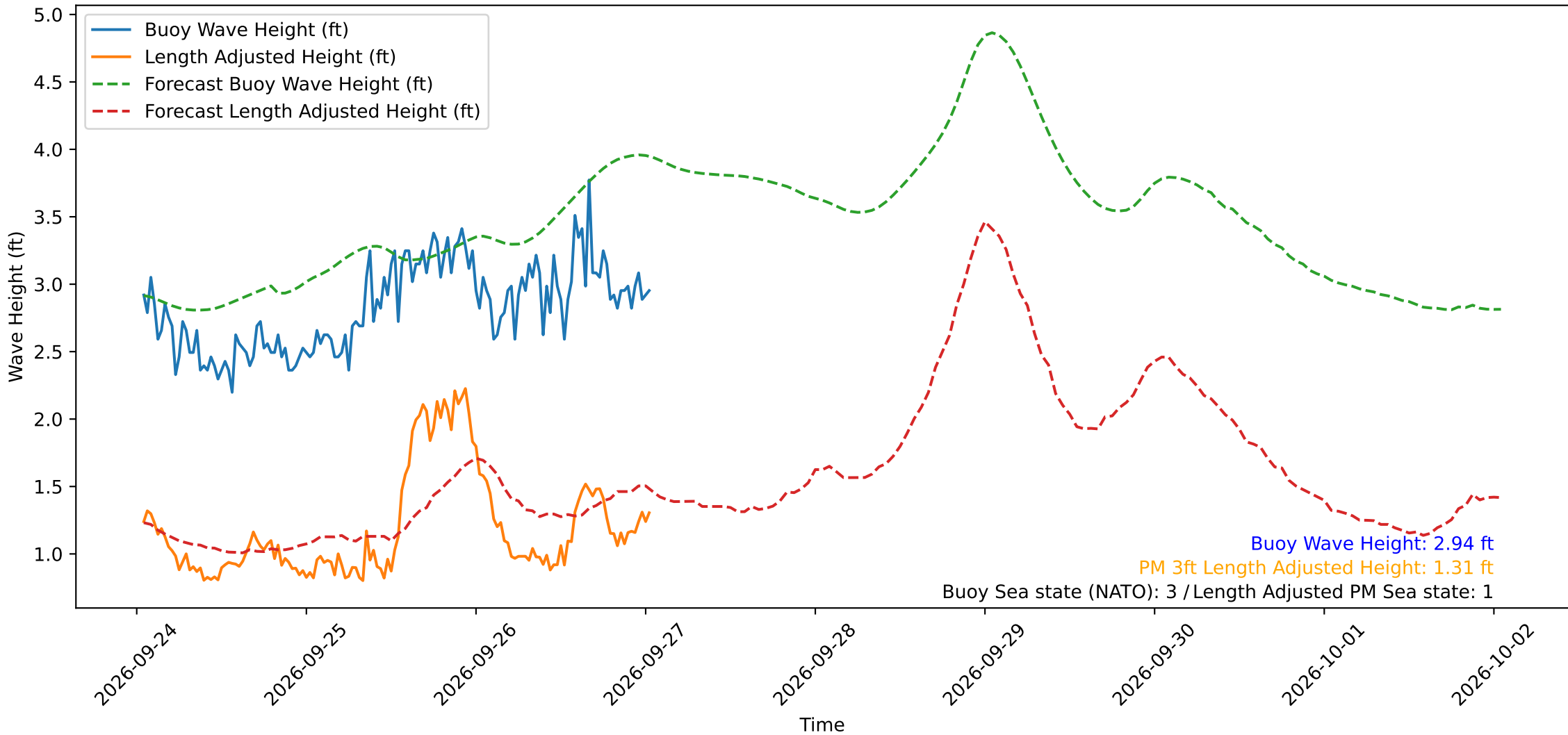
Wave Heights over Time for Oceanside Harbor at 2026-09-27 01:00:31
