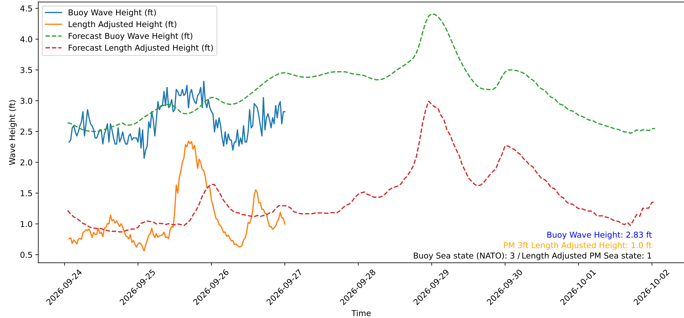
Wave Heights over Time for Red Beach at 2026-09-27 01:00:51
