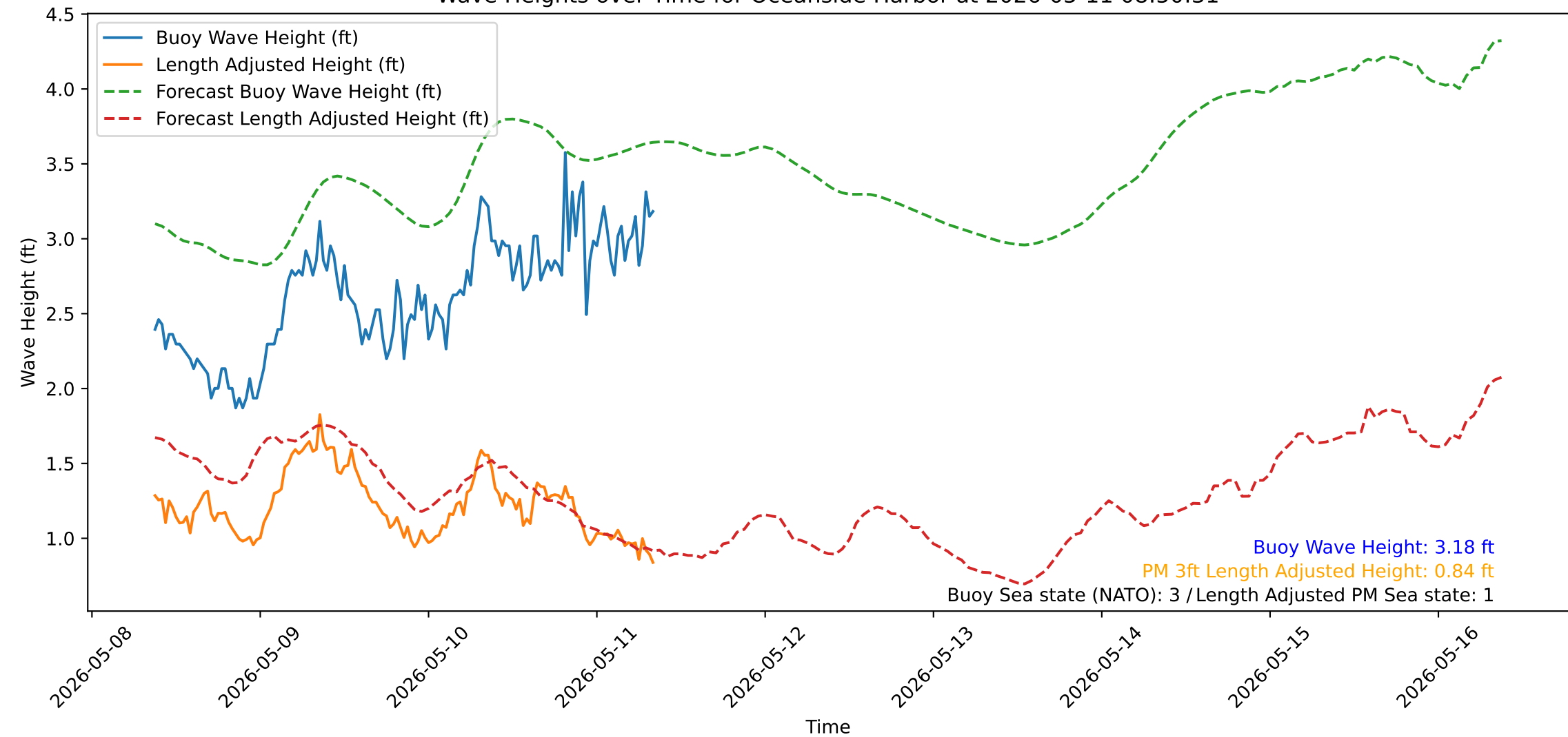
Wave Heights over Time for Oceanside Harbor at 2026-05-11 08:50:31
