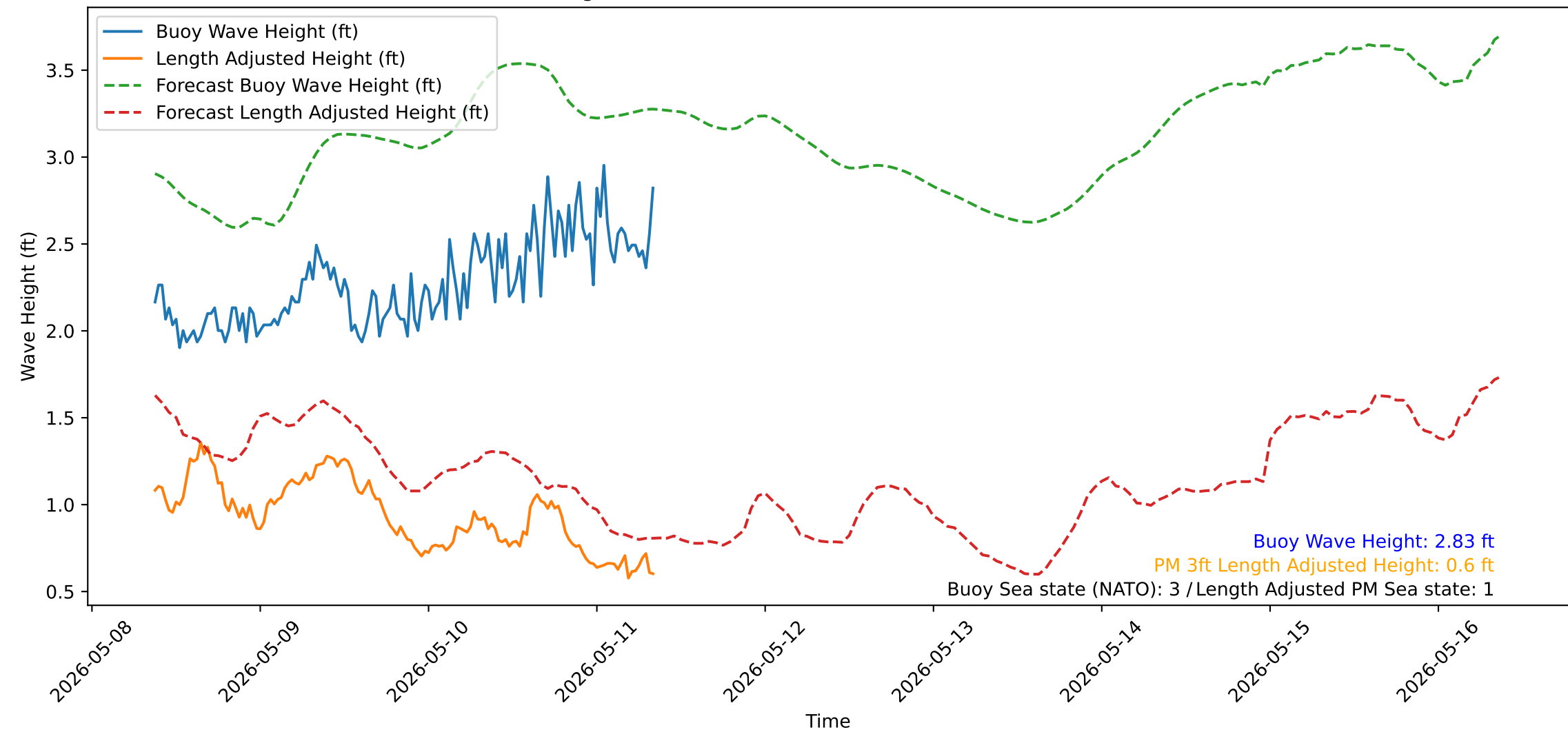
Wave Heights over Time for Red Beach at 2026-05-11 08:50:51
