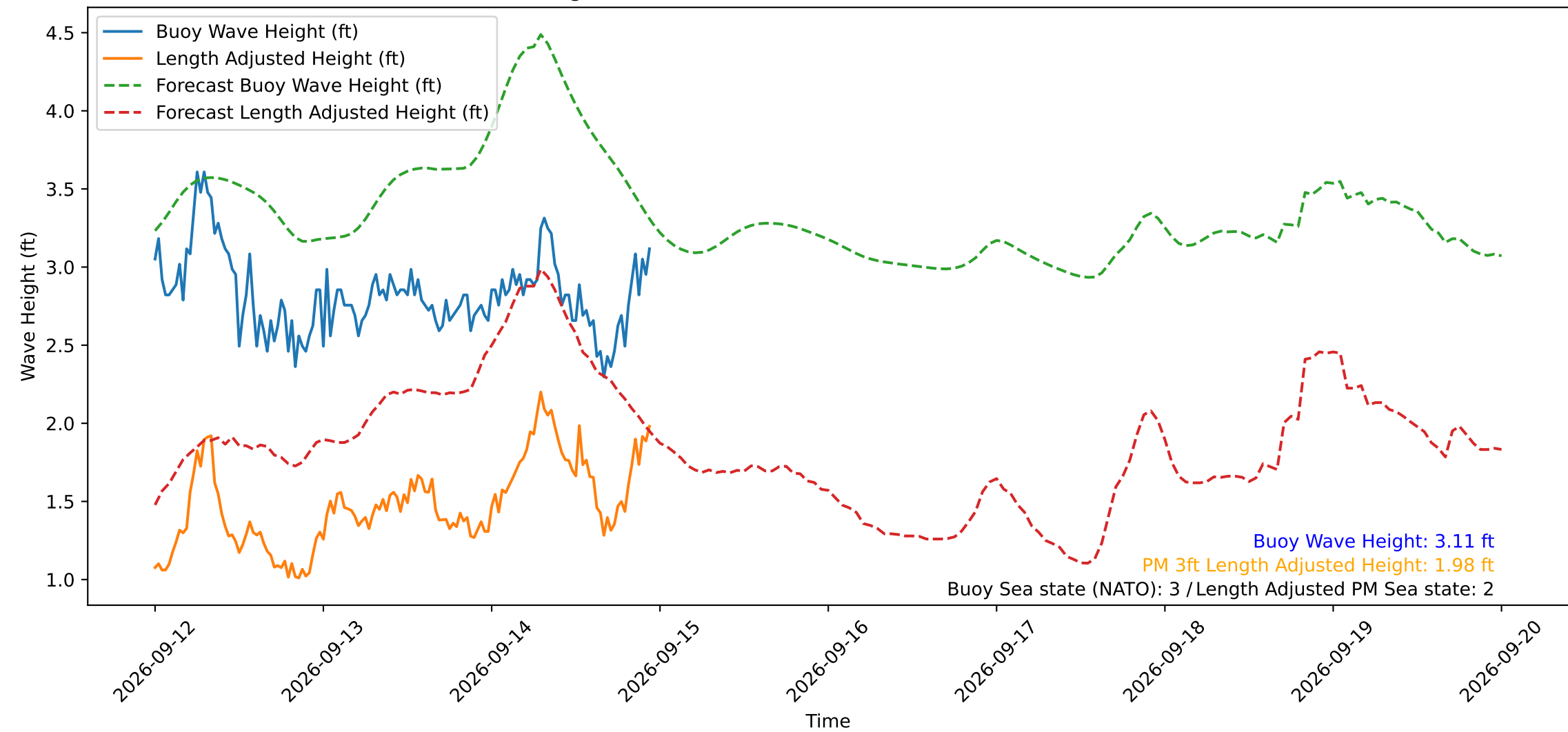
Wave Heights over Time for Green Beach at 2026-09-14 23:31:11
