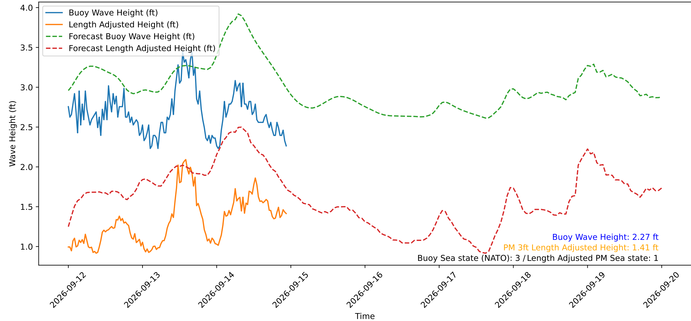
Wave Heights over Time for Red Beach at 2026-09-14 23:30:49
