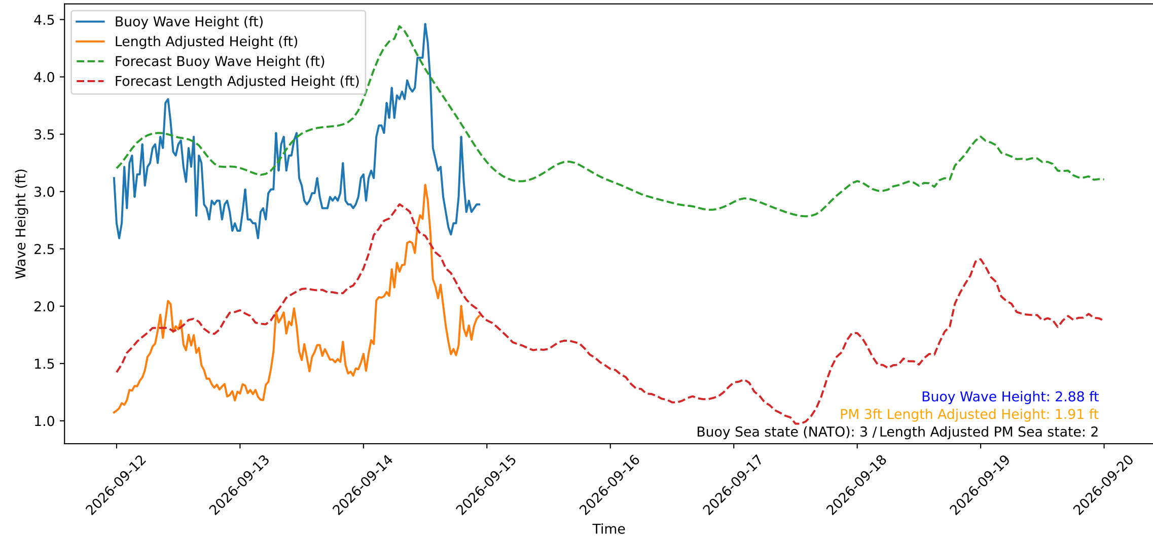
Wave Heights over Time for Oceanside Harbor at 2026-09-14 23:30:29
