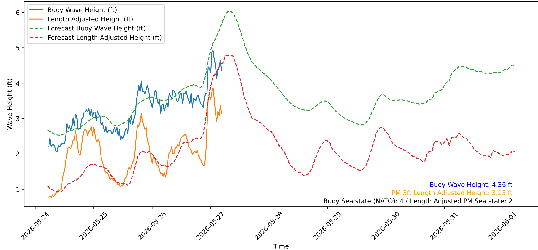
Wave Heights over Time for Green Beach at 2026-05-27 05:21:10
