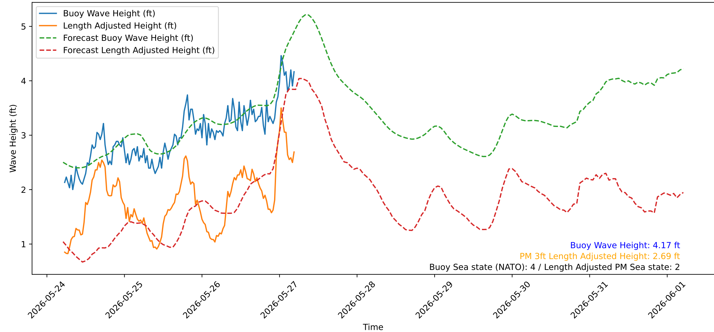
Wave Heights over Time for Red Beach at 2026-05-27 05:20:47
