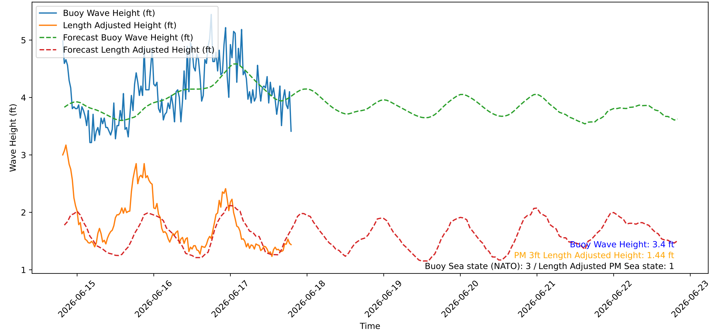
Wave Heights over Time for Oceanside Harbor at 2026-06-17 19:30:27
