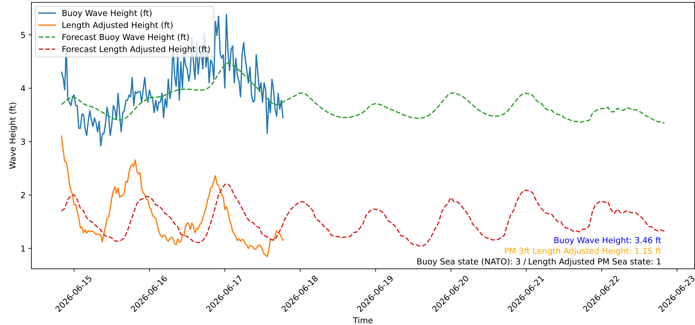
Wave Heights over Time for Red Beach at 2026-06-17 19:30:47
