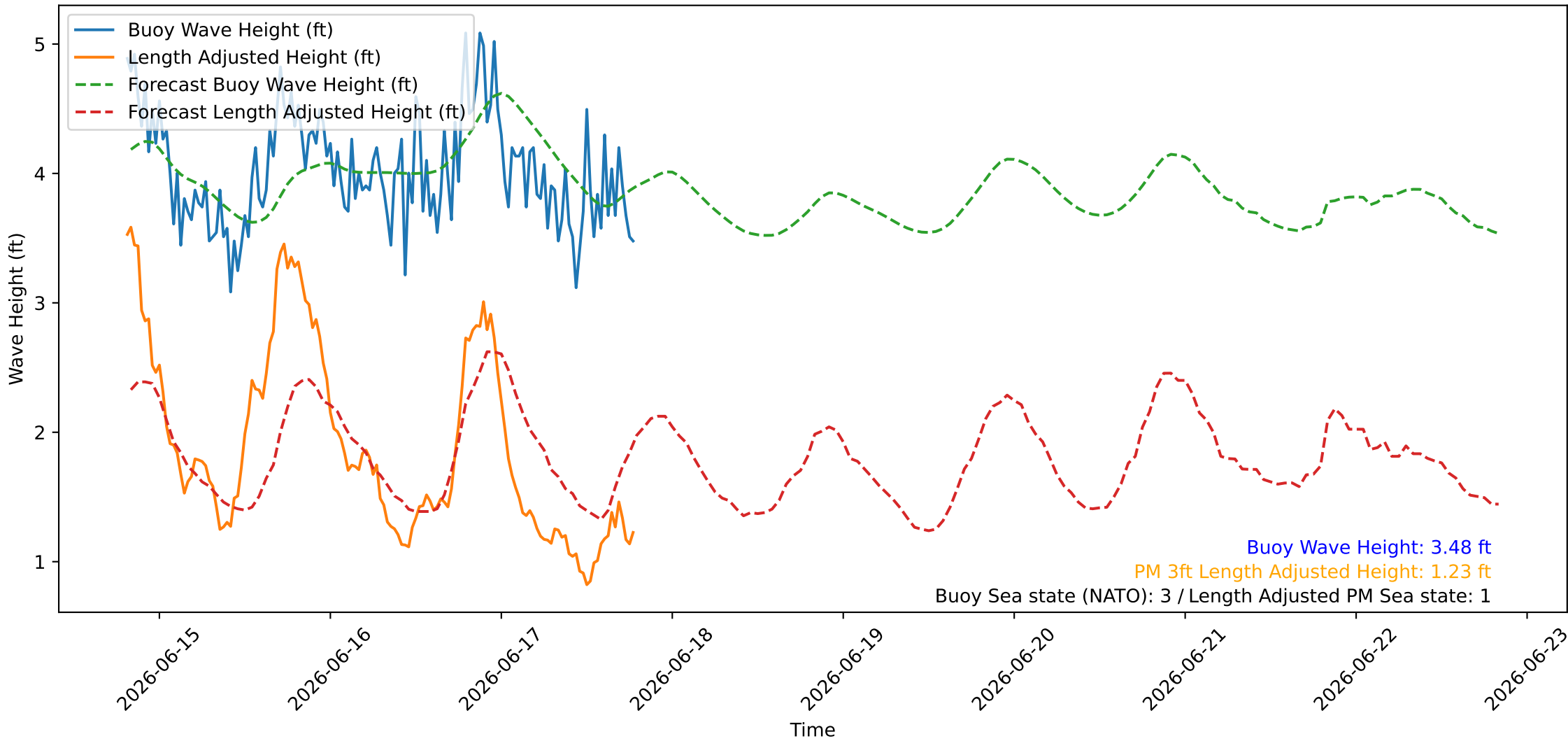
Wave Heights over Time for Green Beach at 2026-06-17 19:31:09
