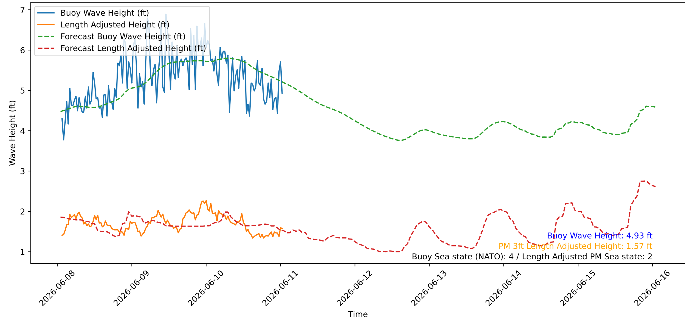
Wave Heights over Time for Green Beach at 2026-06-11 01:21:12
