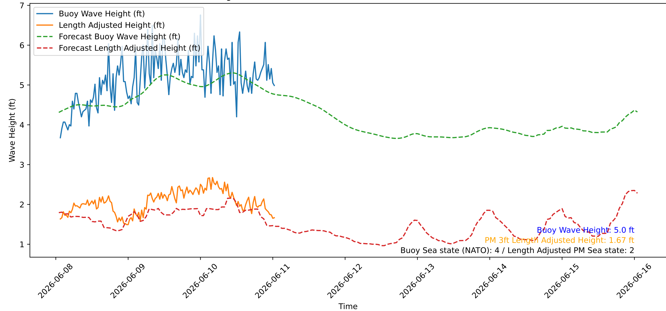
Wave Heights over Time for Oceanside Harbor at 2026-06-11 01:20:27
