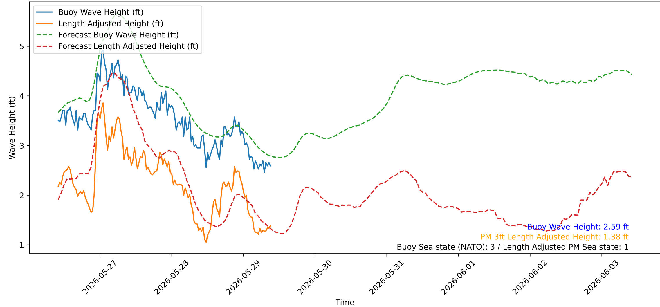
Wave Heights over Time for Green Beach at 2026-05-29 09:51:05
