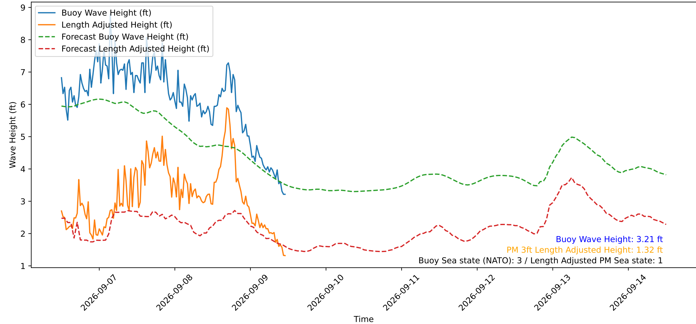
Wave Heights over Time for Green Beach at 2026-09-09 11:41:11
