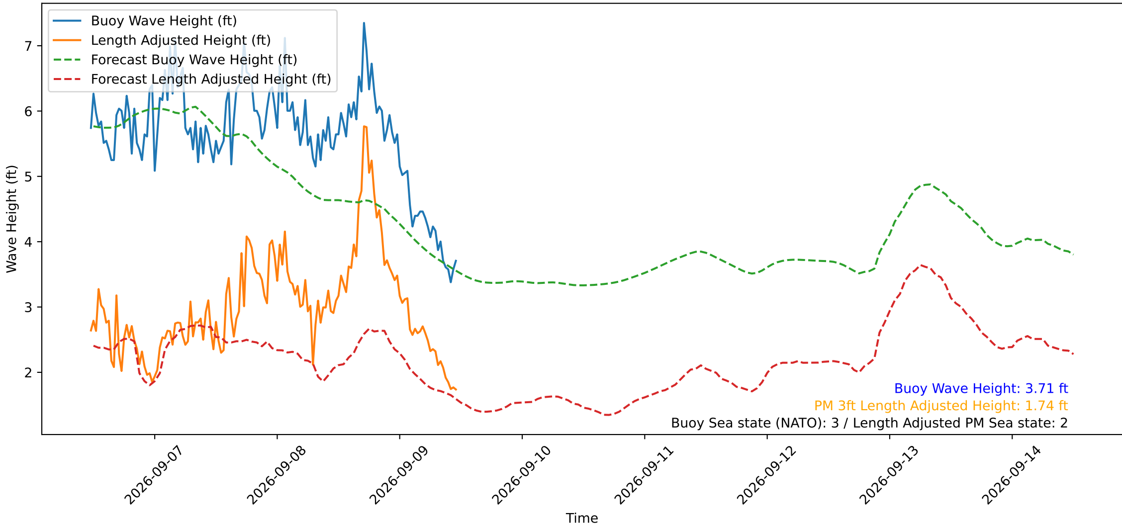
Wave Heights over Time for Oceanside Harbor at 2026-09-09 11:40:29
