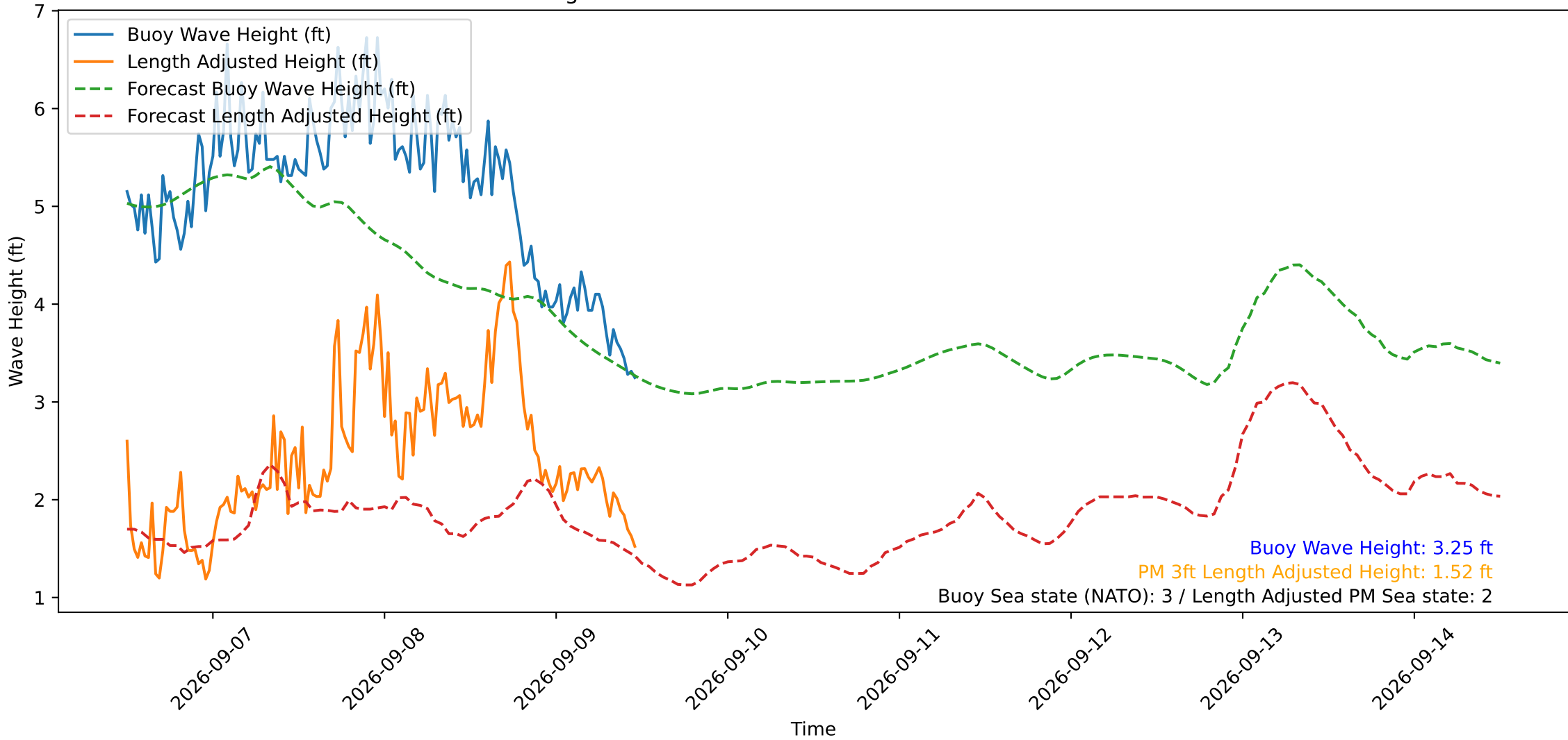
Wave Heights over Time for Red Beach at 2026-09-09 11:40:49
