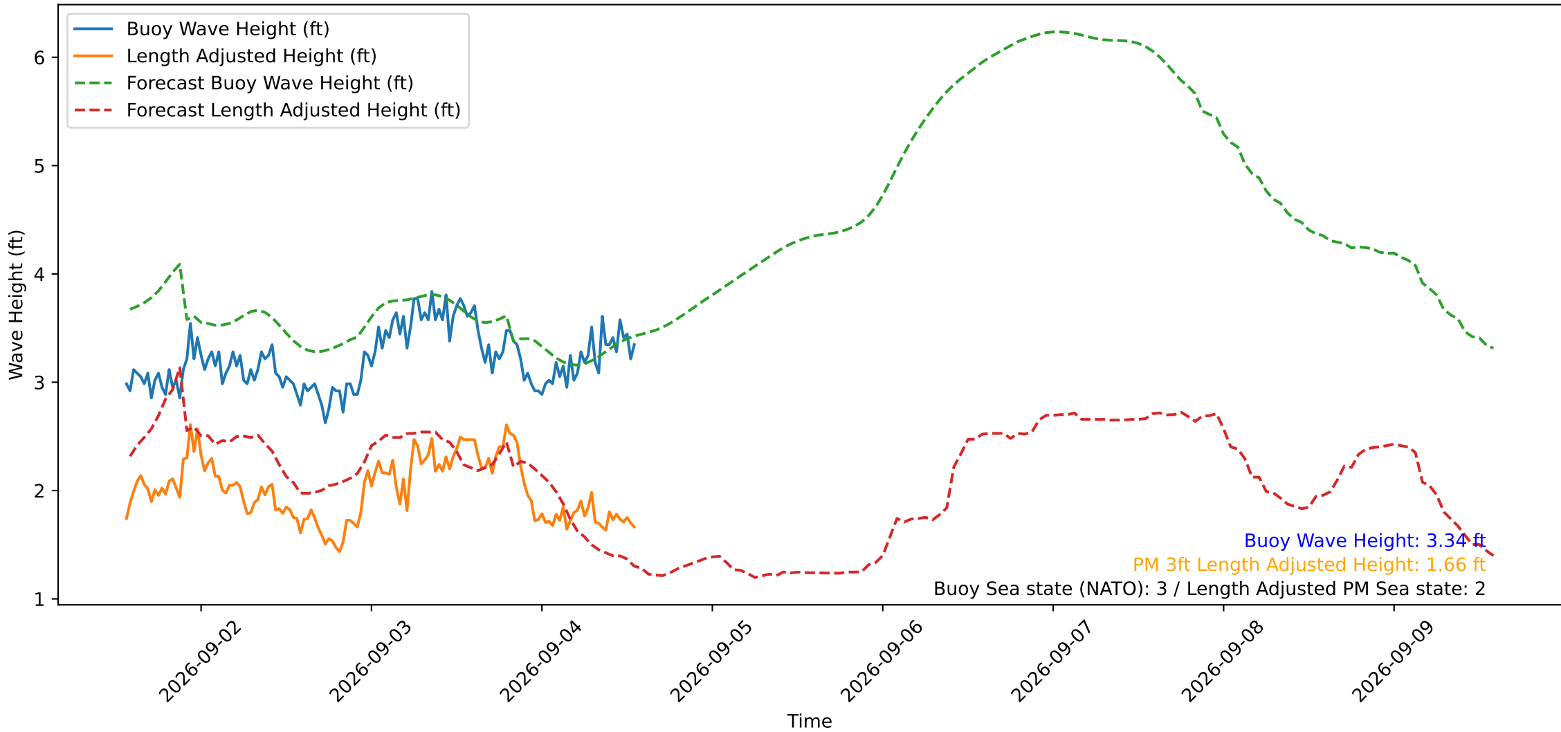
Wave Heights over Time for Oceanside Harbor at 2026-09-04 13:30:30
