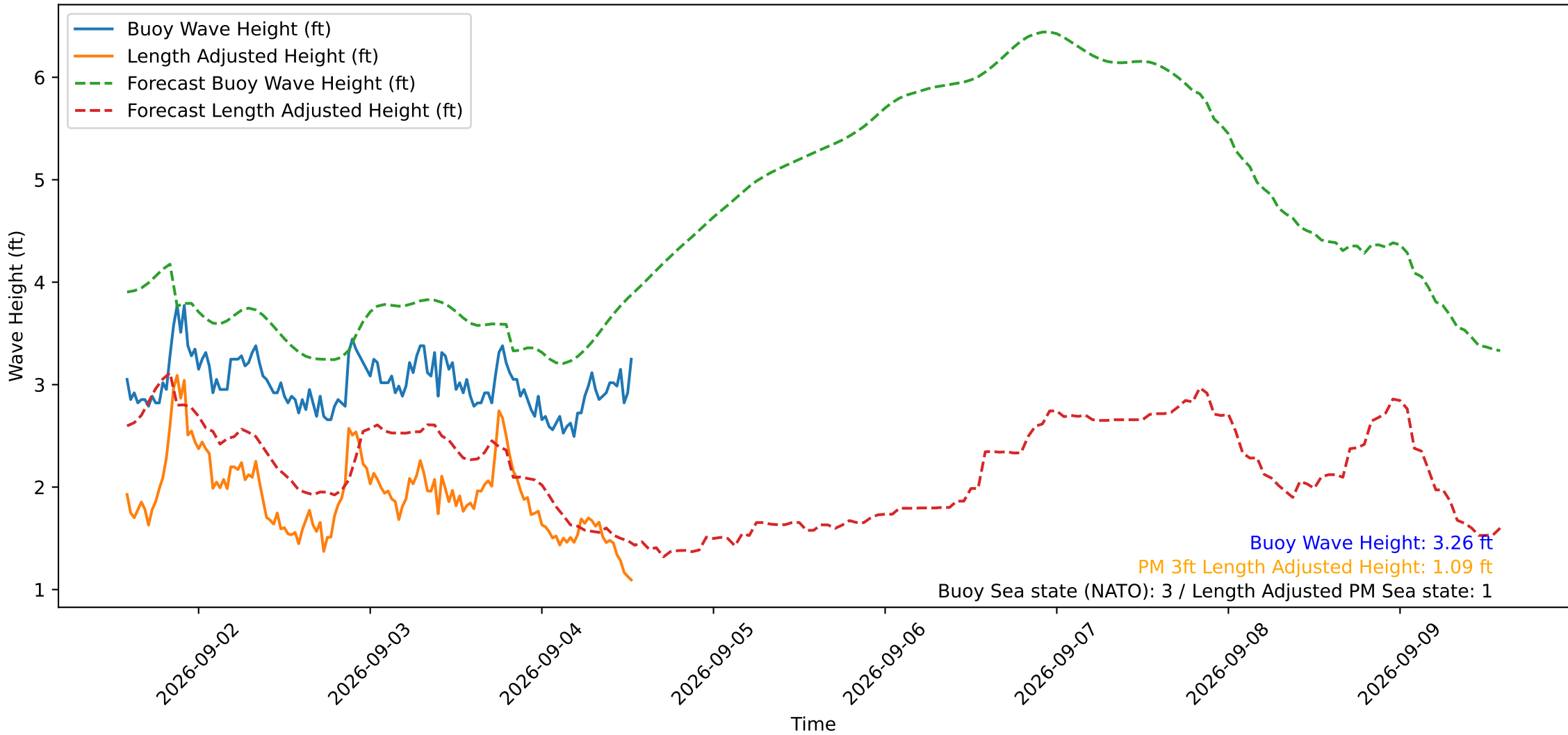
Wave Heights over Time for Green Beach at 2026-09-04 13:31:12
