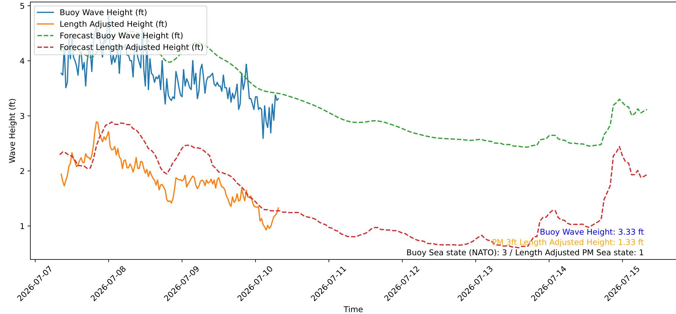
Wave Heights over Time for Red Beach at 2026-07-10 08:10:46
