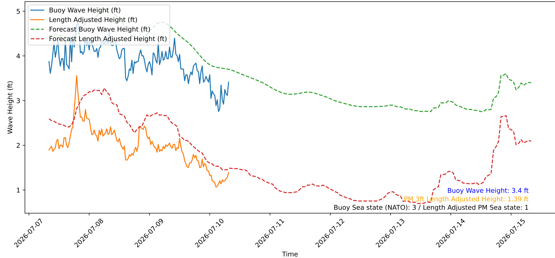
Wave Heights over Time for Green Beach at 2026-07-10 08:11:08
