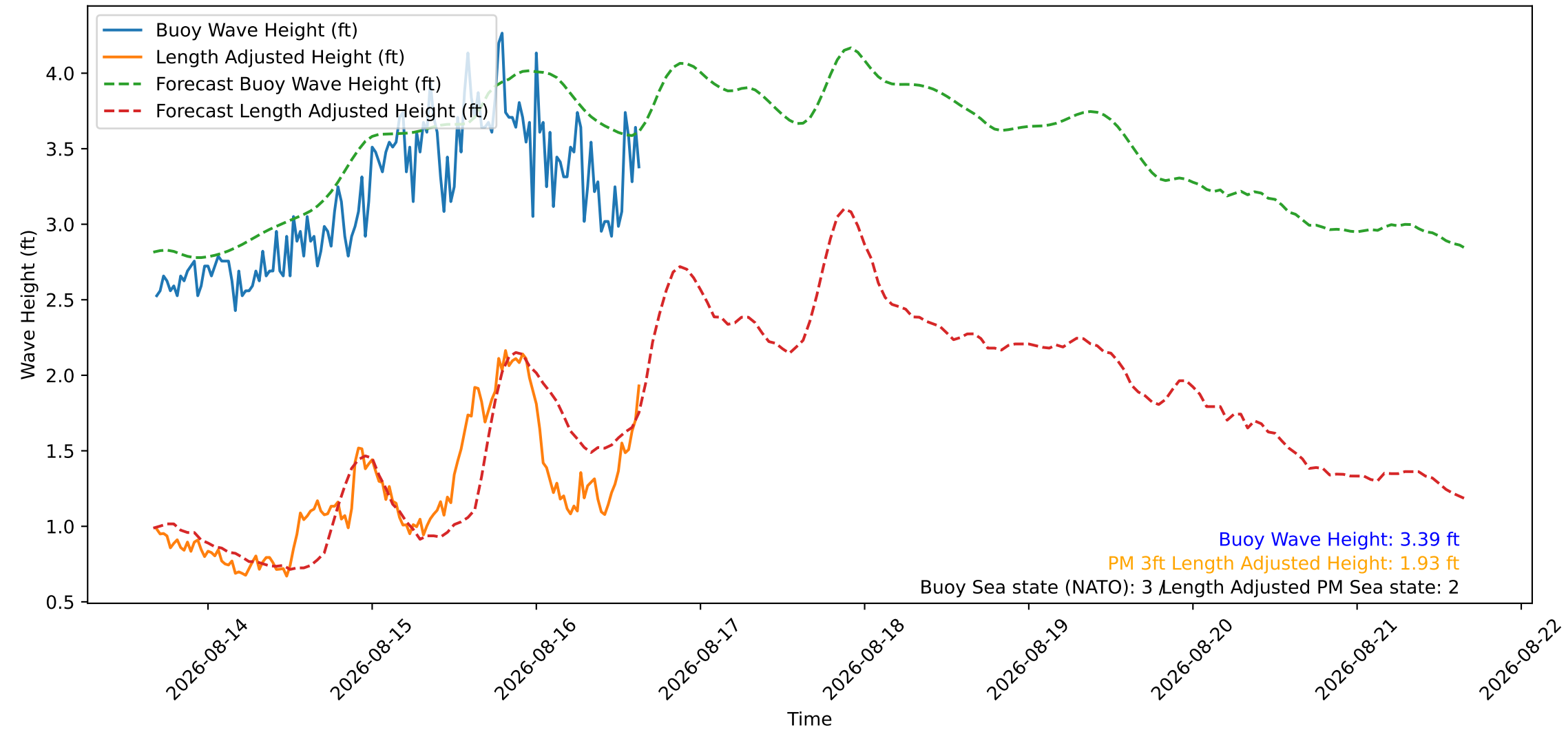
Wave Heights over Time for Green Beach at 2026-08-16 16:01:07
