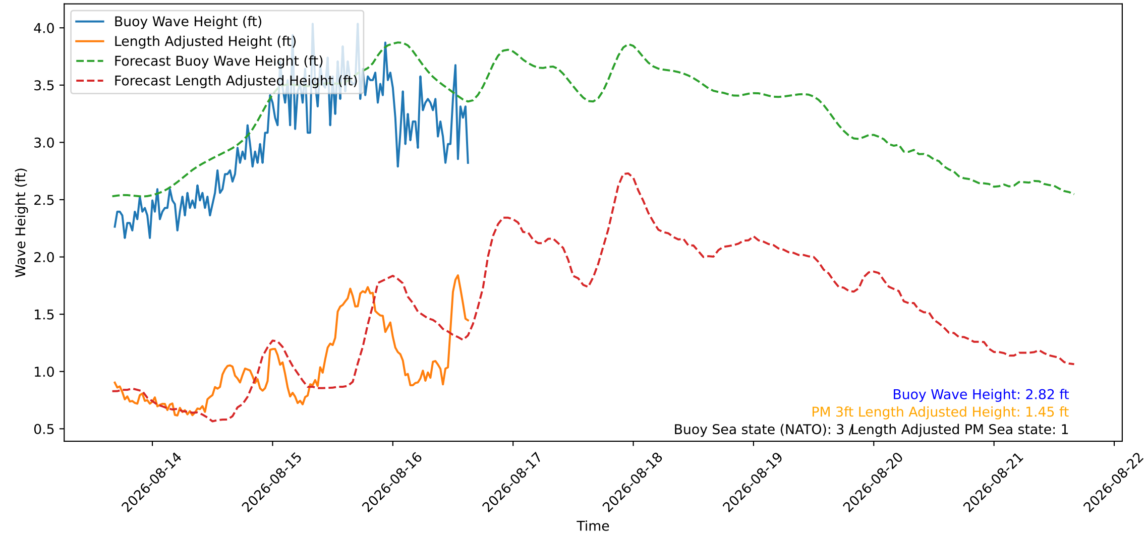
Wave Heights over Time for Red Beach at 2026-08-16 16:00:45
