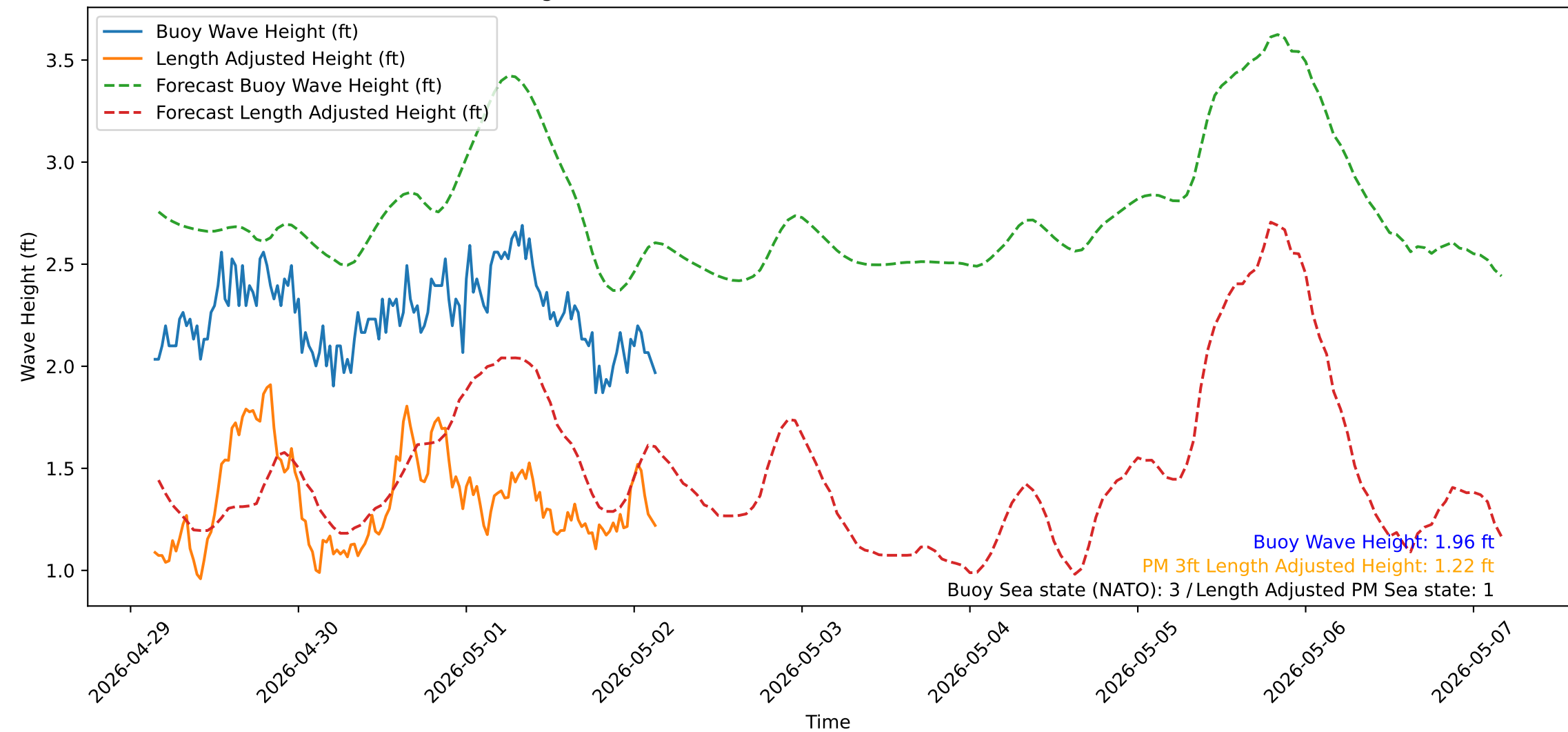
Wave Heights over Time for Oceanside Harbor at 2026-05-02 03:30:31
