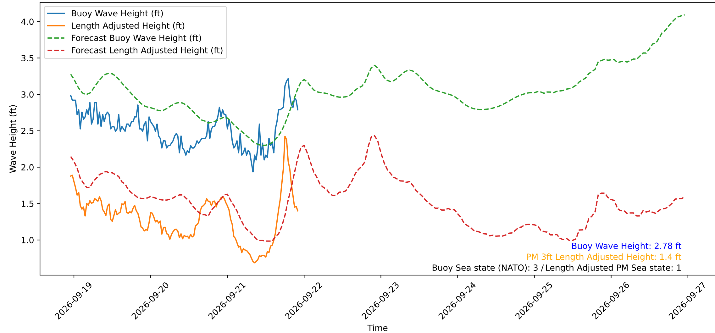
Wave Heights over Time for Green Beach at 2026-09-21 22:51:15
