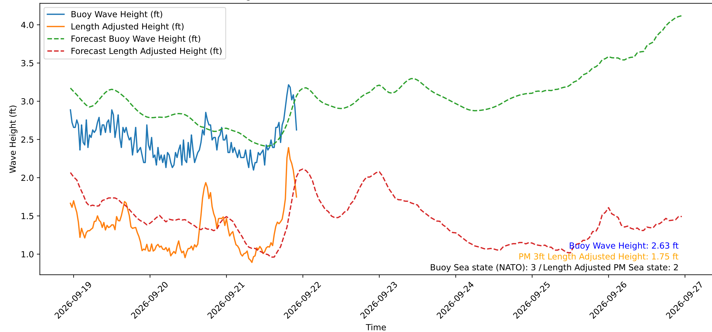
Wave Heights over Time for Oceanside Harbor at 2026-09-21 22:50:29
