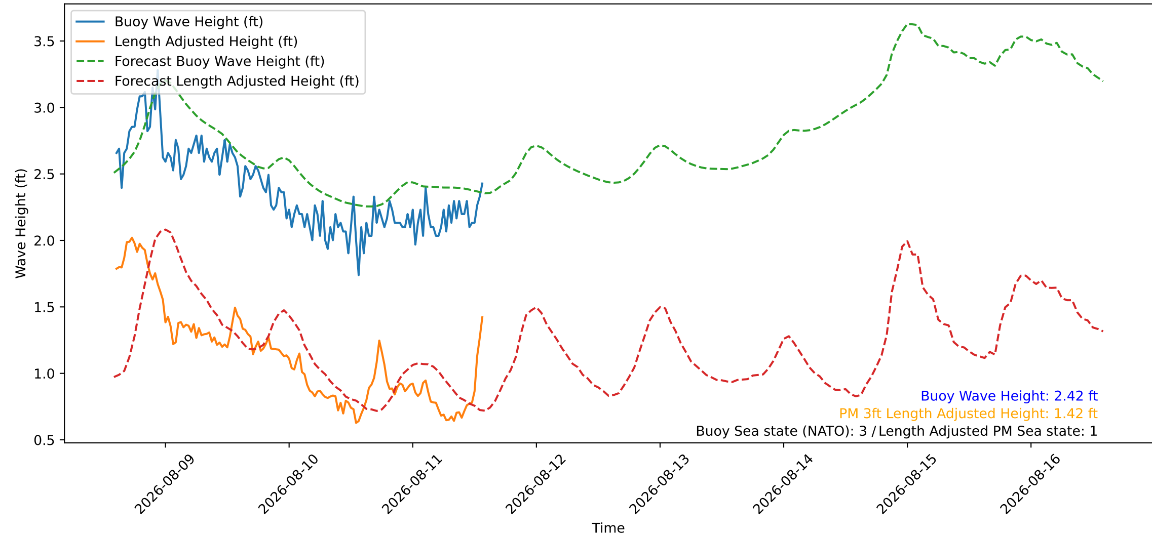
Wave Heights over Time for Red Beach at 2026-08-11 14:20:47
