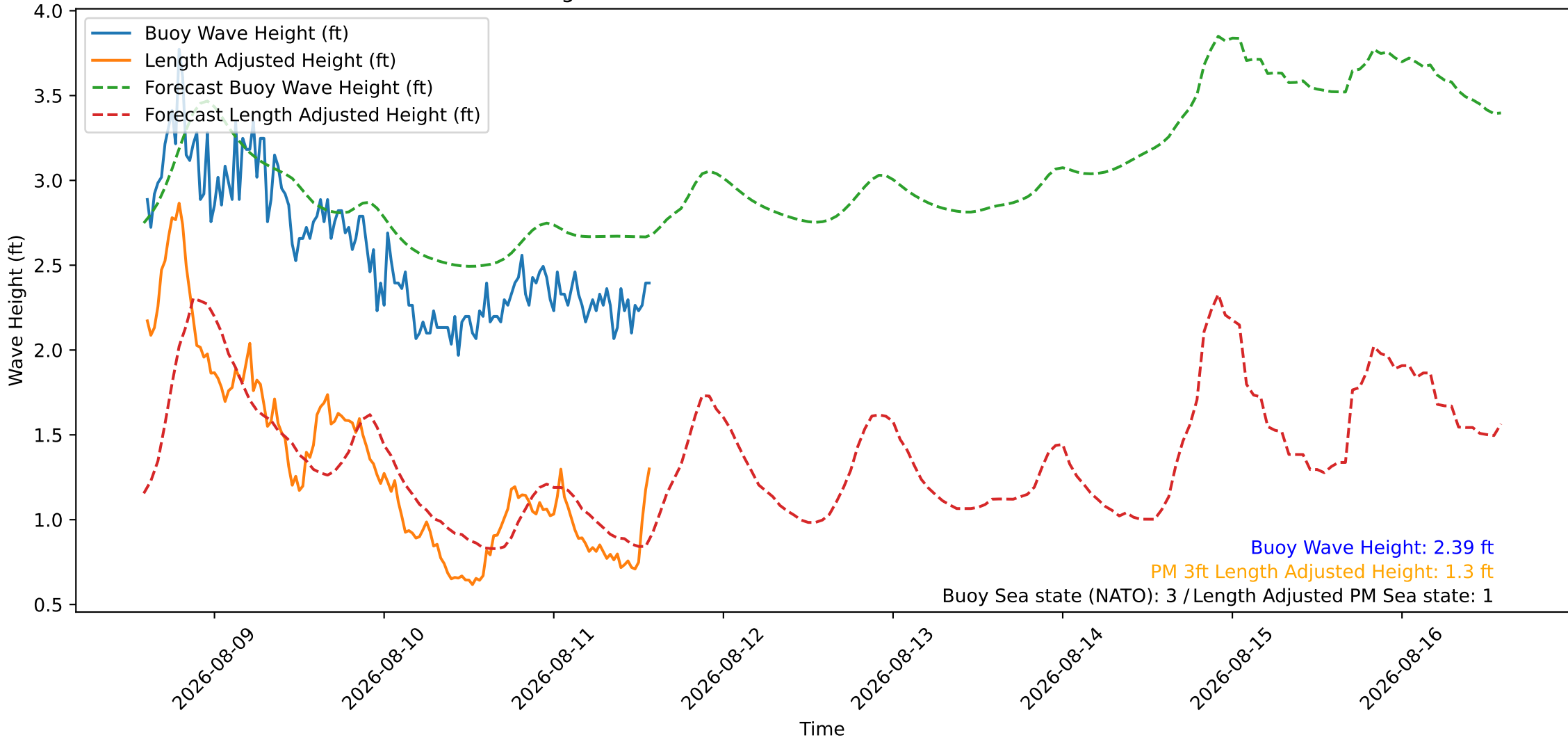
Wave Heights over Time for Green Beach at 2026-08-11 14:21:10
