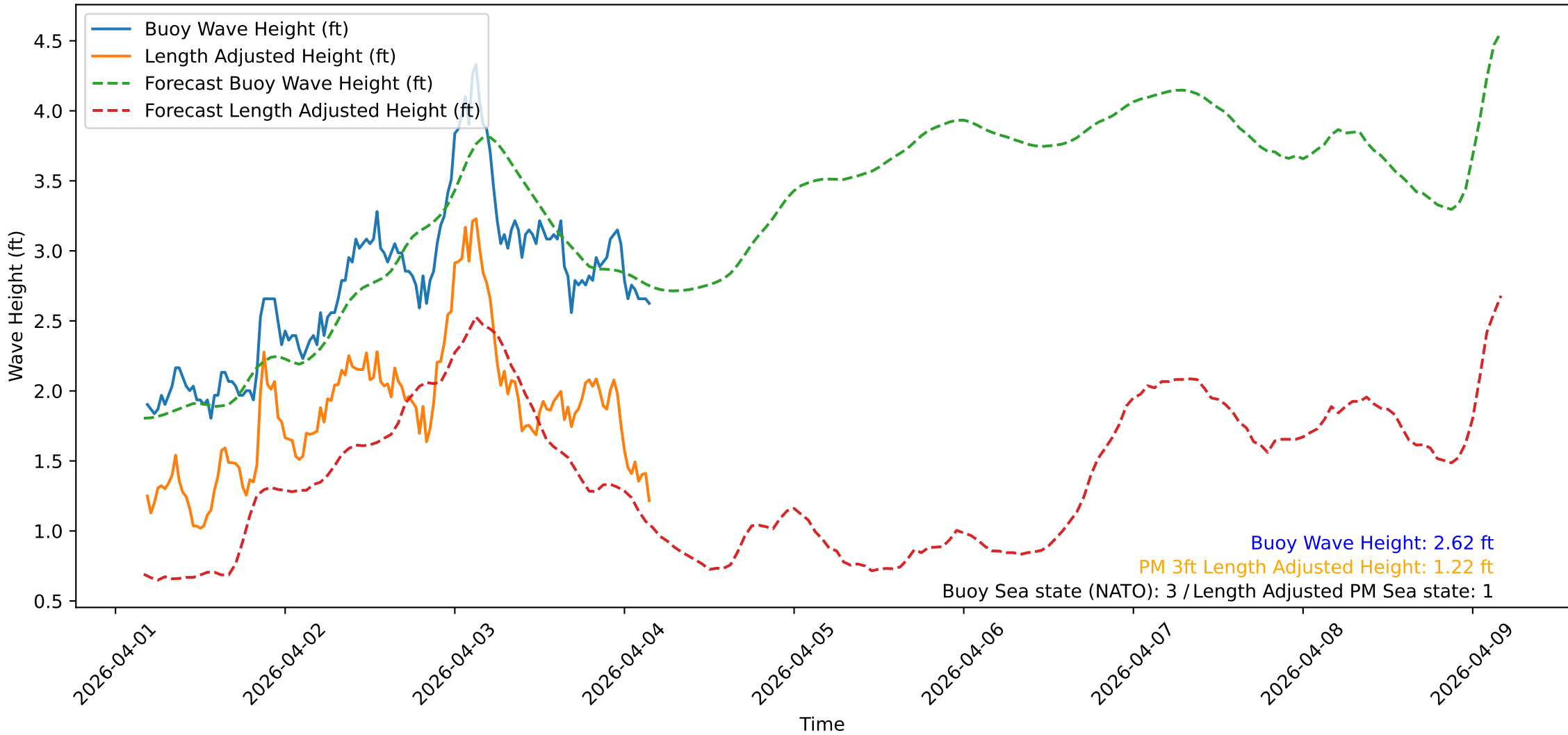
Wave Heights over Time for Green Beach at 2026-04-04 04:21:10
