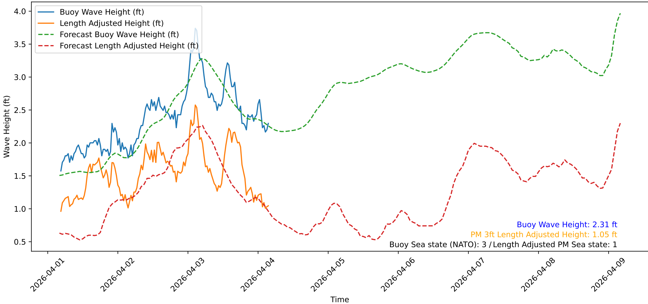
Wave Heights over Time for Red Beach at 2026-04-04 04:20:48
