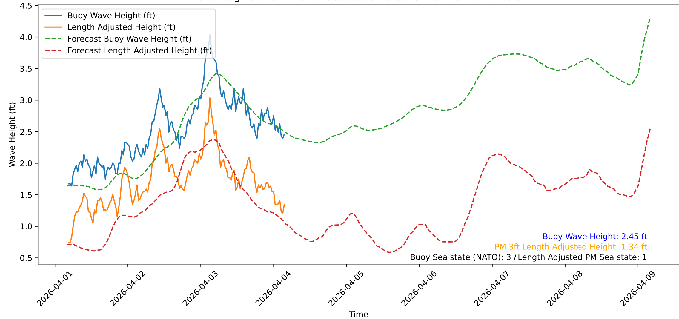
Wave Heights over Time for Oceanside Harbor at 2026-04-04 04:20:31
