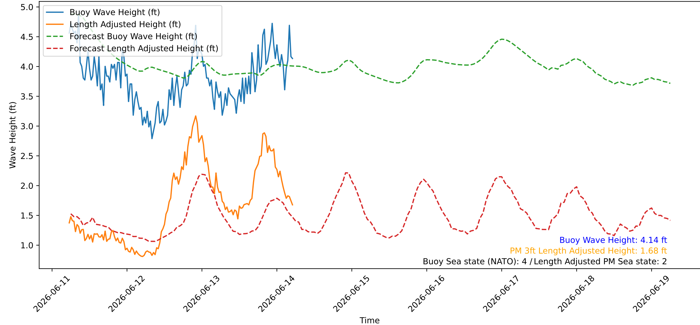
Wave Heights over Time for Oceanside Harbor at 2026-06-14 05:40:27
