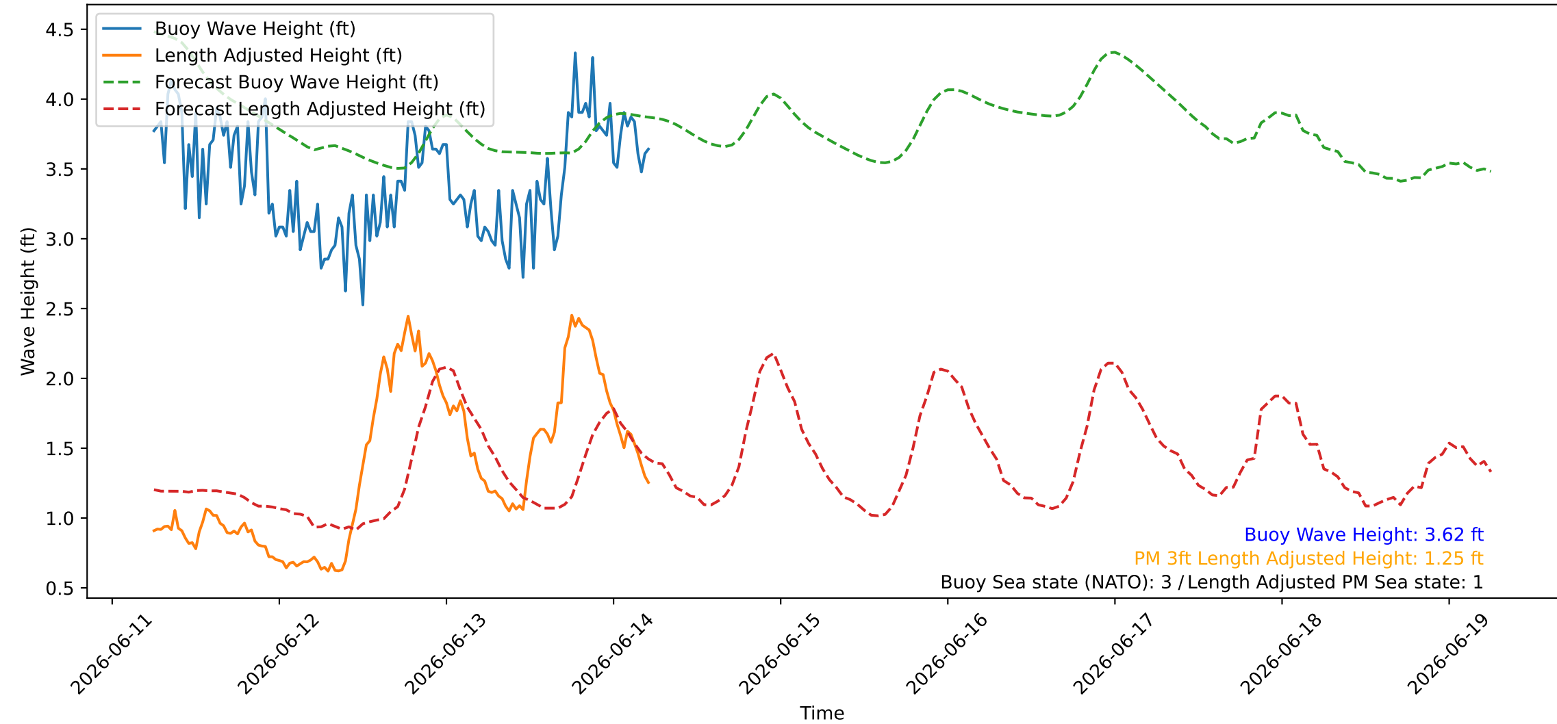
Wave Heights over Time for Red Beach at 2026-06-14 05:40:46
