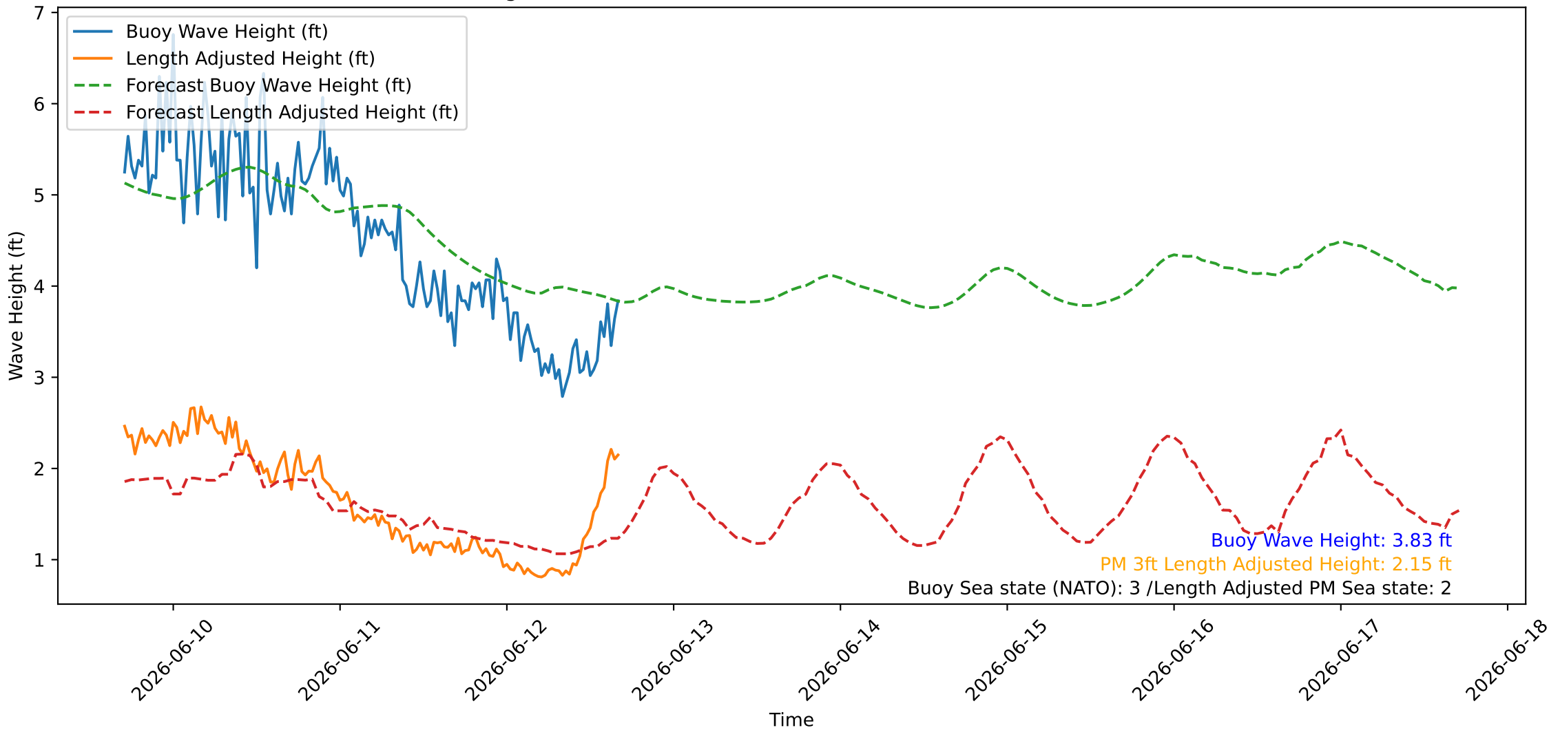
Wave Heights over Time for Oceanside Harbor at 2026-06-12 16:50:26
