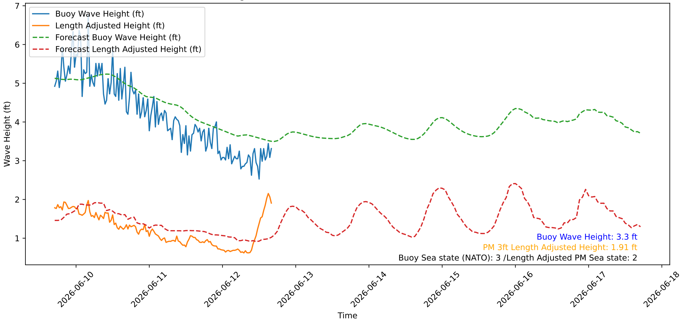
Wave Heights over Time for Red Beach at 2026-06-12 16:50:47
