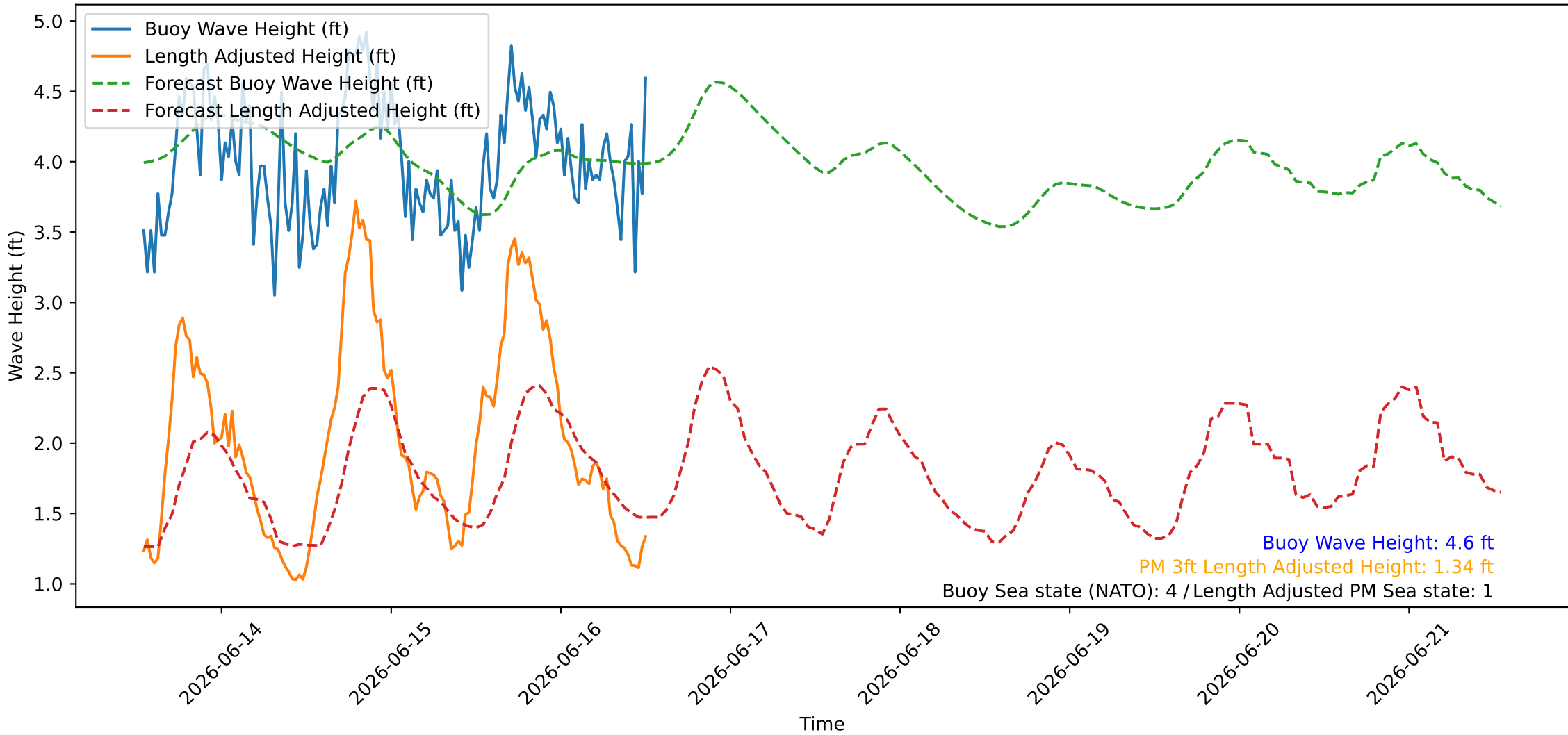
Wave Heights over Time for Green Beach at 2026-06-16 13:01:07
