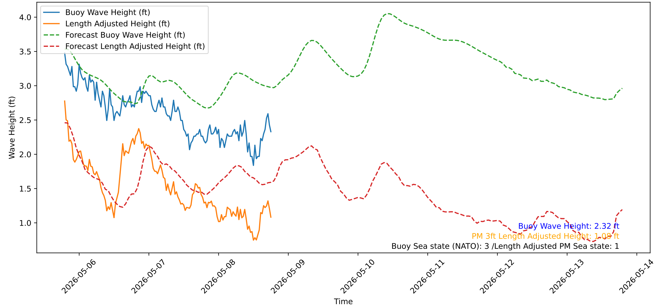
Wave Heights over Time for Green Beach at 2026-05-08 18:51:14
