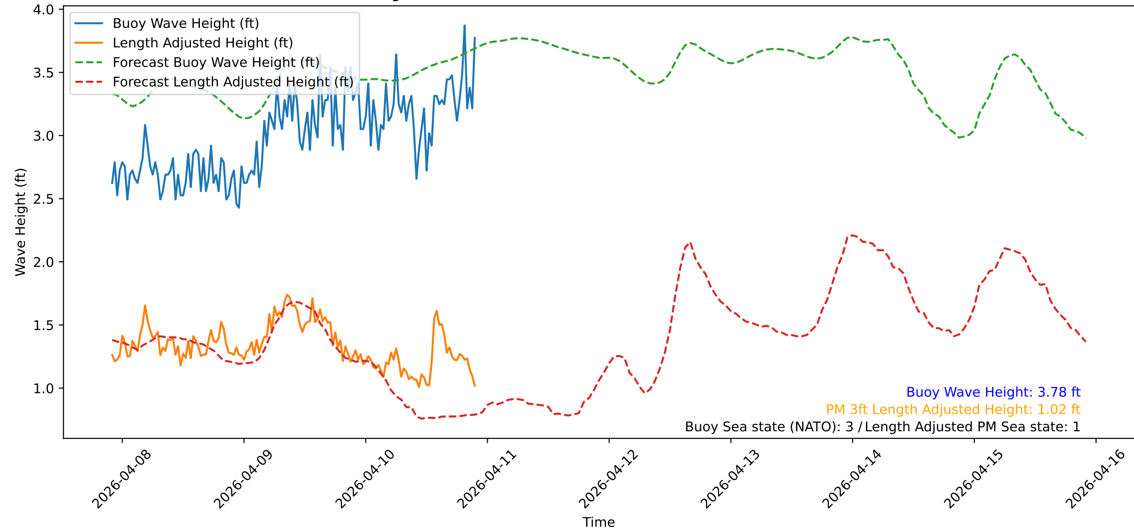
Wave Heights over Time for Oceanside Harbor at 2026-04-10 22:10:32
