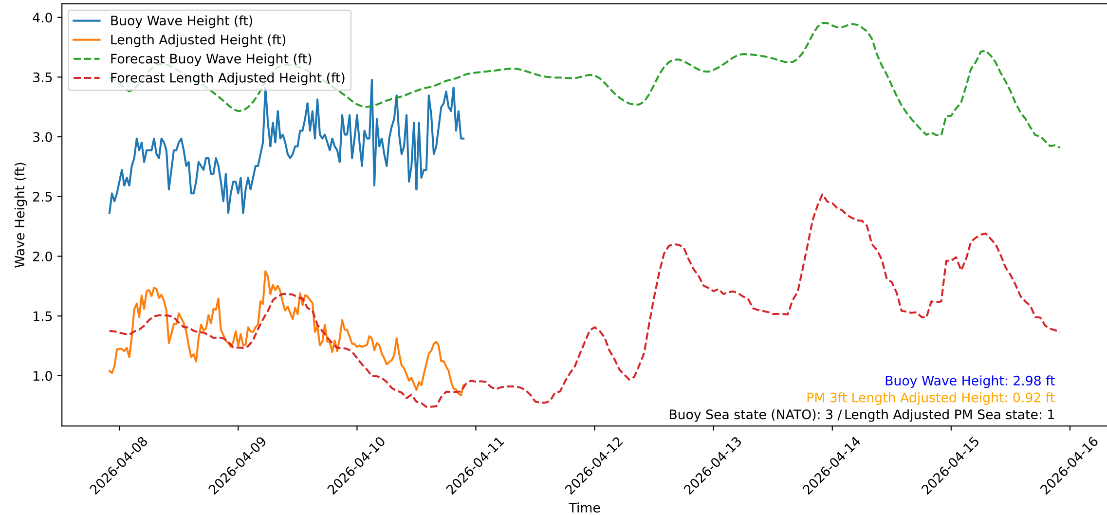
Wave Heights over Time for Green Beach at 2026-04-10 22:11:13
