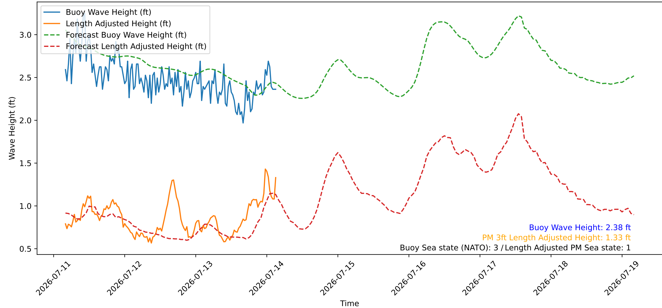
Wave Heights over Time for Red Beach at 2026-07-14 03:50:48
