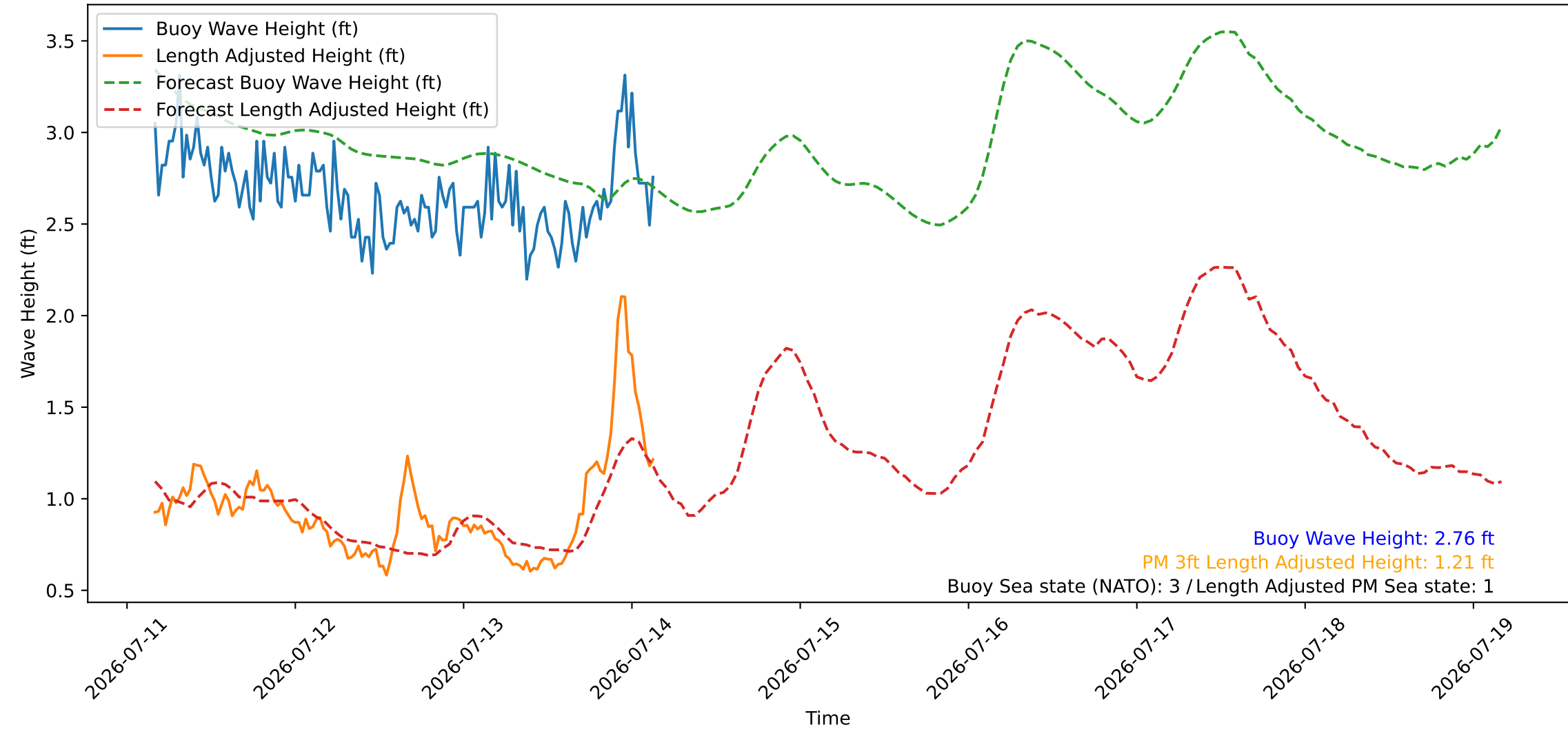
Wave Heights over Time for Green Beach at 2026-07-14 03:51:12
