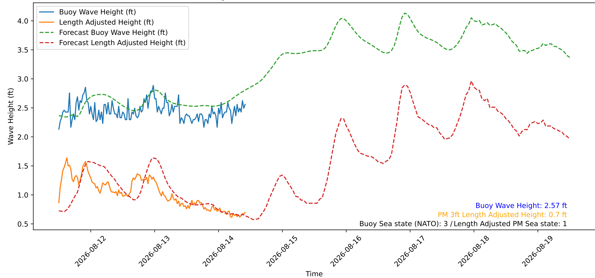
Wave Heights over Time for Red Beach at 2026-08-14 11:30:47
