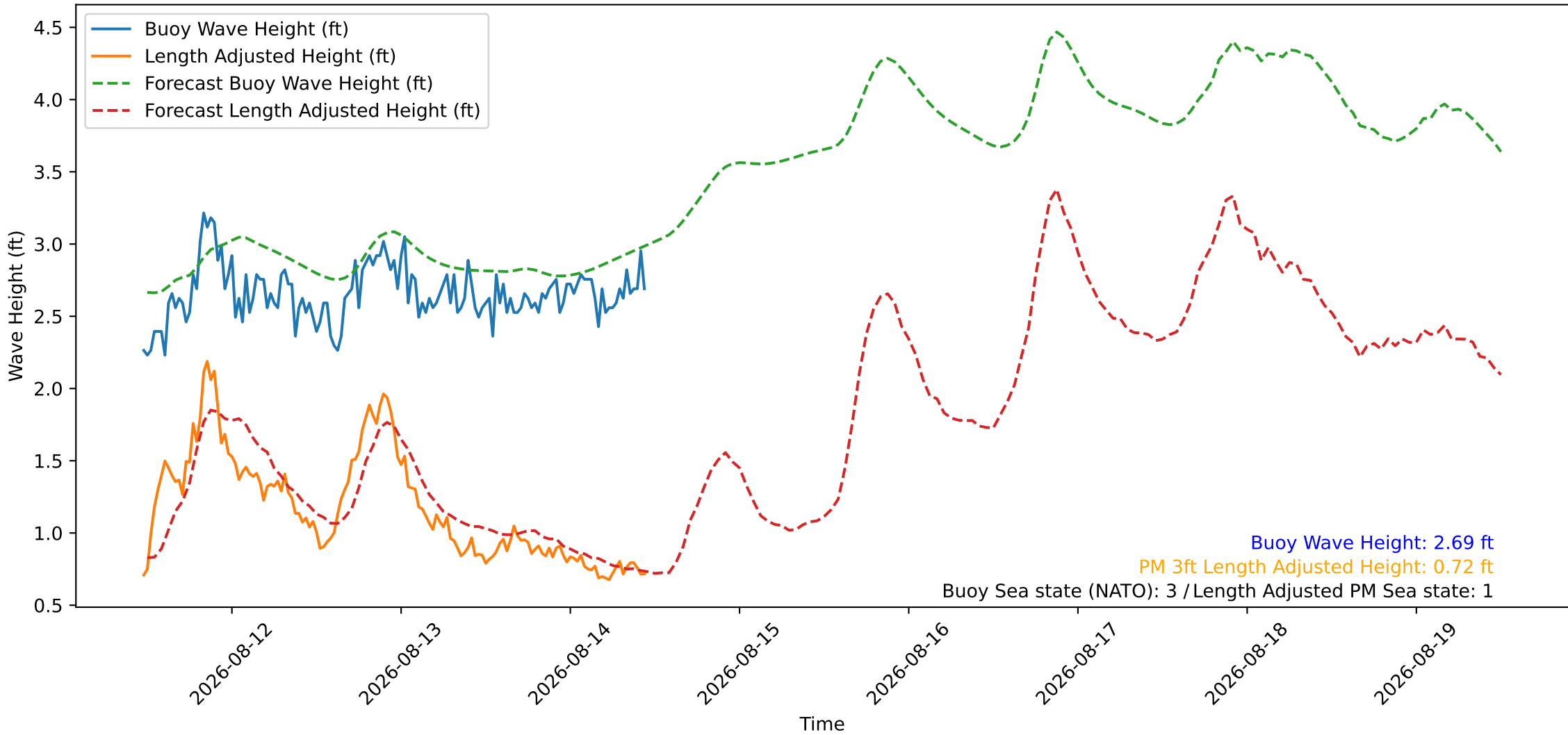
Wave Heights over Time for Green Beach at 2026-08-14 11:31:10
