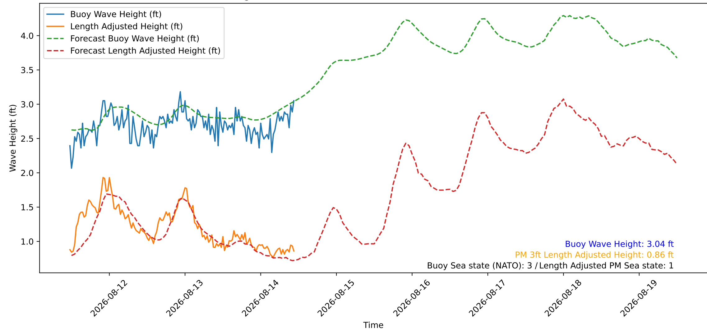
Wave Heights over Time for Oceanside Harbor at 2026-08-14 11:30:27
