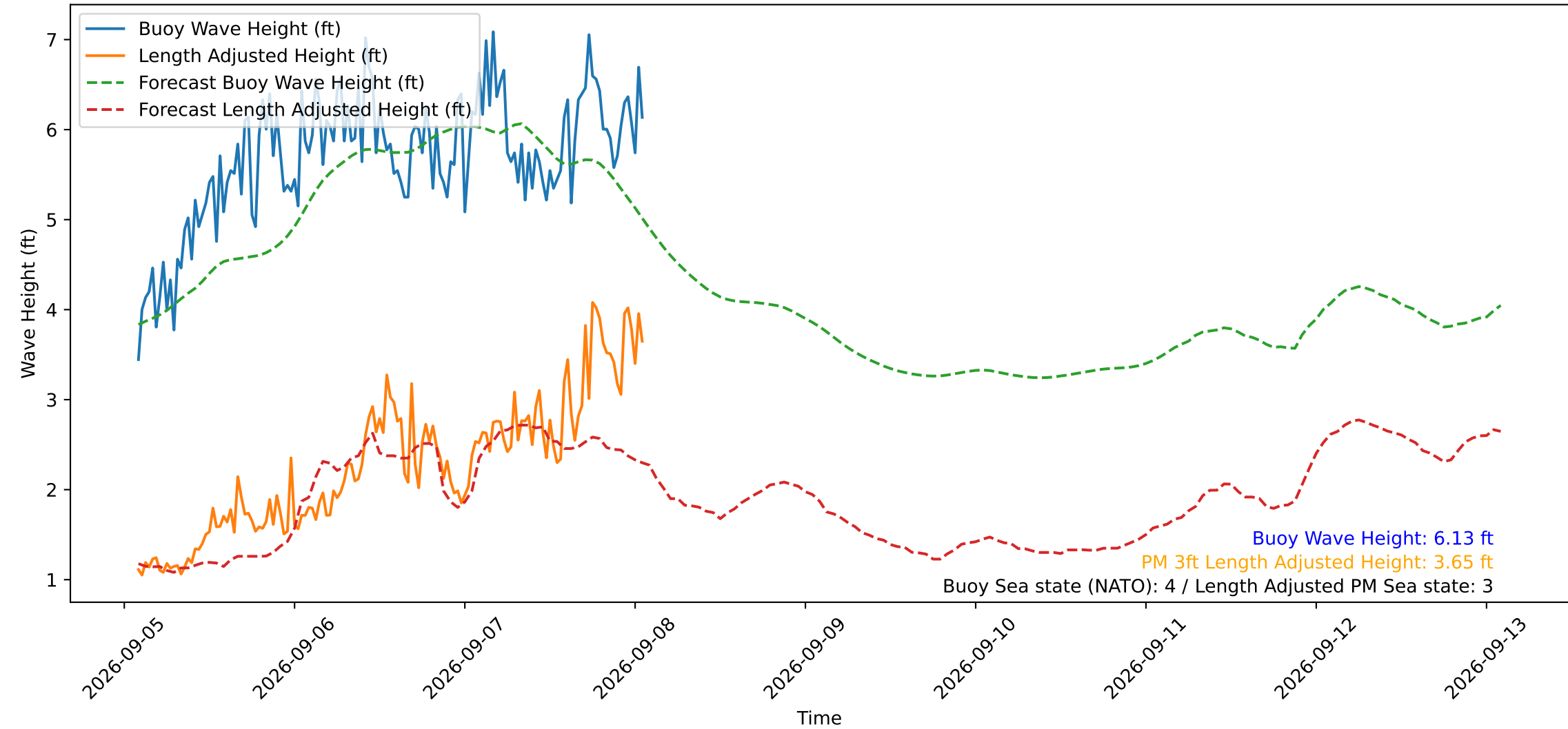
Wave Heights over Time for Oceanside Harbor at 2026-09-08 01:50:29
