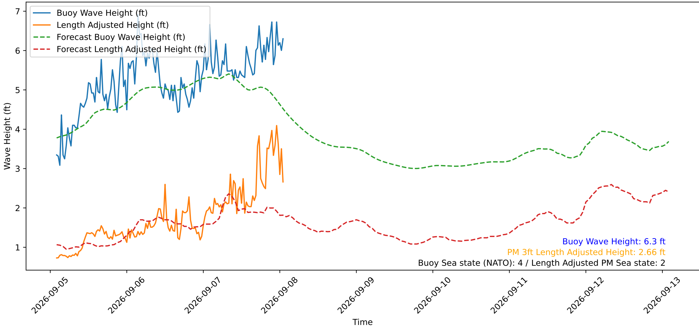
Wave Heights over Time for Red Beach at 2026-09-08 01:50:51
