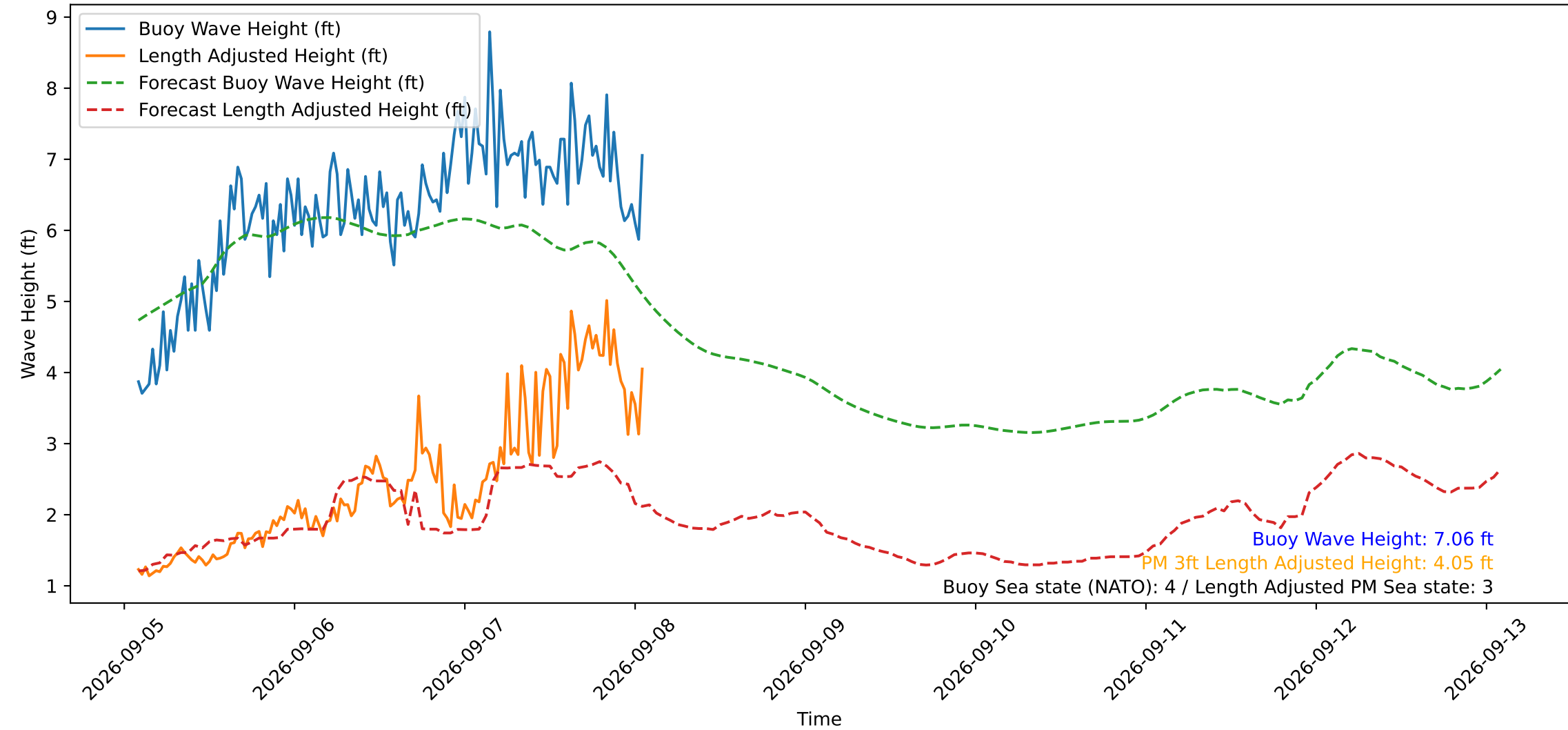
Wave Heights over Time for Green Beach at 2026-09-08 01:51:14
